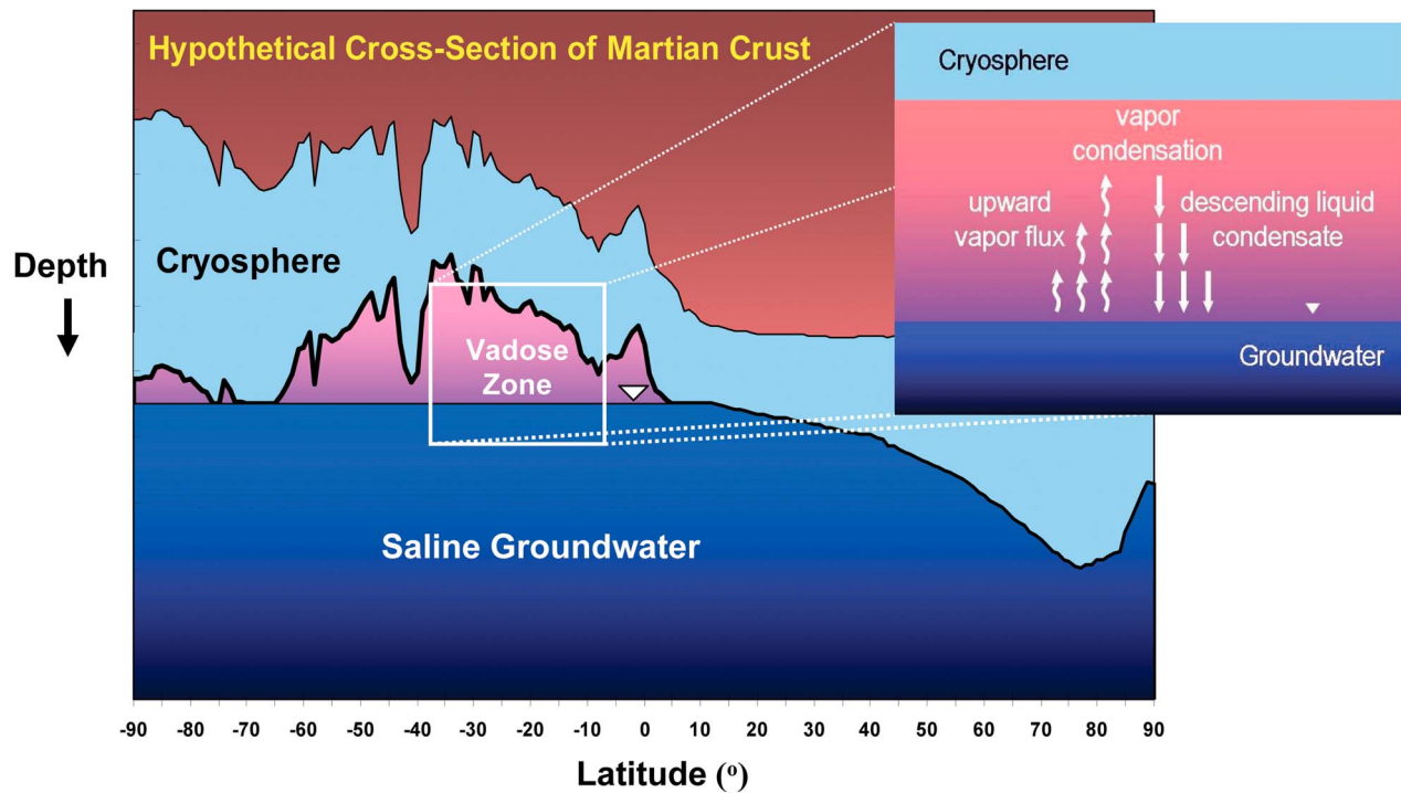
Figure 1. A hypothetical pole-to-pole cross section of the present-day Martian crust (along 203°E longitude), illustrating the potential relationship between surface topography, ground ice, and groundwater. Surface elevations are from the MOLA Mission Experiment Gridded Data Record with a 2° smoothing function [Smith et al. , 2003]. At those locations where the base of the cryosphere is in contact with the water table, the presence of dissolved salts may reduce the thickness of frozen ground by depressing the freezing point of the groundwater to a value as low as the 203 K eutectic temperature of a saturated \text{Mg}(\text{ClO}_4)_2 brine. Conversely, where the cryosphere and groundwater are not in direct contact, the leaching of soluble salts by low-temperature hydrothermal convection (see inset and discussion from Clifford [1993]) may result in basal melting temperatures closer to ~273 K. Note that local variations in the thermal, diffusive, and hydraulic properties of the crust are likely to result in significant differences in the distribution of ground ice and groundwater from that depicted here. After Figure 1 of Clifford and Parker [2001].
