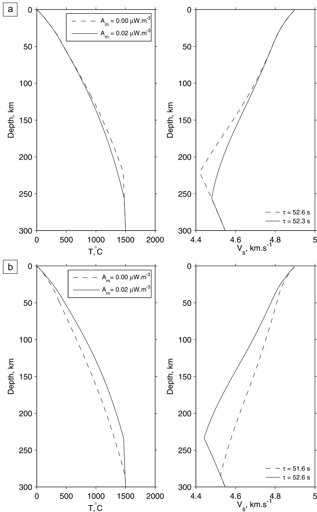
Figure 11. Sensitivity test for thermal models of the lithospheric mantle with different values of heat production for a surface heat flux of 40 mW m -2 . (a) Calculations for a fixed Moho heat flux (equal to 15 mW m -2 ) and hence variable heat flux at the base of the lithosphere. (b) Calculations for a fixed basal heat flux (12 mW m -2 ) and variable Moho heat flux.
