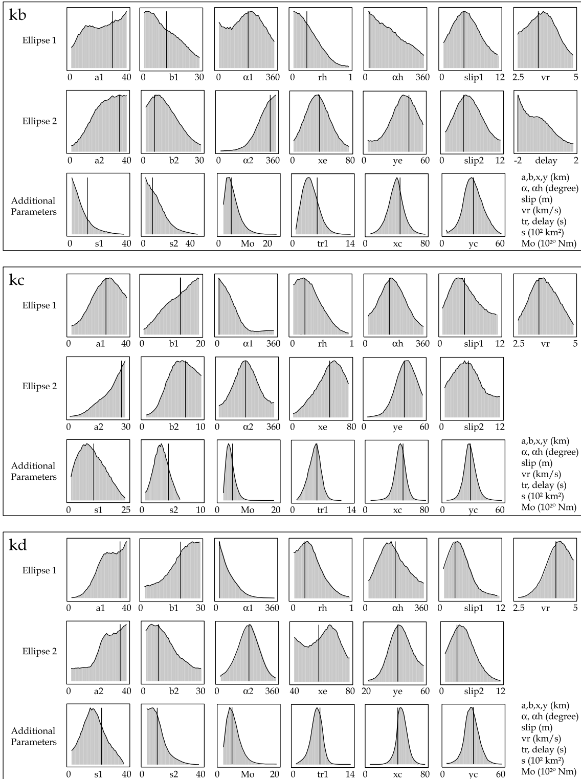
Figure 7. Results of the resampling algorithm for the three kinematic models with two patches. For each models k_b , k_c and k_d , each panel represents the marginal PDF for the inverted parameters and for some additional deduced parameters. The first row represents the PDF of the inverted parameters of the first slip patch, and the rupture velocity. The second row represents the PDF of the inverted parameters of the second slip patch. The third row represents the PDF of the following additional parameters computed during the resampling: the surfaces of the ellipses ( s_1 and s_2 ), the total seismic moment, the approximated rupture time on the first ellipse ( t_{r1} ) and the coordinates of the rupture centroid on the fault ( x_c and y_c ). Each x -axis is over the complete range of the parameters space. The vertical lines show the results of each model. Each curve is scaled to the same maximum height, not the same area.
