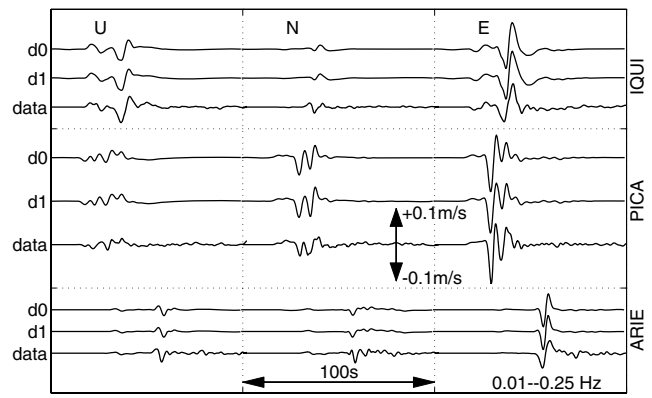
Figure 10. Comparison of the velocity waveforms of the dynamic models d_0 and d_1 with the strong motion data. Waveforms are dominated by S wave but P wave and intermediate field are visible on PICA and IQUI. All waveforms are filtered in the frequency band 0.01–0.25 Hz. A general good agreement is observed. The complexity of the waveforms is similar. Phases of arrivals and pulses are correct. Although local differences of amplitude and pulse durations may be observed (especially on the north components), amplitudes are globally satisfactory for such models built by trial and error. Models d_0 and d_1 produce waveforms with insignificant differences.
