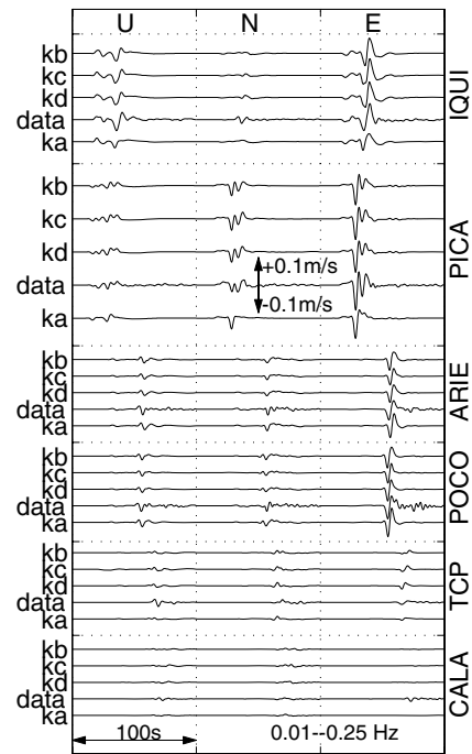
Figure 5. Data and synthetic waveforms (velocities) for single patch model k_a and for double patch models k_b , k_c and k_d . All waveforms are filtered in the frequency band 0.01–0.25 Hz. Single patch model k_a does not reproduce waveforms complexities on IQUI and PICA whereas double patch models fit better the data, and almost equivalently.
