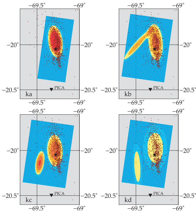
Figure 4. Kinematic inverted models. Slip colour scale ranges from blue (0 m) to red (5 m). The star is the epicentre and red dots are the aftershocks. Model k_a is the single patch model. Model k_b , k_c and k_d are three inverted double patch models, with one main patch attached to the hypocentre and one secondary patch. These three models are obtained with different additional assumptions. For k_b : an additional delay of triggering for the secondary patch, for k_c : a limited range of exploration for the ellipses dimensions to force the finding of a slower rupture velocity and for k_d : a wide range of exploration for the ellipses dimensions. The main characteristics of these models are reported on Table 2
