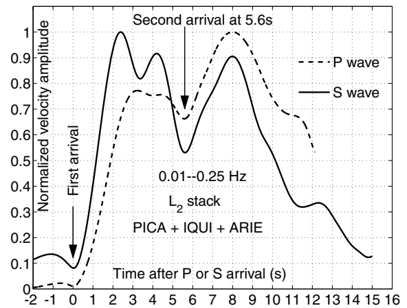
Figure 2. Main features of strong motion records. Dotted and plain curves represent L_2 stacks of the normalized P and S amplitude waveforms at stations PICA, IQUI and ARIE. Before stacking the stations with L_2 norm, each station is normalized by its own L_2 norm computed on the observation duration (12 s for P wave and 15 s for S wave). The resulting curves are dimensionless velocity waveforms. The data are filtered in the frequency band 0.01–0.25 Hz. The signal of the P wave is not represented after 12 s because of the S -wave arrival. On both P and S waves, a clear minimum of amplitude at 5.6 s separates two episodes of strong radiation. At 11 s, most of the main rupture process is done (on the S wave, the slower decreasing signal after 11 s can be partly attributed to structure and free surface effects).
