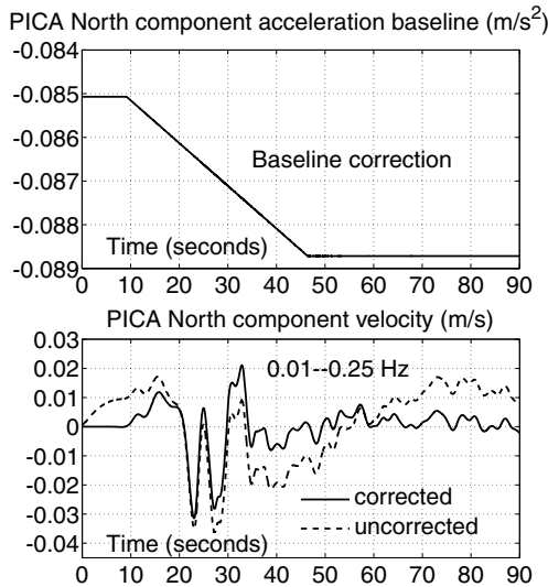
Figure 3. Top panel: piecewise linear baseline corrections performed on the PICA north acceleration component. Bottom panel: 0.01–0.25 Hz filtered PICA north velocity component obtained with and without the application of the baseline correction. The filter is designed as a 0.01 Hz fourth-order highpass Butterworth combined to a 0.25 Hz second-order twice-passed lowpass Butterworth. The difference between the corrected and uncorrected signals is large in this frequency range.
