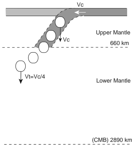
Figure 5. Cartoon representing the construction of a density heterogeneity model for the Earth based on subduction history from Lithgow-Bertelloni & Richards (1998).
