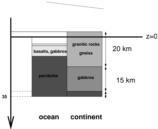
Figure 11. Simple model of continental and oceanic crust.
