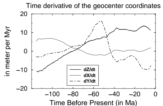
Figure 10. Time-derivative of the coordinates of the geocentre, in metre per million years (or in millimetre per century), since 120 Ma.
