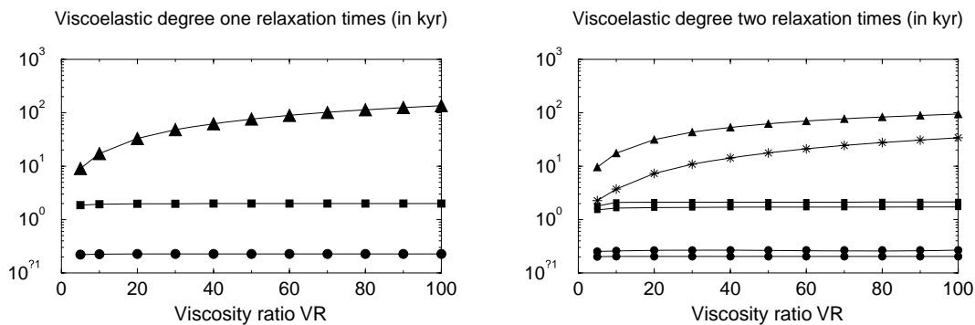
Figure 1. Viscoelastic relaxation times for the degree n = 1 (left-hand panel) and the degree n = 2 (right-hand panel) in Kyr as a function of a viscosity ratio VR ranging from 5 up to 100. Circle symbol: transition times associated with the viscosity jump between lower and upper mantle. Square symbol: transition times associated with the viscosity jump between upper mantle and lithosphere. Triangle up symbol: time associated with C mode induced by density jump at the CMB. Star: time associated with M_o mode induced by density jump at the surface.
