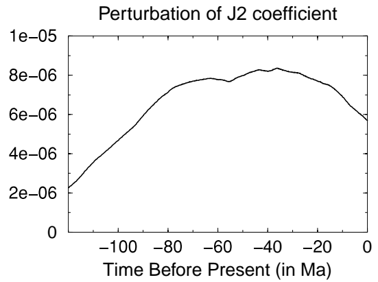
Figure 8. Temporal evolution of the degree 2 geopotential coefficient J_2 induced by our time-dependent internal loads model, since 120 Ma.
