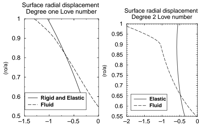
Figure 2. Kernels for the surface radial displacement, for the degree n = 1 (left-hand panel) and the degree n = 2 (right-hand panel): elastic Love number (solid line) and fluid Love number (dashed line).
