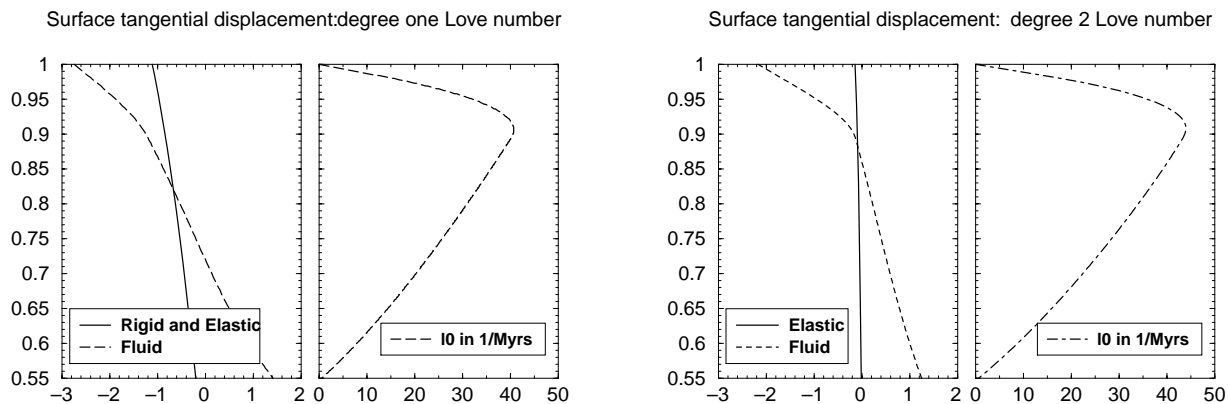
Figure 3. Kernels for the surface tangential displacement, for the degree n = 1 (left-hand panel) and the degree n = 2 (right-hand panel): elastic Love number (solid line), fluid Love number (dashed line) and l_0(r_o) in \text{Myr}^{-1} in dot-dashed line. The y-axis is \frac{r_o}{a} the normalized radius of the load.
