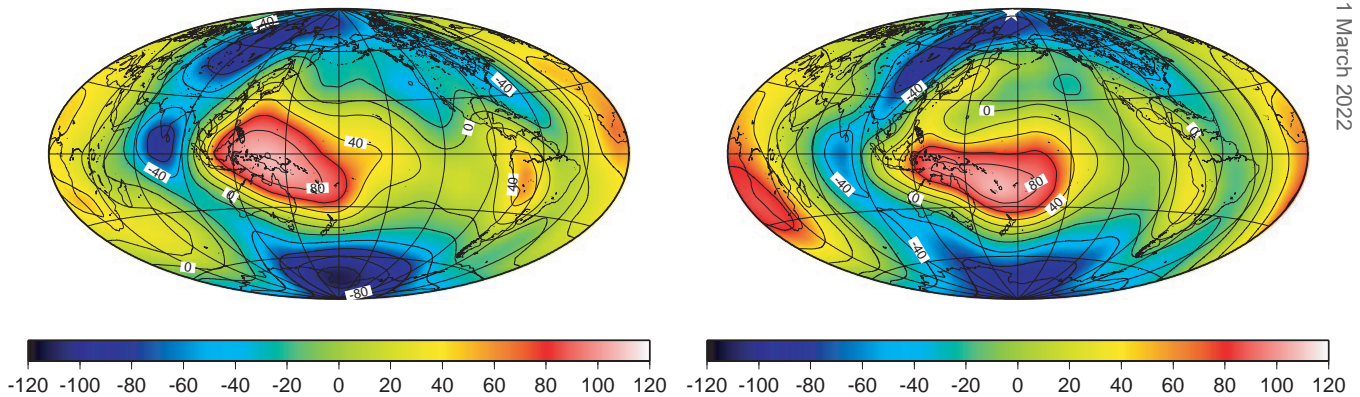
Figure 6. Geoid in metre, from degree 2 to 12. Color contour interval is 20 m. Left-hand panel: observed geoid from EIGEN-GM2008 (Heister et al. 2008) in which the hydrostatic reference ellipsoid (Nakiboglu 1979, 1982) and the effect of postglacial rebound have been corrected. The gravitational contribution of the postglacial rebound has been corrected using the simple model (three ice-sheets with the same dependence) detailed in Greff-Lefftz (2000) and our surface loading viscoelastic Love numbers for VR = 40 . Right-hand panel: present-day computed geoid induced by our mantle density heterogeneities model, for a mantle with a viscosity ratio VR = 40 , using geoid kernels plotted in Fig. 4.
