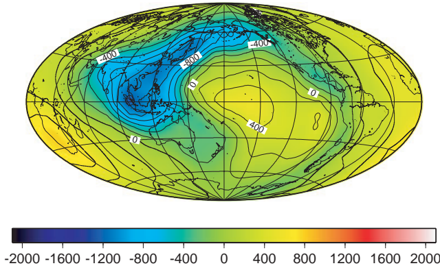
Figure 7. Surface topography from degree 1 to 12. The contour interval is 200 m.
