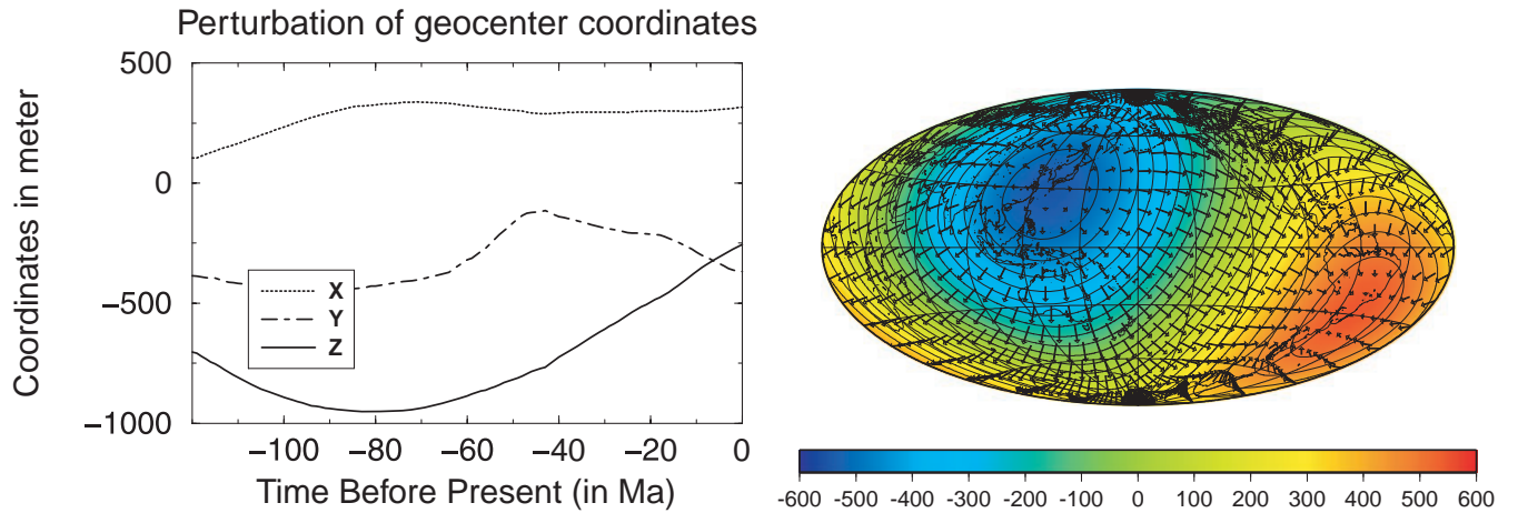
Figure 9. Temporal evolution of the coordinates of the geocentre (left-hand panel), and present-day degree 1 surface displacement with contour interval of 50 m (right-hand panel), in metre, induced by our time-dependent internal loads model, since 120 Ma.
