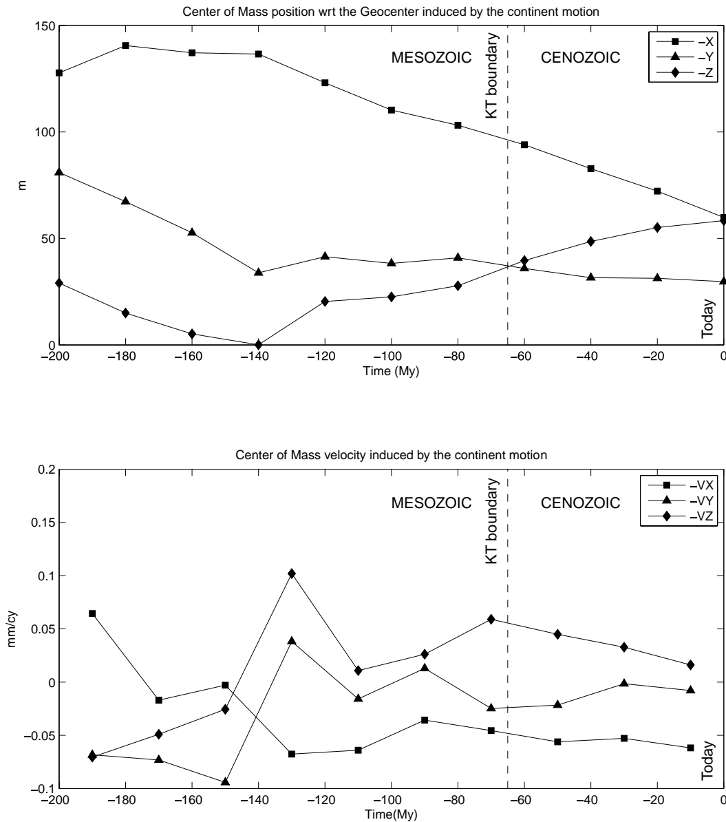
Figure 13. Centre of mass wrt geocentre position and velocity induced by the continent motion from 200 Ma to today.
