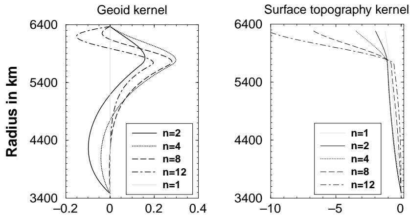
Figure 4. Geoid kernel and surface topography kernel for degree n = 1 (grey line), n = 2 (solid line), n = 4 (dotted line), n = 8 (dashed line) and n = 12 (dot-dashed line). The y-axis is r_o the radius of the load.
