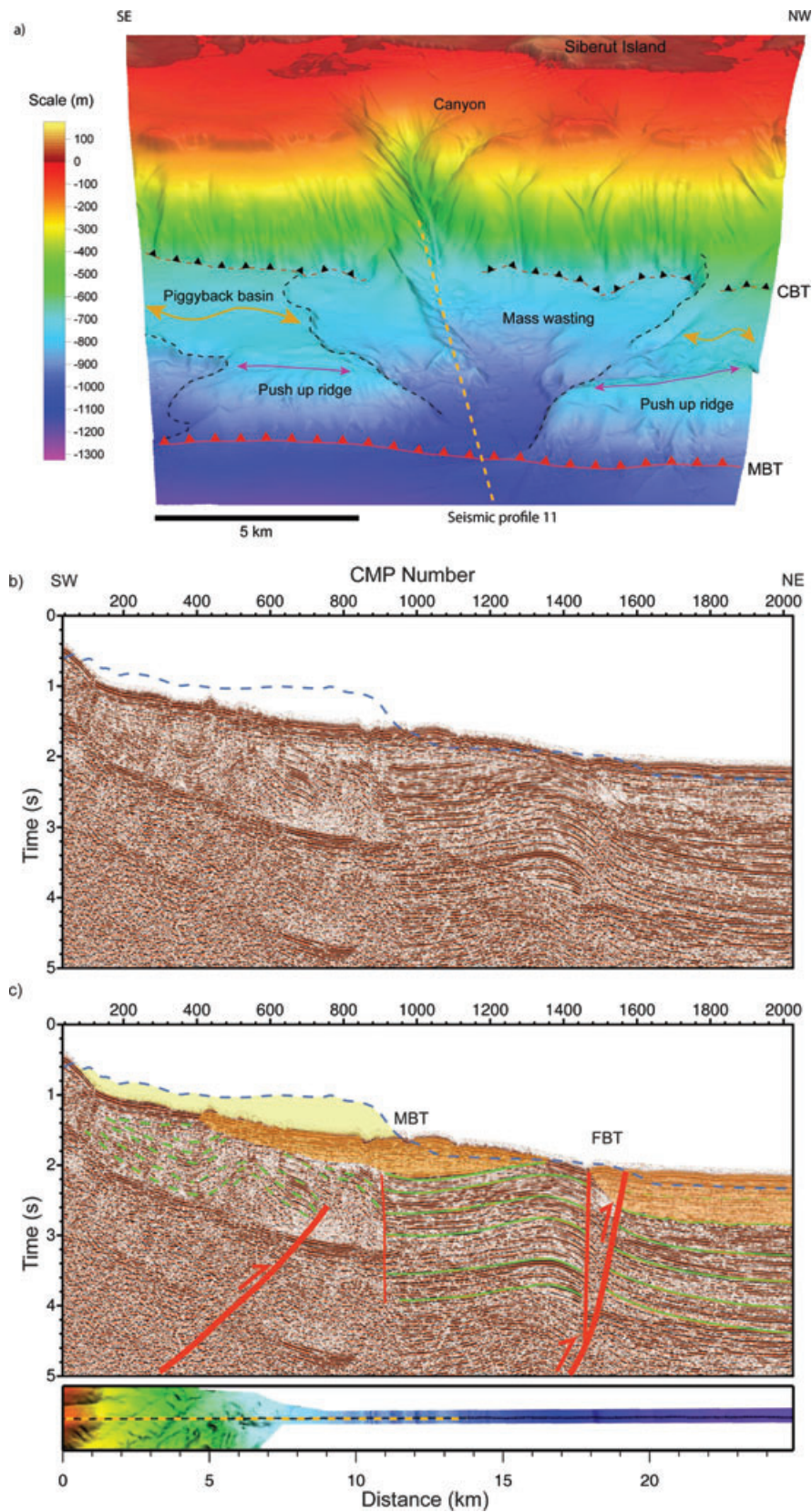
Figure 6. Mass wasting: (a) 3-D view of the mass wasting near 1.25^{\circ}\text{S} on Fig. 4. Black dashed lines mark boundary of mass wasted regions, purple arrows push-up ridges, mustard colour arrows piggyback basins. Uninterpreted (b) and interpreted (c) seismic profile 11 traversing the mass wasted region. Blue dashed curve shows the seafloor on profile 5 (Fig. 3b), yellow area is the difference between seafloor on profiles 5 and 11, possibly mass wasted, and brown coloured zone shows low reflectivity sediments, possibly debris flow. The portion of profile 11 on two images is marked by mustard colour dashed line.
