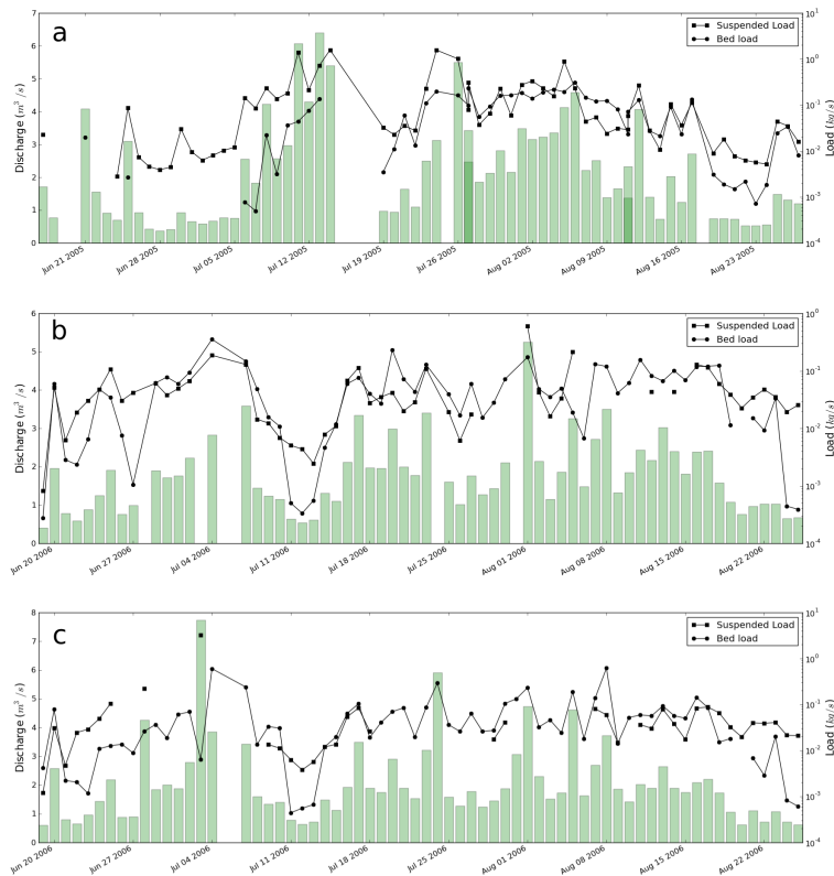
Fig. 8. Daily measurement of discharge, suspended load and bed load transport rates along the Urumqi River in its glacial valley. (a) site 1-1 in 2005, (b) site 1-1 in 2006, (c) site 1-2 in 2006.
