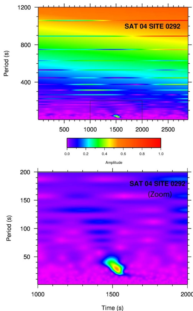
Figure 5 | Periodograms of the residual time-series of the satellite PRN 4 at the site 0292. The seismic signal is only visible in the period range 10–80s with a strongest amplitude in the \sim 30 - 50 s (20 to 35 mHz) period range.
