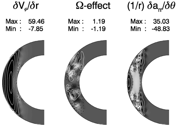
Fig. 5. Left: \partial\bar{V}_\phi/\partial r in units of v/L^2 . Middle: \Omega -effect as given by r\bar{B}_r \partial(r^{-1}\bar{V}_\phi)/\partial r + r^{-1} \sin\theta \bar{B}_\theta \partial(\sin\theta^{-1}\bar{V}_\phi)/\partial\theta (greyscale) and \bar{B}_\phi (superimposed contour lines, solid [dashed] lines indicate positive [negative] values). Right: (1/r)\partial a_{rr}/\partial\theta in units of v/L^2 . Otherwise, the contour plots are presented in the same style as in Fig. 4.
