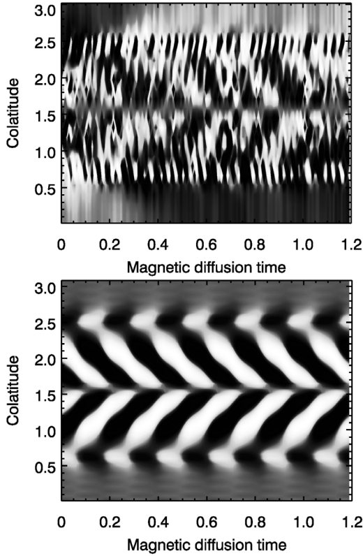
Fig. 3. Azimuthally averaged radial magnetic field at the outer shell boundary varying with time (butterfly diagram) resulting from a kinematic calculation with subtracted \Omega -effect ( top ) and a corresponding mean-field calculation ( bottom ). The contour plots are presented as in Fig. 2.
