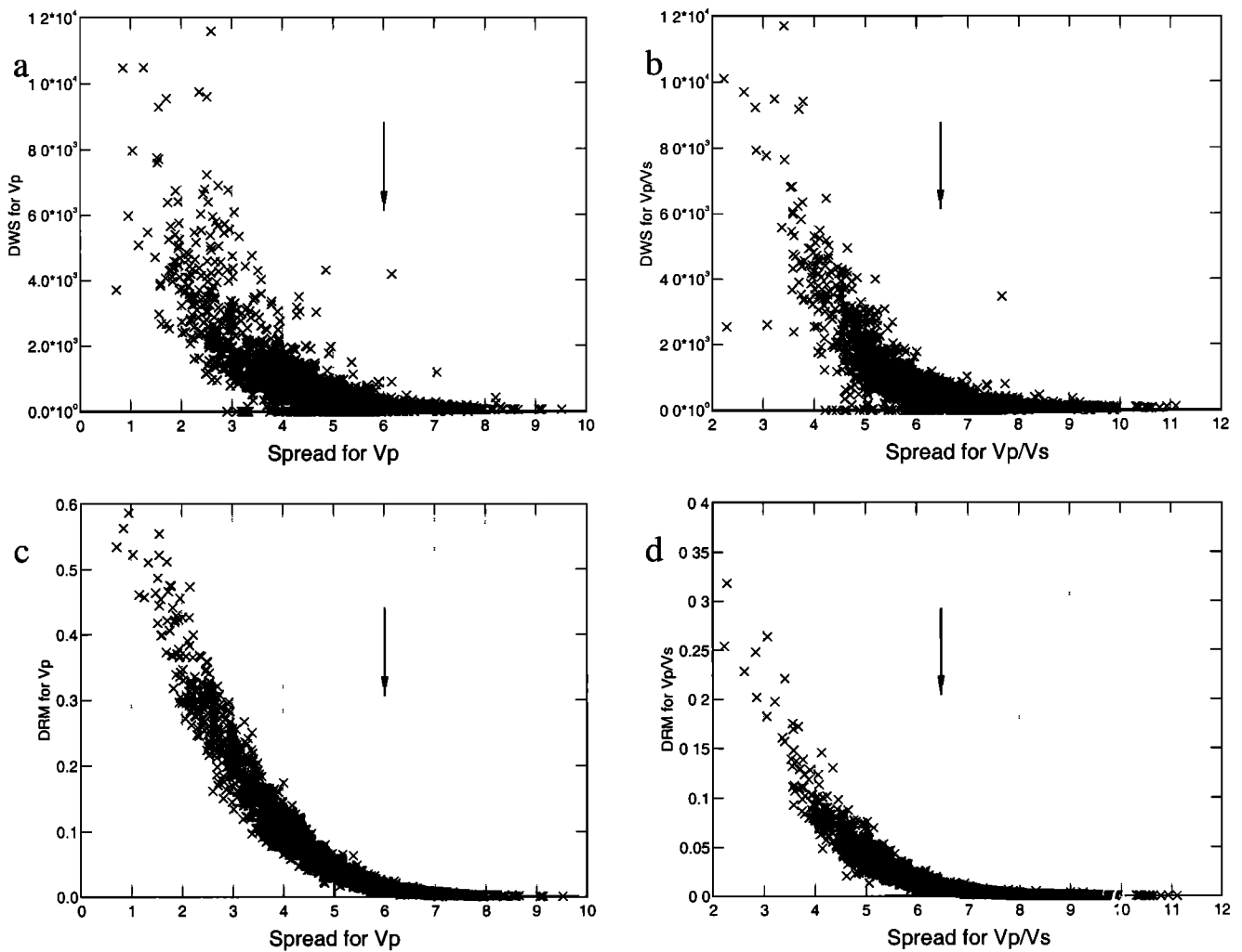
Figure 5. (a, b) Derivative weight sum (DWS) and (c, d) diagonal value of the resolution matrix (DRM) versus spread function values for V_P (Figures 5a and 5c) and V_P/V_S (Figures 5b and 5d) models computed from the direct inversion for the fine grid. The arrows indicate the threshold of spread-function chosen to delineate poorly resolved areas in subsequent velocity maps.
