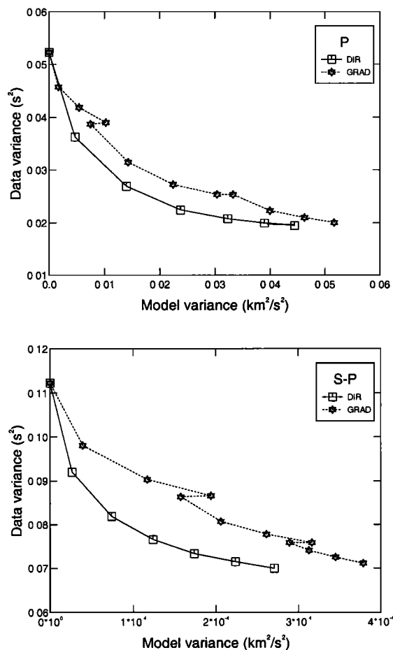
Figure 4. Data misfit versus model length for (top) P and (bottom) S - P data sets for the direct (DIR) and gradational (GRAD) inversions.
