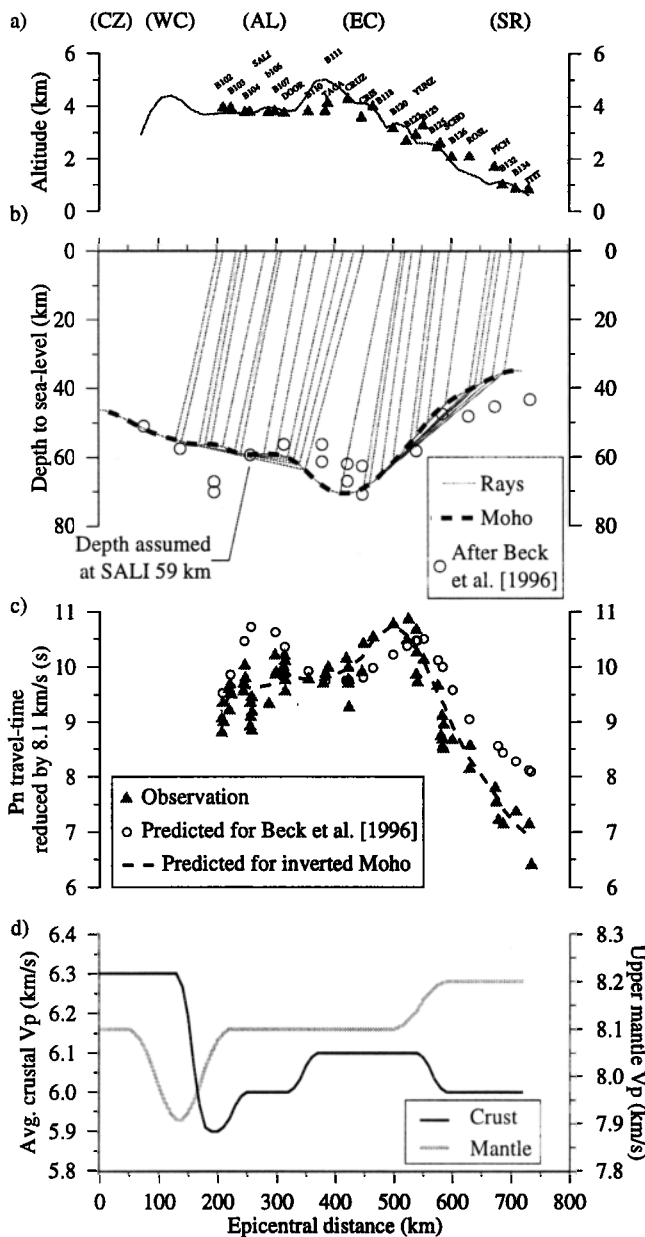
Figure 2. (a) Topography of the Central Andes along the profile. (b) Geometry of the Moho resulting from the inversion of P_n travel times (dashed line) and inferred by Beck et al. [1996] (circles) after conversion using our assumption of the lateral variations of the average crustal V_p (shown in Figure 2d). P_n raypaths (thin lines) are only shown to illustrate the relationship between a station and the emission point of the P_n at the Moho. (c) Fit between observed (triangles) and predicted P_n travel times for the inverted geometry of the Moho (dashed line) and the Moho inferred by Beck et al. [1996] (circles). (d) Lateral variations of the average velocity models modified from Wigger et al. [1994] and used in the Moho inversion.
