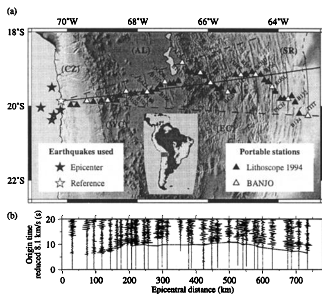
Figure 1. (a) Topographic map of the Central Andes showing the locations of the stations (triangles) and earthquakes (stars) used in this study. Station names are written only for stations used in this study. The aperture of the profile along its mean axis (solid line) through the reference earthquake epicenter (white star) is delineated by the long-dashed line. The arcs of circles represent the P_n wavefront. The main morpho-tectonic units are from west to east: Coastal Zone (CZ), Western Cordillera (WC), Altiplano (AL), Eastern Cordillera (EC), Subandean Range (SR). (b) Vertical component record section of the reference crustal earthquake (white star in Figure 1a). A reduction velocity of 8.1 km/s has been used. The P_n travel time curve is shown by the solid line.
