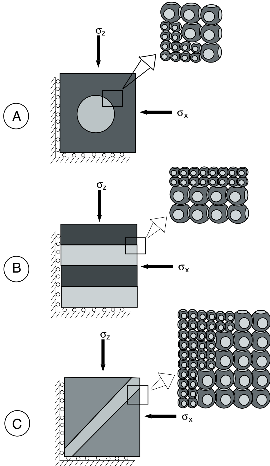
Figure 3. Domains where coupled pressure solution creep and local diffusive mass transport are simulated. Each element in the numerical grid contains a given number of grains with the same size. The domain is two-dimensional ( x and z directions) and has a thickness of one layer of grains in the y direction. The grain size and porosity can vary between the elements. Here are presented the three geometries simulated. In case (A) the grains size heterogeneity is located in a circular region in the center of the grid, case (B) corresponds to layers of alternating smaller and larger grain sizes and finally, in case (C) the small grains are located in a layer between coarser grained particles and are meant to represent fault gouge.
