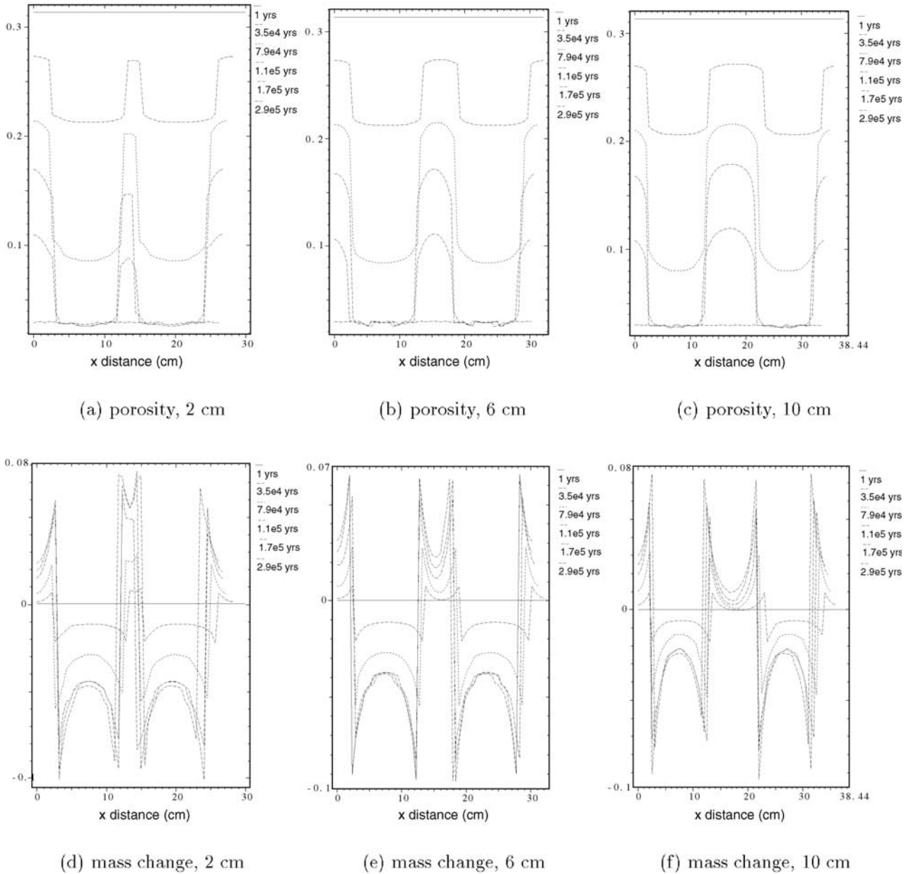
Figure 5. Compaction and porosity variations in the case of two concretions, represented as circles with grain size L_f = 90 micron whereas the grain size in the surroundings is L_f = 130 micron. The curves in plots (a), (b) and (c) indicate the porosity evolution along a line passing through the center of the two concretions. Plots (d), (e), and (f) represent the mass of silica transported by diffusion in a section passing through the two centers of the concretions. The distance between the concretions is 2 cm in plots (a) and (d), 6 cm in plots (b) and (e), and 10 cm in plots (c) and (f). As this distance increases, the interaction between the concretions becomes smaller.
