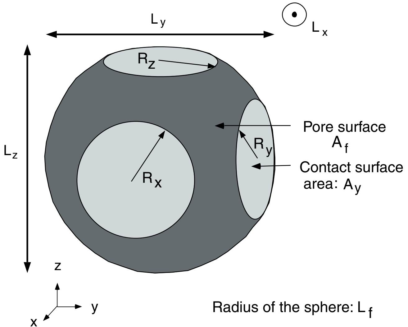
Figure 2. Schematic representation of a single grain for which the surface is divided into contacts with other grains (light areas) and free faces in contact with the pore fluid (dark area). Each grain has six neighbors, arranged in a cubic packing.
