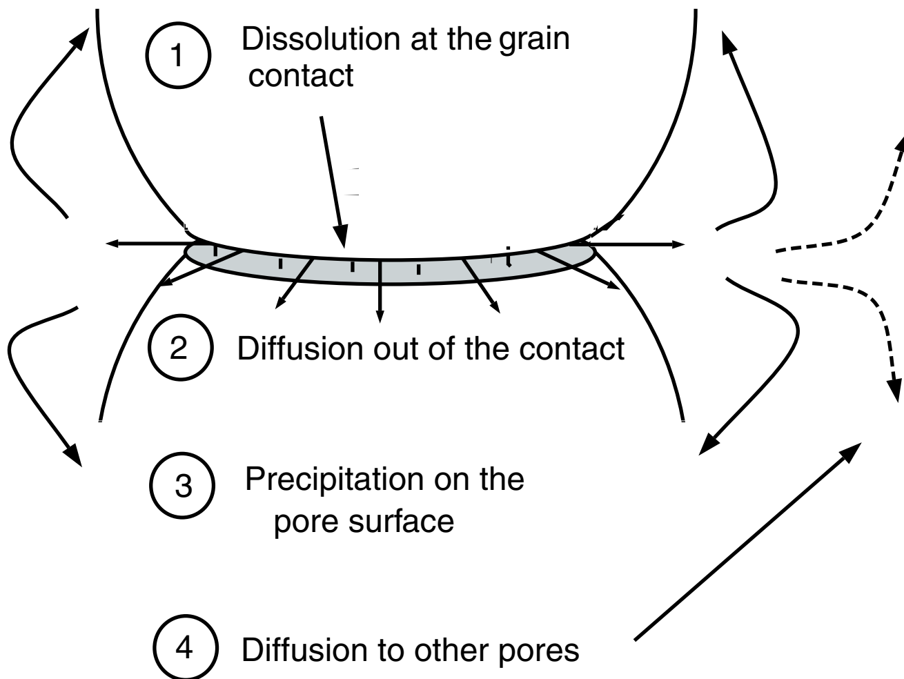
Figure 1. At a grain scale, pressure solution is a three-step process: (1) stress-enhanced dissolution at grain contacts, (2) diffusion along the contact to the pore, and (3) precipitation on the pore surface. If one considers that the system is not closed at the grain scale, a fourth step adds a level of complexity to the process: (4) transport between pores, which can lead to mass transport at decimeter or larger scales.
