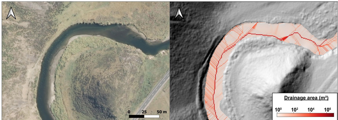
Figure 1. Aerial photo of a river near Wellington in New Zealand (left; LINZ, 2014) and the 1 m resolution LiDAR DEM (right; LINZ, 2017) showing drainage area values calculated by a D \infty flow routing where the river is wider than the grid resolution. Location: 1757118; 5414793 (NZTM2000).
