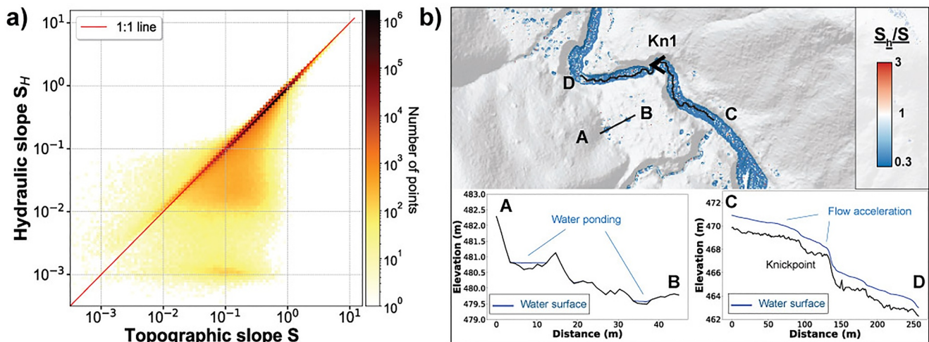
Figure 5. Comparison between the hydraulic slope S_h and the topographic slope S . (a) 2D histogram of S_h versus S . The number of bins in x and y axis is 100. (b) Subset of the Elder Creek catchment near knickpoint Kn1, showing the ratio between the two variables. Two cross sections show both situations where hydraulic slope is lower than topographic slope and vice versa.
