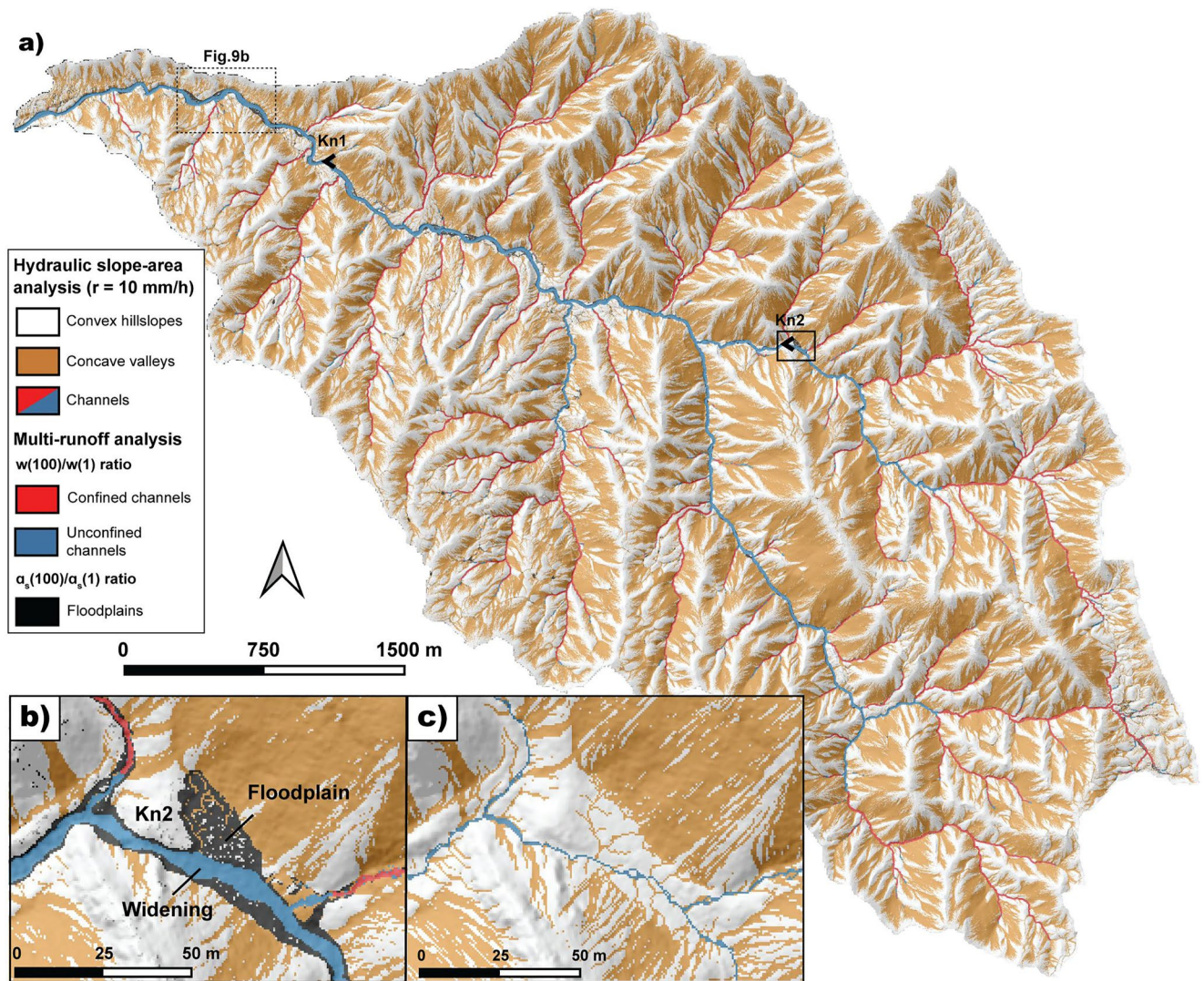
Figure 13. Map of the Elder Creek catchment showing geomorphic domains classified from the single runoff hydraulic slope-area ( r = 10 \text{ mm/hr} ) and multi-runoff w(r) and a_s(r) analyses. (a) Overview of the Elder Creek catchment map. An operation of dilatation has been applied to the channel domain to increase the river segment width by a factor of 2. This operation has not been applied in (b) and (c). Pixels in blue and red belongs to the channel domain. (b) Focus on knickpoint Kn2 for which an upstream widening and floodplains are observed. (c) Same area as (b) classified from the slope-area analysis.
