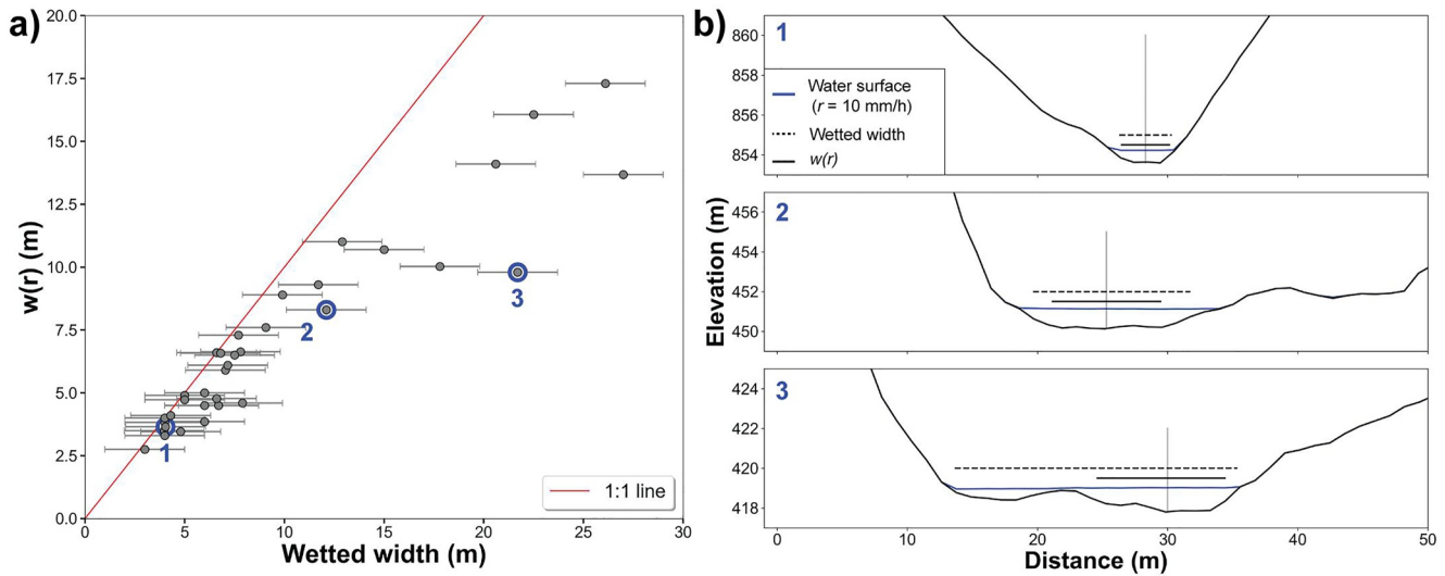
Figure 4. Effective flow width w(r) versus wetted width measured for 35 cross sections along the channel network for r = 10 mm/h. (a) w(r) versus wetted width. Wetted width is measured where water depth is higher than 10 cm. The measurement uncertainty of the wetted width is set to 2 m (1 pixel for each side of the channel). (b) Three cross-sections showing different channel morphologies for which: (1) w(r) equals the wetted width, (2) w(r) is lower than the wetted width and (3) w(r) \ll wetted width. The number associated to each section is shown in blue in (a).
