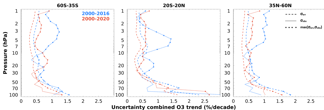
Figure 6. Decomposition of error terms for the combine trend estimates: propagation of errors from fit residuals ( \sigma_{\text{err}} , dashed lines) and standard error of the trend sample ( \sigma_{\text{obs}} , dotted lines) for LOTUS22 in red and LOTUS19 in blue for the three broad latitude bands. Combined trend uncertainty is shown by circle symbols that indicate the maximum of \sigma_{\text{err}} and \sigma_{\text{obs}} in each case.
