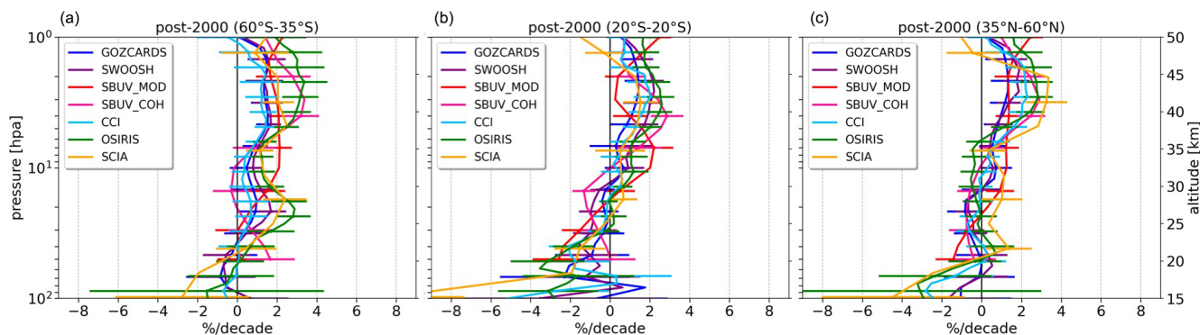
Figure 2. Merged satellite ozone trends with their 2\sigma uncertainties for the post-2000 period as estimated by the LOTUS regression model for latitude bands 60–35° S (a), 20° S–20° N (b) and 35–60° N (c). Coloured lines are the trend estimates from the individual merged datasets on their native vertical grid.
