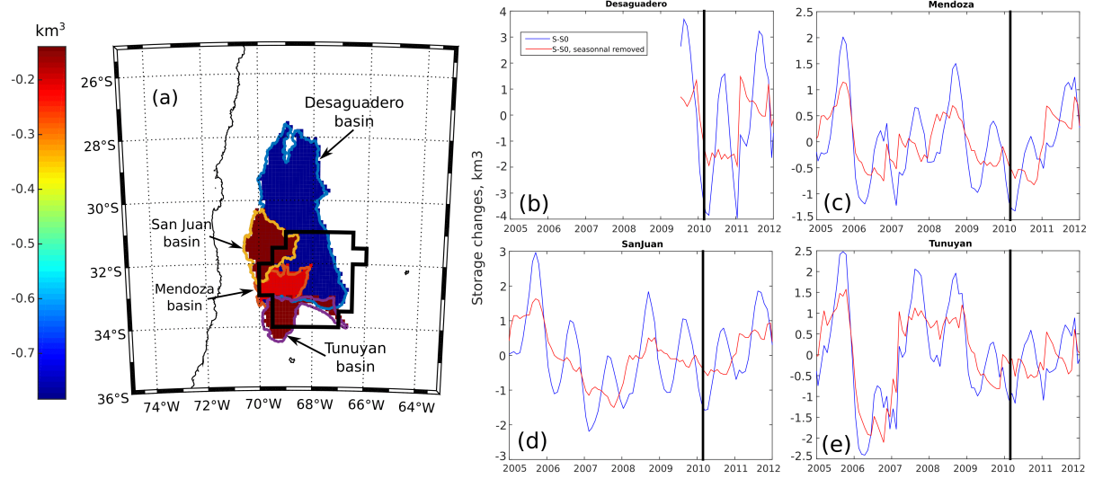
Figure 5: Estimated water storage variations of the Desaguadero, San Juan, Mendoza and Tunuyan basins in the region of Maule. Panel a: mass changes over the basins from the beginning of January to the end of February 2010, superimposed with the contour of the GRACE pre-seismic signal of Fig. 1a (black line). Panels b-e: time series of the water storage variations for each basin, before and after removing a seasonal cycle.
