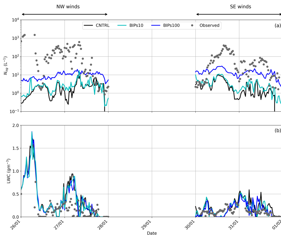
Figure 7. Time series of (a) total N_{\text{ice}} and (b) LWC predicted between 26 January and 1 February 2014 by the two sensitivity simulations accounting for the effect of blowing snow, i.e., BIPs10 (cyan line) and BIPs100 (blue line).
