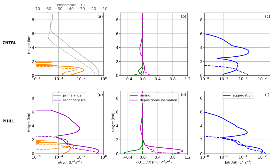
Figure 6. Vertical profiles of (a, d) primary and secondary ice production, (b, e) riming and vapor deposition or sublimation, and (c, f) snow aggregation produced by the CNTRL (a–c) and PHILL (d–f) simulations at 17:00 UTC on 26 January (solid line) and at 19:00 UTC on 30 January (dashed line). The vertical profile of simulated temperature is also superimposed in panel (a). The cloud liquid water content ( Q_C ) is shown in panels (b) and (e) to represent the tendency due to riming, while the mass mixing ratio of the ice and snow species ( Q_i + Q_s ), represents the relative tendencies due to vapor deposition or sublimation. Note that the tendencies due to snow aggregation in panels (c) and (f) are presented in absolute values. The height is given in km a.g.l.
