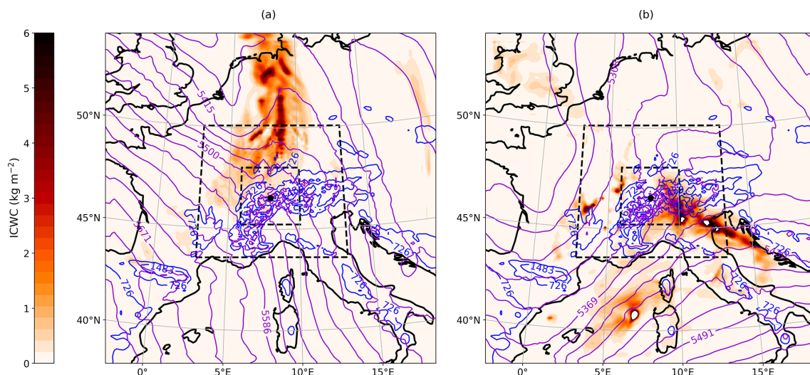
Figure 1. Map of synoptic conditions around JFJ station at (a) 00:00 UTC, 26 January 2014, and (b) 00:00 UTC, 30 January 2014, from the control simulation (12 km resolution domain). The purple (blue) contours show the 500 hPa geopotential height in meters (the terrain heights in meters). The color shading shows the vertically integrated condensed water content (in kilograms per square meter; hereafter \text{kg m}^{-2} ). The black dashed lines delimit the 3 and 1 km resolution domains, while the black dot indicates the location of the JFJ station.
