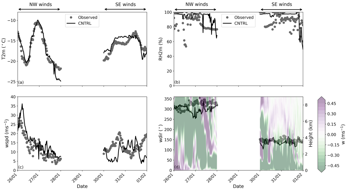
Figure 2. Time series of (a) temperature (T2m), (b) relative humidity with respect to liquid phase at 2 m height (RH2m), (c) wind speed (wspd), and (d) wind direction (wdir). Gray circles indicate measurements collected between 26 January and 1 February 2014 at JFJ station, while modeled values from the CNTRL simulation are shown with a black line. The semi-transparent contour plot represents the vertical velocity ( w ) profile predicted by the CNTRL simulation. Each day starts at 00:00 UTC.
