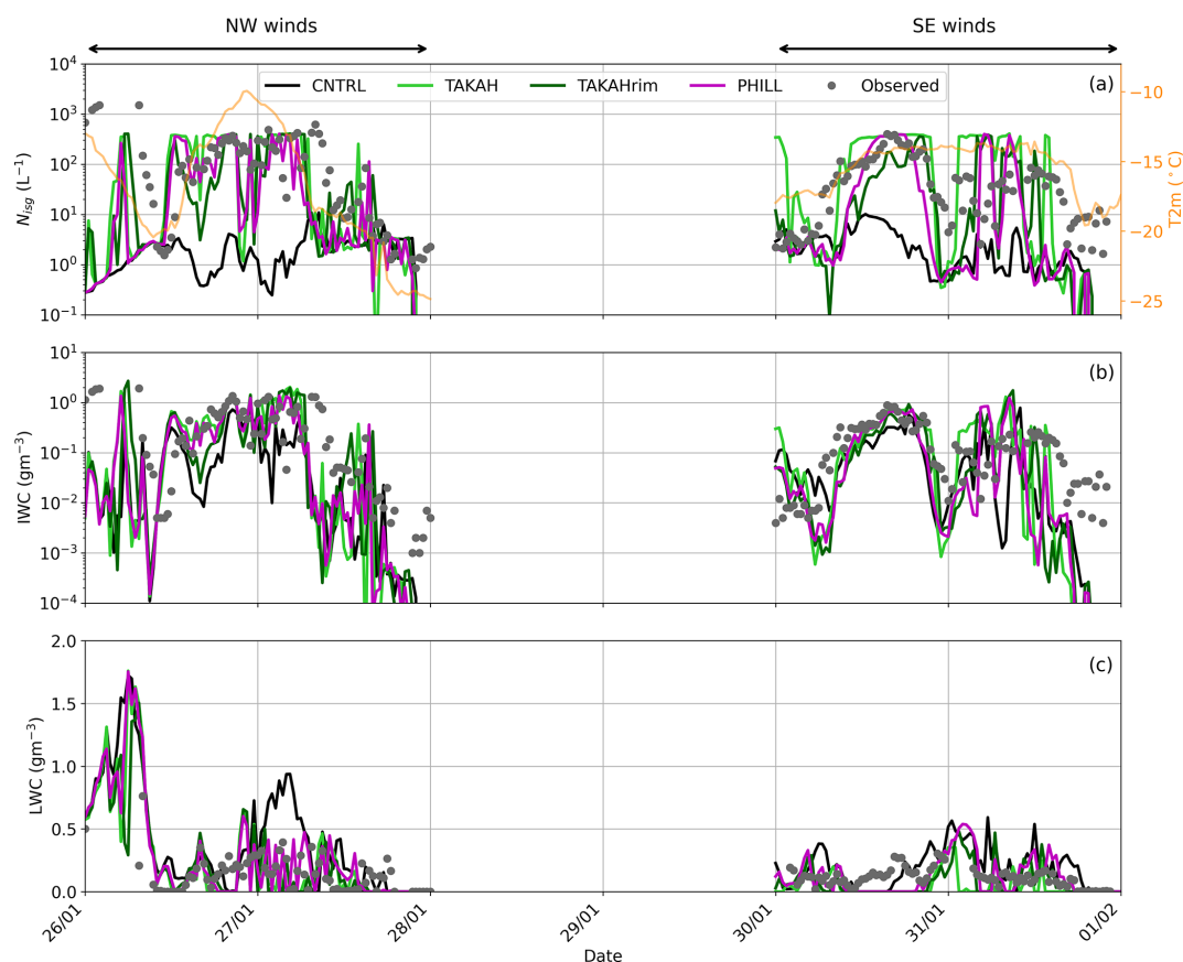
Figure 3. Time series of (a) total N_{\text{ice}} and temperature at 2 m height (orange line), (b) IWC, and (c) LWC, predicted by the CNTRL (black line), TAKAH (light green line), TAKAHrim (dark green), and PHILL (magenta line) simulations between 26 January and 1 February 2014. The gray dots in all three panels represent the 2D-S ICNCs, the inferred IWC, and the CDP LWC measured at the JFJ station, respectively. Note the logarithmic y axes in panels (a) and (b).
