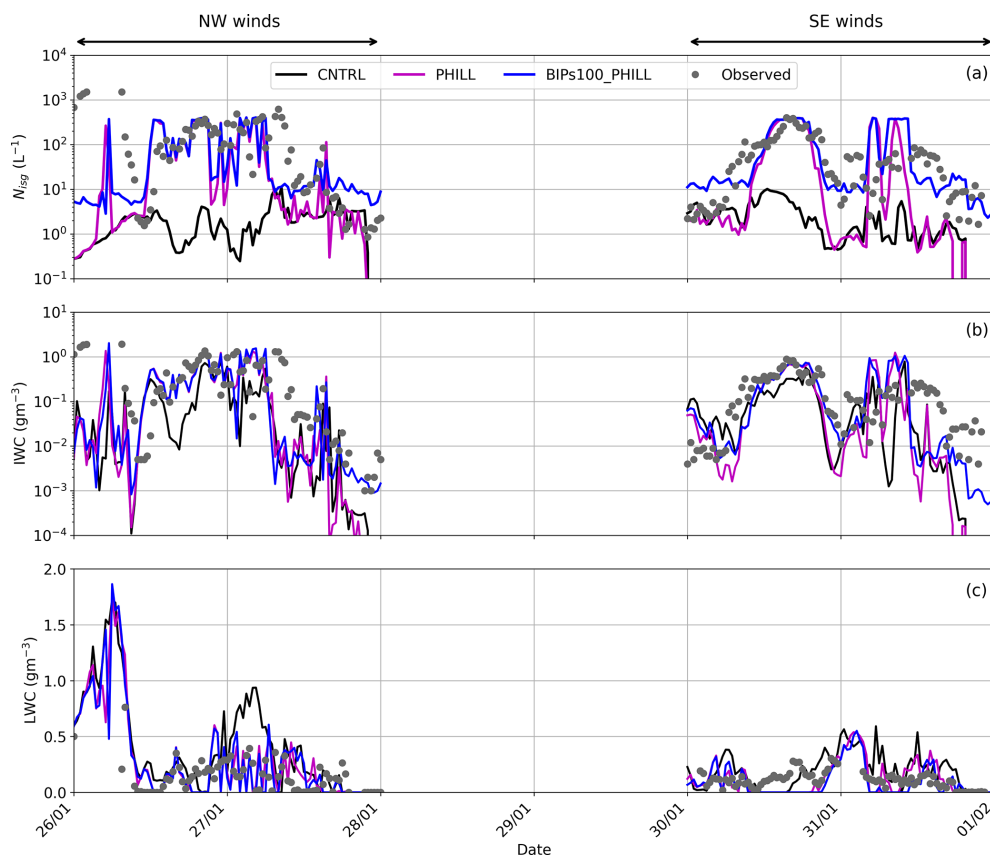
Figure 8. Time series of (a) total N_{\text{ice}} , (b) IWC, and (c) LWC predicted between 26 January and 1 February 2014 by the sensitivity simulation BIPs100_PHILL (blue line), which examines the combined effect of ice multiplication through BR and blowing snow.
