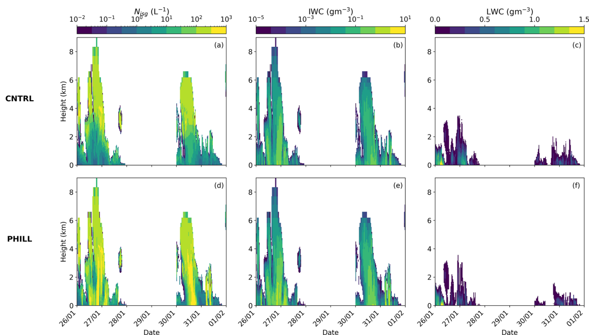
Figure 5. Time–height plots of total N_{\text{issg}} (a, d), IWC (b, e), and LWC (c, f) produced by CNTRL (a–c) and PHILL (d–f) simulations between 26 January and 1 February 2014. The height is given in km a.g.l.
