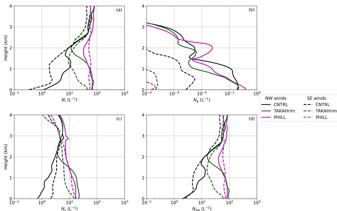
Figure 4. Mean vertical profiles of (a) N_i , (b) N_g , (c) N_s , and (d) total N_{\text{isg}} predicted by the CNTRL (black), TAKAHrim (dark green), and PHILL (magenta) simulations for the NW (solid lines) and SE (dashed lines) cases. Note the different scale on the x axis of the N_g vertical distribution. The height is given in kilometers above ground level (hereafter km a.g.l.).
