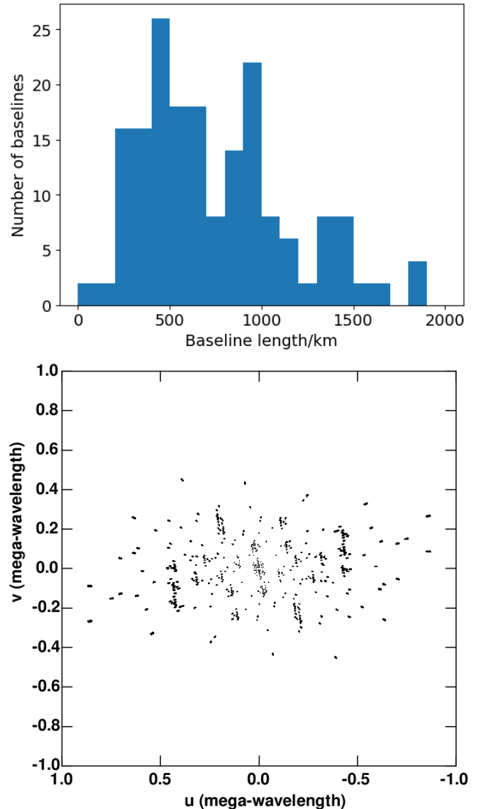
Fig. 1. Lengths and u-v coverage of the baselines used in the LOFAR observations. Top: Distribution of LOFAR baseline lengths between international stations. Core and remote LOFAR stations have baselines up to 100 km, so a gap in the u-v coverage still exists between 100 and 200 km. The longest baseline, 1890 km between Birr (Ireland) and Baldy (Poland) will be exceeded soon with the advent of the station in Irbene (Latvia). Bottom: Snapshot u-v plane coverage for a source at 34^\circ declination.
