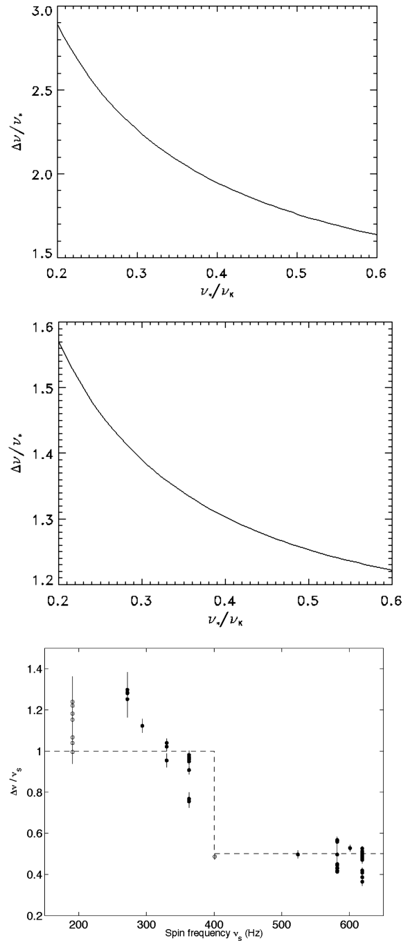
Figure 2. The upper plot shows the dimensionless quantity \nu_w(r_0 = 0.8r_M) - \nu_K(r_M)/\nu_* = \Delta\nu/\nu_* in our model, when \nu_*/\nu_K(r_M) varies. \Delta\nu is the frequency difference between the two kilohertz QPO, \nu_* is the neutron star spin frequency and \nu_K(r_M) is the rotation frequency at the inner edge of the Keplerian disc. The lower plot is the observational data as plotted by Méndez & Belloni (2007). The shape of the curves is similar, although the numerical values differ, as explained in the text.
