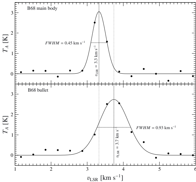
Fig. C.1. ^{13}\text{CO} (2–1) spectra extracted at two positions in the corresponding map. The upper spectrum shows a line on the western rim of B68 (RA (J2000) = 17 h 22 m 34.1, Dec (J2000) = −23°49′53''), while the lower spectrum is taken at the location of the point source mentioned in Sect. 4.2. A Gaussian profile fit was applied to both spectra.
