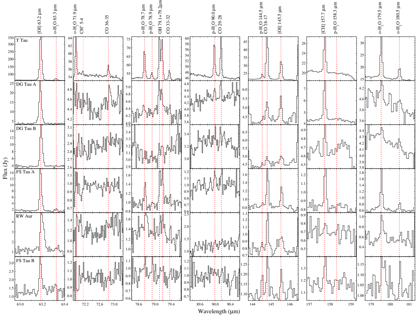
Fig. 1. Spectral ranges covered by the Herschel /PACS observations for all of the sources in the sample. The wavelengths of the targeted atomic ([O I], [C II]) and molecular ( \text{H}_2\text{O} , OH, CO) lines are shown by the vertical dotted red lines.
