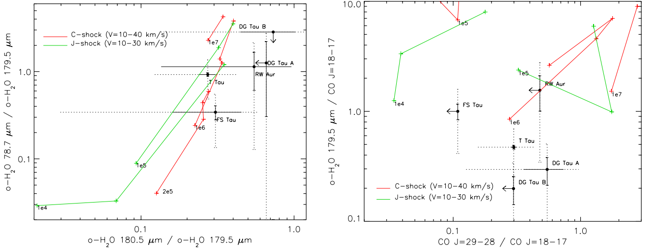
Fig. 6. Observed H 2 O and CO line ratios (black dots) are compared with the predictions of slow C-type (red lines) and J-type (green lines) shock models (Flower & Pineau Des Forêts 2010). The solid lines indicate the errors due to the line signal-to-noise, while the dashed lines indicate the total error, obtained by adding the 30% error in the PACS flux calibration. The crosses along the red and green curves correspond to increasing shock velocity, from 10 km s -1 to 40 km s -1 (C-type shocks) or from 10 km s -1 to 30 km s -1 (J-type shocks). At the lowest velocity ( V_{\text{shock}} = 10 \text{ km s}^{-1} ), the pre-shock density is given.
