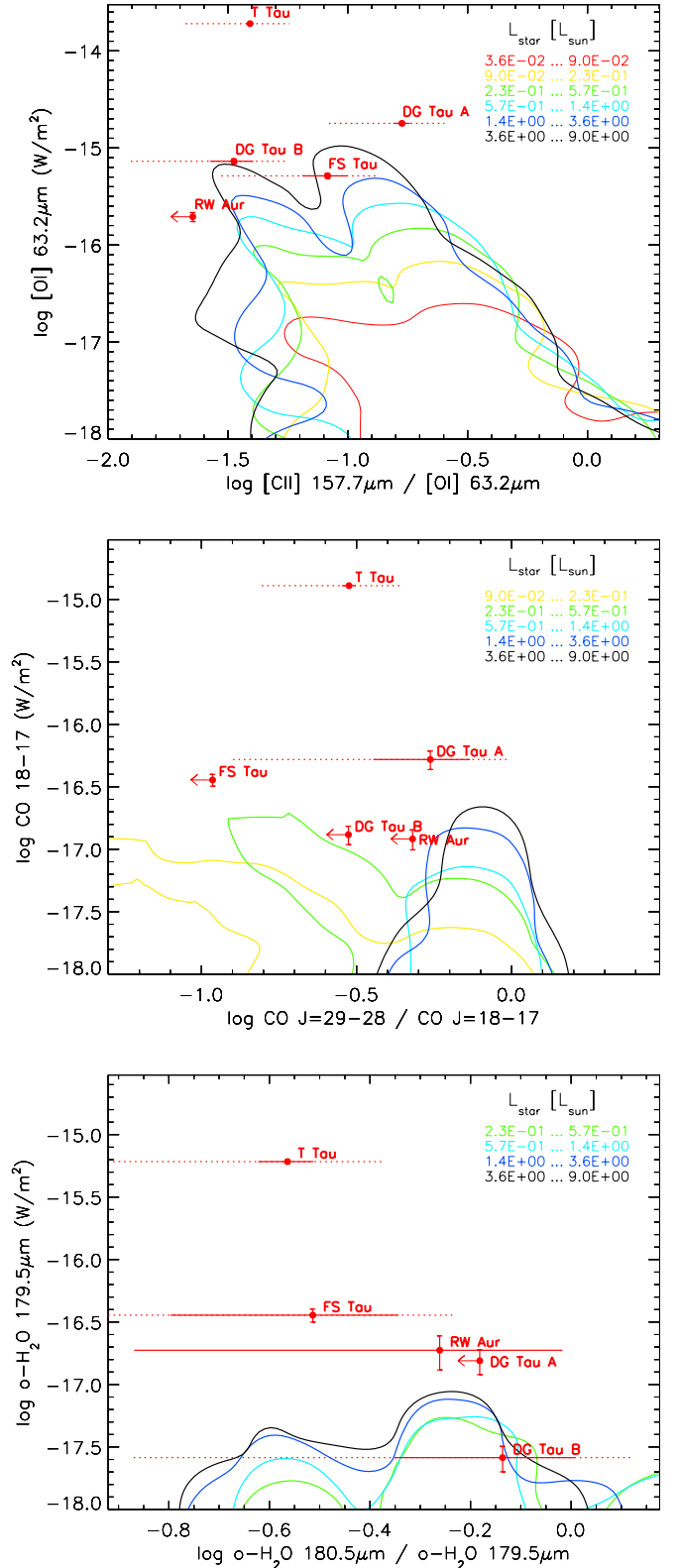
Fig. 4. Observed [O I], [C II], CO, and H 2 O line fluxes and ratios (red dots) are compared with predictions from a subsample of disk models from the DENT grid (Woitke et al. 2010; Kamp et al. 2011). Contours encircle 85% of the DENT disks for star luminosity values from 10^{-2} L_\odot to 9 L_\odot (red, yellow, green, cyan, blue, and black contours). The total errors on the observed values (dotted red lines) are obtained summing the error due to the line signal-to-noise (solid red lines) and the 30% error affecting PACS flux calibration. The subsample of disk models is obtained by selecting M \leq 2.5 M_\odot , T_{\text{eff}} \leq 5500 K, L \leq 9 L_\odot , R_{\text{in}} = R_{\text{subl}} , and dust-to-gas ratio = 0.01.
