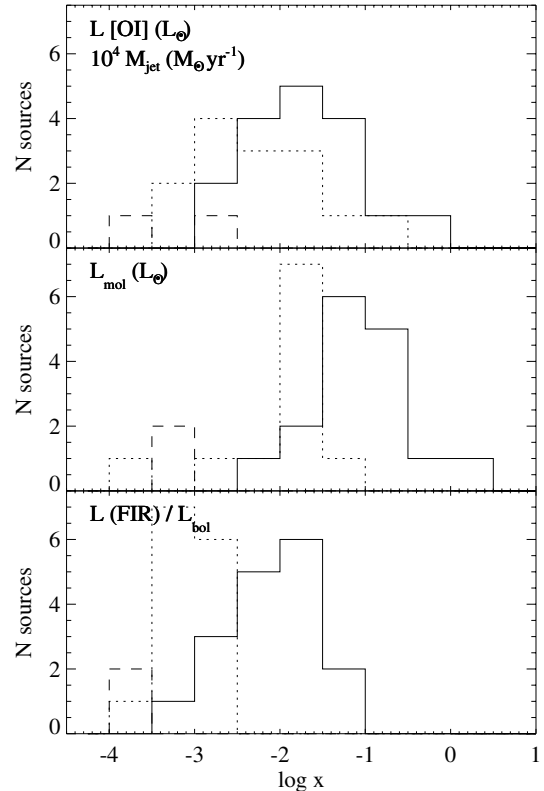
Fig. 9. Histograms of L [O I] (upper panel), L_{\text{mol}} (middle panel), and L (FIR)/ L_{\text{bol}} (bottom panel) for Class 0, I, and II sources (solid, dotted, and dashed lines).
