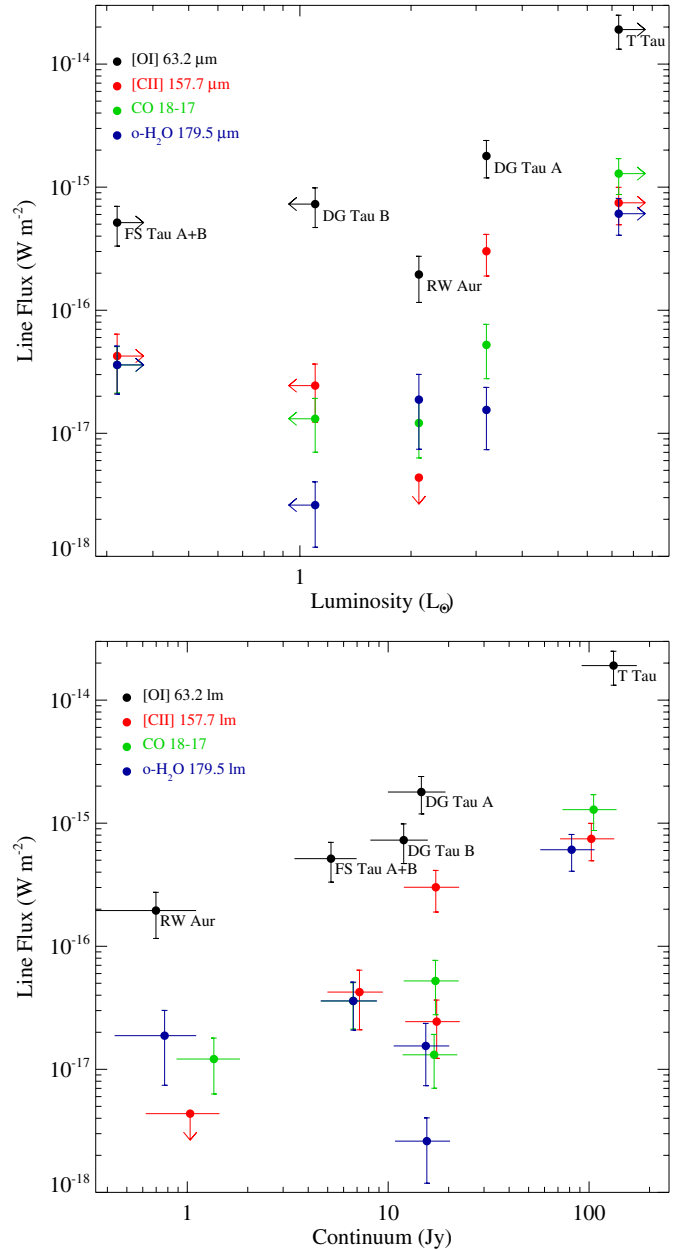
Fig. 3. The fluxes of the [O I] 63 \mu\text{m} , the [C II] 158 \mu\text{m} , the CO J = 18 -17, and the o- \text{H}_2\text{O} 179.5 \mu\text{m} lines are plotted versus the source luminosity (upper panel) and their adjacent continuum (lower panel) for all the sources in our sample (black, red, green, and blue dots). For FS Tau A+B and T Tau N+S the plotted source luminosity is a lower limit, since L_* of the Class I components FS Tau B and T Tau S is unknown. The upper limit on the stellar luminosity for DG Tau B corresponds to its bolometric luminosity as estimated by Kruger et al. (2011).
