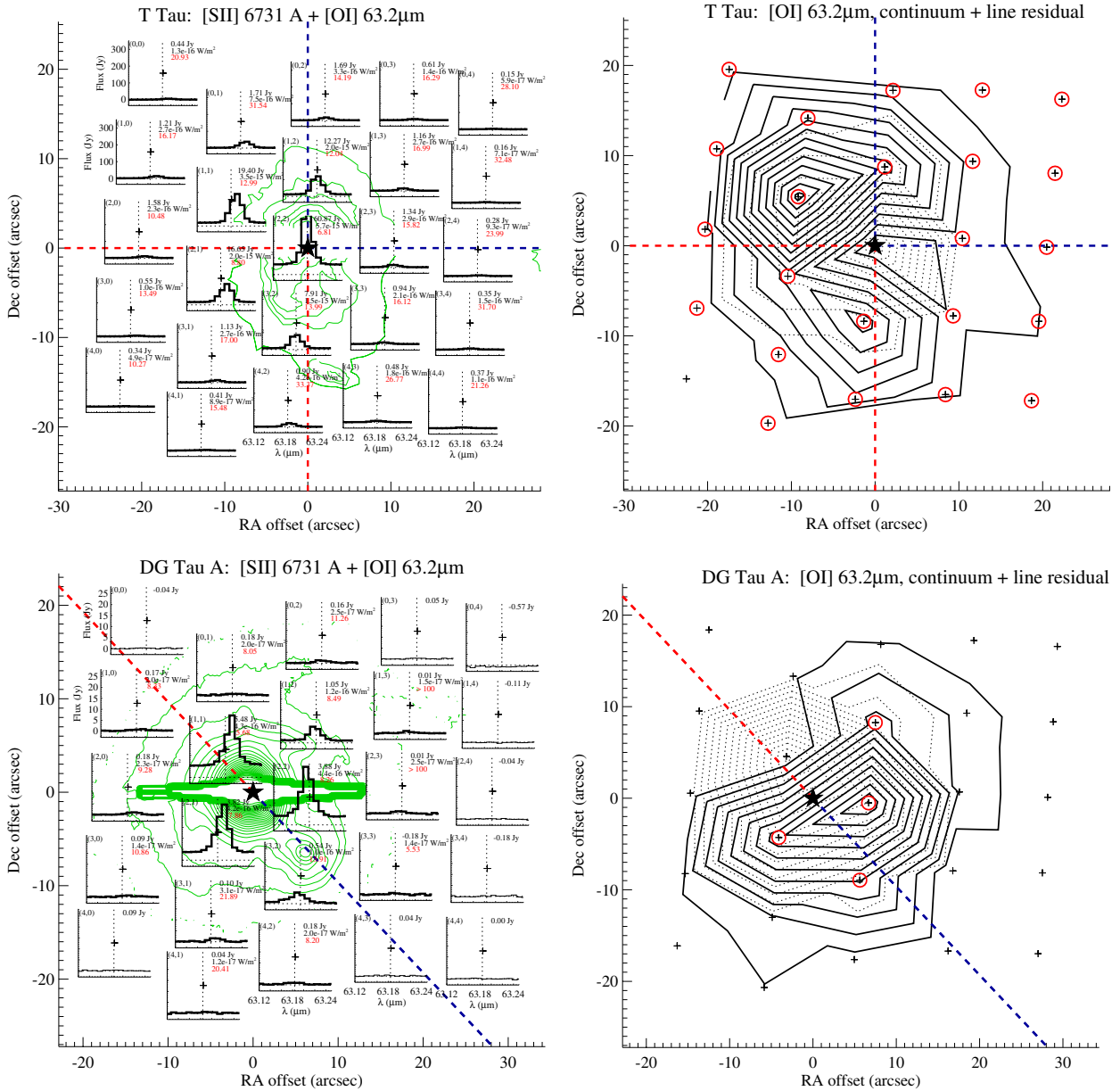
Fig. 2. Left panel: [O I] 63 \mu\text{m} line spectra in the 25 spaxels of the PACS array. Each spaxel is labelled by its (x, y) index and its position is indicated by a black cross. The RA and Declination offsets with respect to the source (in arcseconds) are indicated on the x and y axis. The black star is the source position and the blue/red dashed lines show the position angle of the optical-jet blue/red lobe. In each spectrum, vertical and horizontal dotted lines show the line wavelength and the zero flux level, respectively. In those spaxels where the line is detected above the 3\sigma level, the spectrum is drawn with a black thick line, and the estimated continuum level (in Jy), line flux (in \text{W m}^{-2} ), and line-to-continuum ratio (in red) are indicated. Where the line is not detected only the estimated continuum level (in Jy) is given. The optical-jet emission in the [S II] \lambda\lambda 6716, 6731 \text{\AA} forbidden lines is overplotted (green contours). Contours are from Solf & Böhm (1999) (T Tau), Eisloffel & Mundt (1998) (DG Tau A, DG Tau B, FS Tau A+B), and Dougados et al. (2000) (RW Aur). Right panel: contour levels of continuum (dotted lines) and line residual (solid lines) emission obtained from the analysis in Appendix B. The spaxels where residual line emission is detected with a confidence level \geq 5 are highlighted by a red circle (for RW Aur the red circles indicate residual emission above the 2\sigma level). The contours indicate that the line emission is shifted and/or more extended with respect to the continuum emission along the optical jet PA.
