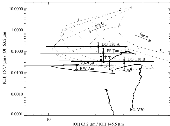
Fig. 5. Observed atomic line ratios are compared with predictions from PDR (dotted lines, Kaufman et al. 1999) and fast J-type shock (solid lines, Hollenbach & McKee 1989) models. For the PDR models, the labels on the broken curves indicate the gas density ( n ) and the intensity of the FUV field ( G_0 ), respectively. For the shock models, the pre-shock density is marked at the lowest shock-velocity point ( V_{\text{shock}} = 30 \text{ km s}^{-1} ), and the shock velocity increases along the full curves, up to V_{\text{shock}} = 150 \text{ km s}^{-1} .
