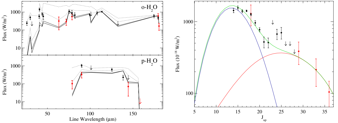
Fig. 8. All the available ISO (black points) and Herschel (red points) observations of H 2 O (left panel) and CO (right panel) lines for T Tau are shown. Left panel: line fluxes predicted by a slow C-shock for an emitting area of \sim 360 AU diameter and pre-shock density of n = 10^6 \text{ cm}^{-3} (velocity V = 20\text{--}30 \text{ km s}^{-1} , solid lines), or n = 10^7 \text{ cm}^{-3} ( V = 10\text{--}20 \text{ km s}^{-1} , dotted lines). The low-excitation water lines are well reproduced by C-shock with pre-shock density of 10^6 \text{ cm}^{-3} while the higher excitation lines require higher pre-shock density. Right panel: CO line fluxes predicted by: a C-shock model ( n = 10^6 \text{ cm}^{-3} , V = 20\text{--}30 \text{ km s}^{-1} , emitting area diameter, D = 360 AU, red line); an LVG warm gas component ( n = 10^6 , T = 300 \text{ K} , D = 360 AU, N_{\text{CO}} = 1.5 \times 10^{18} \text{ cm}^{-2} , blue line); the sum of the two models (green line). While the high- J CO lines are well reproduced by the same C-shock model used for water lines, a warm gas component is required to simultaneously fit the lower- J lines observed with ISO (down to J_{\text{up}} = 14 ).
