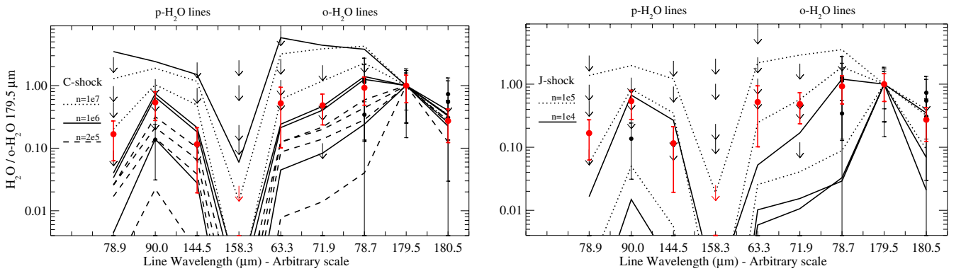
Fig. 7. Observed H 2 O line ratios for T Tau (red points/arrows) are compared with the predictions of C-type (left panel) and J-type (right panel) shock models (Flower & Pineau Des Forêts 2010) with relatively high pre-shock densities. The H 2 O line ratios and upper limits for the other sources in the sample are overlotted (black points and arrows).
