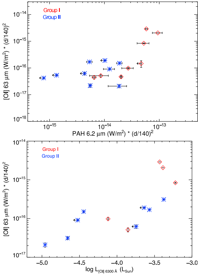
Fig. 10. Top: [O I] 63 \mu\text{m} line flux versus PAH 6.2 \mu\text{m} line flux. Bottom: [O I] 63 \mu\text{m} line flux versus the luminosity of [O I] 6300 Å. Diamonds are group I sources, asterisks are group II sources.
