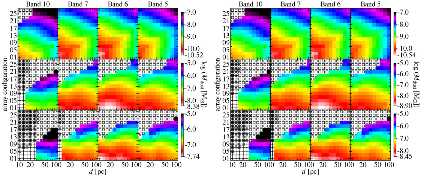
Fig. 5. Maps of the 10\sigma sensitivity of ALMA to face-on seen ( left ) and edge-on seen ( right ) debris disks as a function of the distance and array configuration (spatial resolution) for different wavelengths of observations. The three rows refer to different disk extents given by r_{in} of 5 AU ( top ), 50 AU ( middle ), and 100 AU ( bottom ). Disk mass can be converted into fractional luminosity following Eq. (3). For details about the model images and about the simulation of observations see Sects. 4.1.1 and 4.1.2. The detectable disk mass is color-coded and can be converted into fractional luminosity following Eq. (3). White pixels with symbols mark positions where the simulations failed or observations are impossible for various reasons denoted by the symbols as follows (see Sect. 4.1.3 for more details): cross – the spatial extent of the disk is larger than the field of view of a single pointing, \times – the disk is “resolved out” (the radial width of the ring is larger than the largest scale detectable), open square – artifacts of the image reconstruction caused by deficiencies of the model image dominate the simulated observations.
