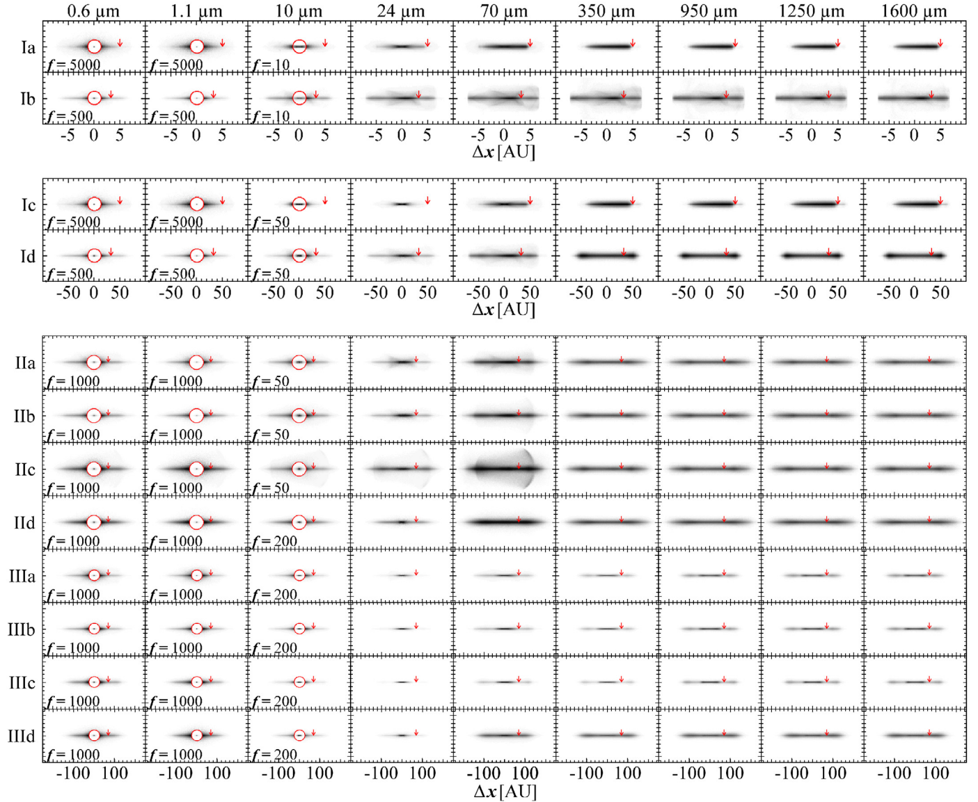
Fig. 3. Same as Figs. 1 and 2, but for an edge-on orientation of the disk. The position of the planet is indicated by the red arrow in each image. The flux is given in arbitrary units and displayed in a logarithmic stretch from zero to peak value for model sequence I, from zero to 1/2 of the peak value at wavelengths up to 24\,\mu\text{m} for model sequence II and III, and at longer wavelengths from zero to 1/2 of the peak value for model sequence II and to the peak value for model sequence III. Note that a disk without a planet would show a smooth, featureless radial surface brightness distribution (besides the possible signpost of inner and outer disk radius).
