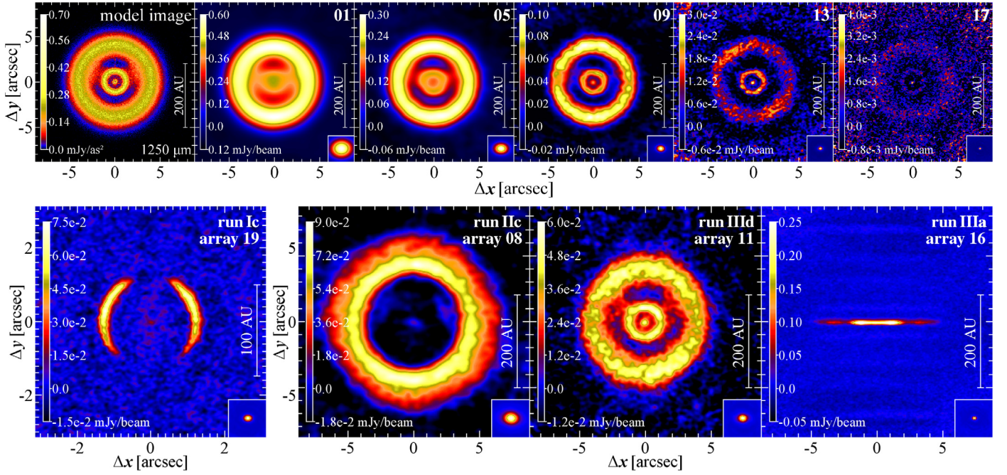
Fig. 6. Top: simulated ALMA observations of the model image resulting from run IIId (face-on orientation) for different array configurations. Only the results from a representative number of array configurations are shown. The number in the upper-right corner of each image denotes the array number. The corresponding beam is displayed in the lower-right corner of each image. Bottom: simulated ALMA observations of all selected model images. The optimum array configurations have been selected. The run and the array number are displayed in the upper-right corner, the corresponding beam is displayed in the lower-right corner of each image. All observations were simulated for Band 6 (central wavelength 1250 \mu\text{m} ).
