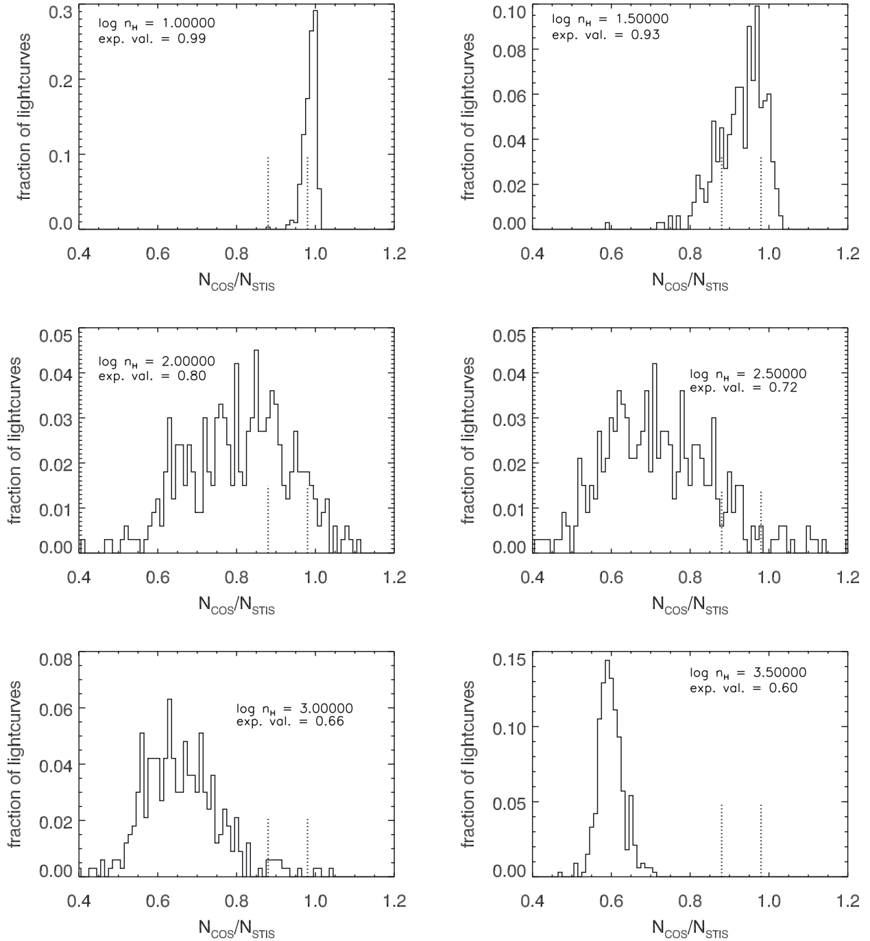
Fig. 5. Determining the upper limit for n_{\text{H}} of the absorber. This example shows the results for trough T2, based on the C IV column density measurements. For each of the 935 simulated light curves (see Sect. 5), we explicitly solve the time-dependent photoionization equations and calculate the expected ratio of C IV column density over a time period equal to the differences between the STIS and COS epochs. Each panel represents the fractional solution distribution of N(\text{C IV})_{\text{COS}}/N(\text{C IV})_{\text{STIS}} for a given \log(n_{\text{H}}) ( \text{cm}^{-3} ), which increases in the panels from left to right and top to bottom. The vertical dashed lines show the positive and negative 1\sigma errors on the measured value. We determine an n_{\text{H}} upper limit by increasing n_{\text{H}} until more than 99% of the calculated N(\text{C IV})_{\text{COS}}/N(\text{C IV})_{\text{STIS}} are outside the error bars. In this example, we find n_{\text{H}} < 10^{3.2} \text{ cm}^{-3} .
