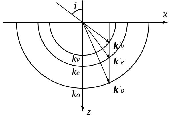
Fig. 4. In case 2, the optical axis is perpendicular to the plane of incidence. The two schematics are drawn as in case 1.
