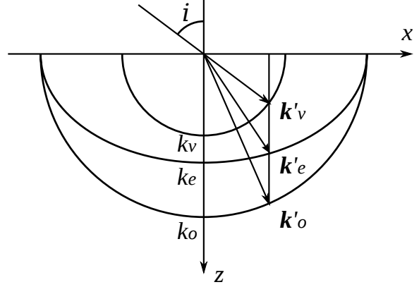
Fig. 3. In case 1, the optical axis is along the x direction. Left: a schematic of the birefringent plate, the rotation axis used to adjust the angle of incidence, and the two sheets of the index surface. Right: the geometry of wave vectors. The two circles and the ellipse are the intersections with the plane of incidence of the two sheets of the index surface and the unity sphere, all scaled by 2\pi/\lambda_0 , such that they are the locus of the tips of wave vectors \mathbf{k}' .
