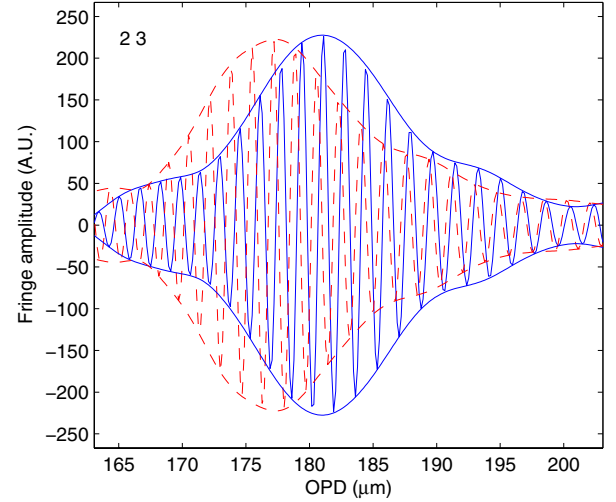
Fig. 1. Measured fringe packets in the Pioneer instrument, between inputs 2 and 3, for the two linear polarizations, and with birefringence uncorrected.
