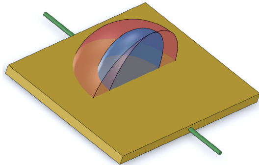
Fig. 5. In case 3, the optical axis is perpendicular to the vacuum-crystal interface, i.e. along the z axis. The two schematics are drawn as in case 1.
