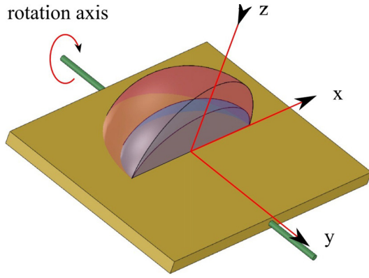
Fig. 3. In case 1, the optical axis is along the x direction. Left: a schematic of the birefringent plate, the rotation axis used to adjust the angle of incidence, and the two sheets of the index surface. Right: the geometry of wave vectors. The two circles and the ellipse are the intersections with the plane of incidence of the two sheets of the index surface and the unity sphere, all scaled by 2\pi/\lambda_0 , such that they are the locus of the tips of wave vectors \mathbf{k}' .
