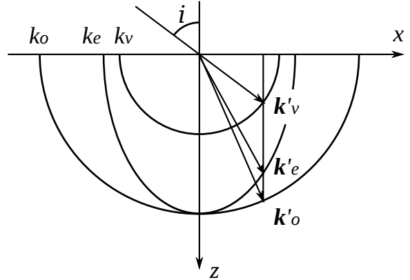
Fig. 5. In case 3, the optical axis is perpendicular to the vacuum-crystal interface, i.e. along the z axis. The two schematics are drawn as in case 1.
