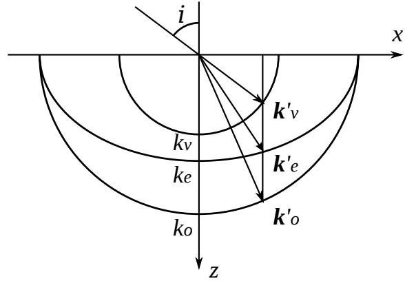
Fig. 3. In case 1, the optical axis is along the x direction. Left : a schematic of the birefringent plate, the rotation axis used to adjust the angle of incidence, and the two sheets of the index surface. Right : the geometry of wave vectors. The two circles and the ellipse are the intersections with the plane of incidence of the two sheets of the index surface and the unity sphere, all scaled by 2\pi/\lambda_0 , such that they are the locus of the tips of wave vectors k' .
