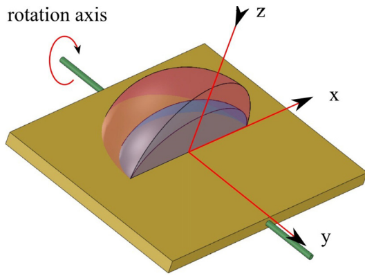
Fig. 3. In case 1, the optical axis is along the x direction. Left : a schematic of the birefringent plate, the rotation axis used to adjust the angle of incidence, and the two sheets of the index surface. Right : the geometry of wave vectors. The two circles and the ellipse are the intersections with the plane of incidence of the two sheets of the index surface and the unity sphere, all scaled by 2\pi/\lambda_0 , such that they are the locus of the tips of wave vectors k' .
