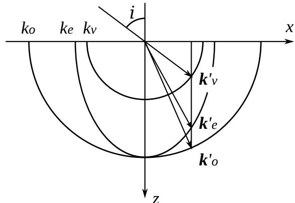
Fig. 5. In case 3, the optical axis is perpendicular to the vacuum-crystal interface, i.e. along the z axis. The two schematics are drawn as in case 1.
