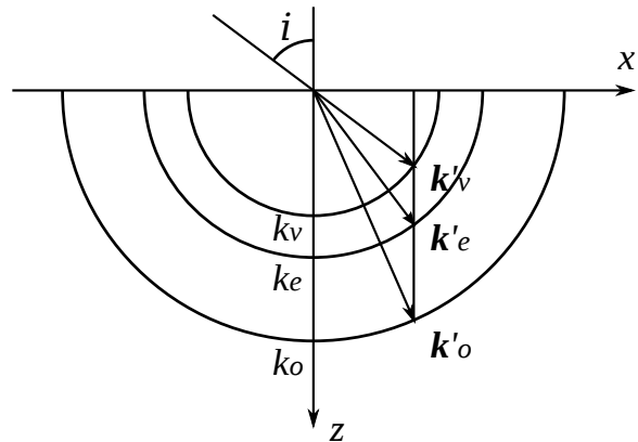
Fig. 4. In case 2, the optical axis is perpendicular to the plane of incidence. The two schematics are drawn as in case 1.
