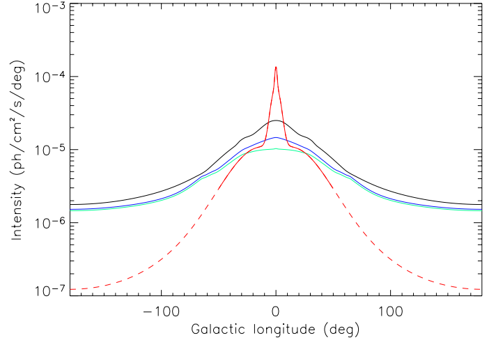
Fig. 7. Longitude profiles of the 511 keV emission of all nucleosynthesis positrons for each transport configuration. The colour coding is the same as in Fig. 6. The intensities correspond to the 511 keV emission from parapositronium and direct annihilation, for a positronium fraction of 0.97.
