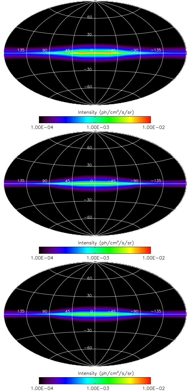
Fig. 3. Predicted 511 keV intensity distributions for the annihilation of ^{44}\text{Ti} positrons in each transport configuration. From top to bottom, the transport was assumed to be collisionless everywhere (case A, small diffusion coefficient), collisionless in the bulge and ballistic out of it (case B, inhomogeneous case), and ballistic everywhere (case C, large diffusion coefficient). The given intensities correspond to parapositronium annihilation only and were normalised to a positron injection rate of 10^{43} e^+ /s, with a positronium fraction of 0.95.
