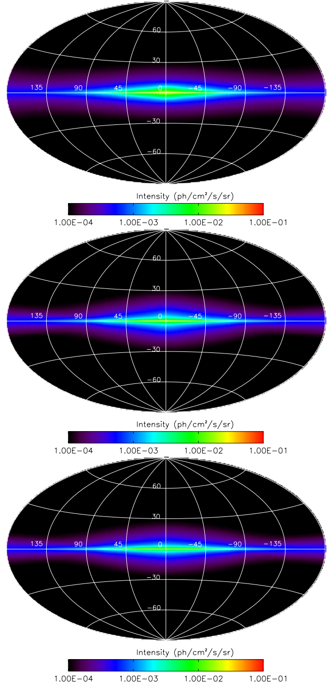
Fig. 5. Predicted 511 keV intensity distributions for the annihilation of all nucleosynthesis positrons, using the estimated mean positron injection rates. From top to bottom, the transport was assumed to be collisionless everywhere (case A, small diffusion coefficient), collisionless in the bulge and ballistic out of it (case B, inhomogeneous case), and ballistic everywhere (case C, large diffusion coefficient). The given intensities correspond to the 511 keV emission from parapositronium and direct annihilation, assuming a positronium fraction of 0.97.
