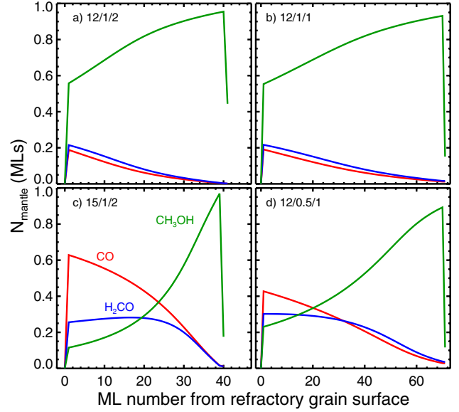
Fig. 9. Chemical composition of the mantle layers as a function of the monolayers at a time of 2 \times 10^5 years, for a density n_{\text{H}} = 10^5 \text{ cm}^{-3} , as in Cuppen et al. (2009) (see text): CO (red), formaldehyde (blue) and methanol (green). The four panels refer to the four cases of Fig. 4 of Cuppen et al. (2009) (see text): a) grain temperature 12 K, n(\text{H})/n(\text{CO}) = 1 and n_d = 2 \times 10^{12} n_h ; b) as a) but n_d = 1 \times 10^{12} n_h ; c) as a) but temperature 15 K; d) as b) but n(\text{H})/n(\text{CO}) = 0.5 .
