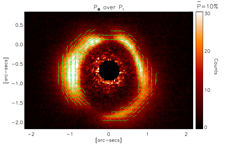
Fig. 9. Polarization angle ( P_\theta ) indicated by the green vectors, plotted over the P_I image. The length of the vectors is proportional to the local polarization degree ( P ). The vectors are plotted in regions of the image where the polarized intensity P_I is higher than three times the standard deviation ( \sigma_{P_I} ) of the sky background (see text).
