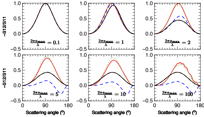
Fig. 10. Polarizability as a function of scattering angles for different mixtures of dust. The polarizability is the ratio of the -S12 over S11 elements of the Mueller matrix. In all cases, dust mixtures have power-law size distributions with a_{\min} = 0.03 \mu\text{m} and a slope of -3.5 . Six cases with increasing values of a_{\max} are considered. The red curves show the polarizability for Mathis & Whiffen (1989) grains (a mix of astrosilicates and amorphous carbon and 80% porosity). The dotted green curves are for pure astronomical silicates with 80% porosity (Draine 2003). The blue dashed curves are for compact astronomical silicates without porosity (Draine 2003). The black curve is for a mixture of compact no porosity grains made of 100% amorphous carbon. All models with porosity have a high polarizability near 90 degrees scattering angles. Models with compact particles show lower maximum polarizations.
