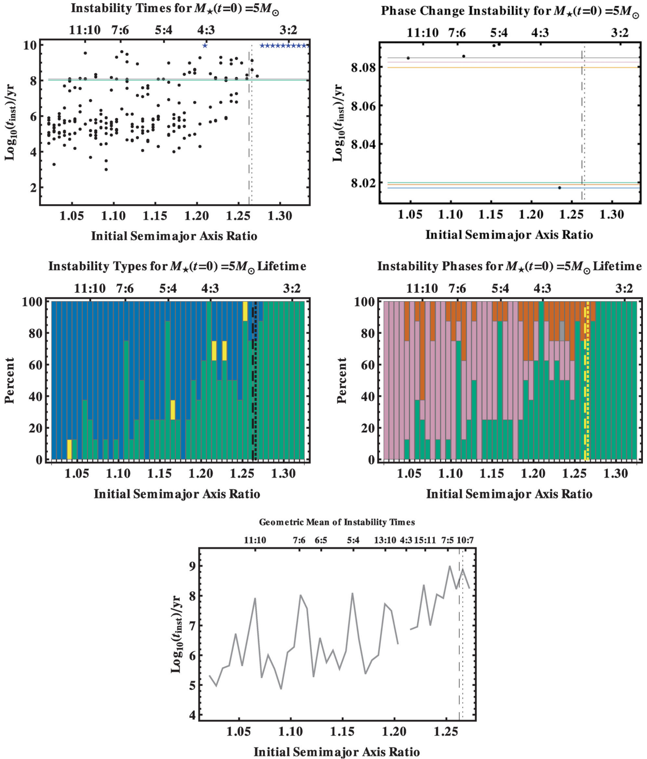
Figure 15. Here, M_1 = M_2 = 1 M_\oplus . The plots are of the same format as in Figs 9–13. Instability during the WD phase occurs almost exclusively at initial separations inside the MS and WD Hill stability limits. MS Hill unstable systems protected by mean-motion commensurabilities, many of which feature resonant behaviour, allow for survival during the MS before becoming unstable on the WD phase.
