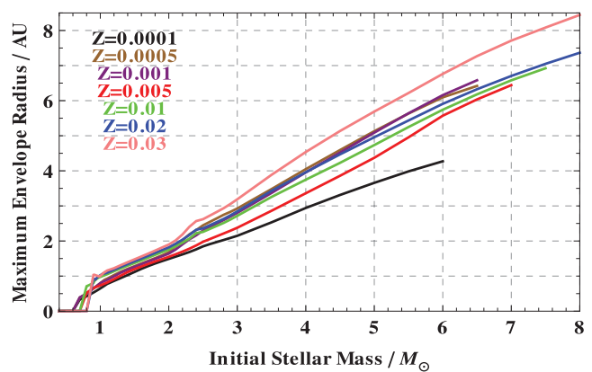
Figure 2. Maximum stellar radius as a function of progenitor mass and metallicity. Colours denote different metallicities; the blue curve ( Z = 0.02 ) represents Solar metallicity. Curves end when supernovae occur. This plot demonstrates a rule of thumb: generally, the number of au at the maximum radius is approximately equal to the number of initial M_{\odot} .
