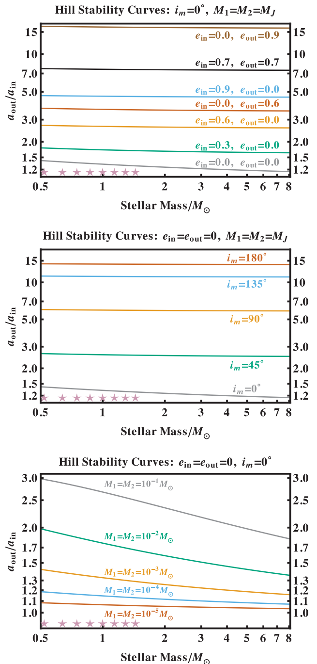
Figure 4. Critical Hill semimajor axis ratios as a function of stellar mass for different eccentricities (upper panel), different mutual inclinations (middle panel) and different planetary masses (bottom panel). The purple stars on the bottom of each plot, from right to left, represent the eventual WD mass (in brackets in the following) for MS progenitor masses of 8 M_\odot [1.44 M_\odot ], 7 M_\odot [1.29 M_\odot ], 6 M_\odot [1.14 M_\odot ], 5 M_\odot [1.00 M_\odot ], 4 M_\odot [0.87 M_\odot ], 3 M_\odot [0.75 M_\odot ], 2 M_\odot [0.64 M_\odot ] and 1 M_\odot [0.52 M_\odot ]. The figure illustrates that the Hill radius is sensitively dependent on e_{out} , e_{in} , i_m , M_1 and M_2 , but weakly dependent on M_\star . For Jovian and terrestrial-mass planets, stellar mass-loss can change the Hill stability limit by at most a few tenths in a_{out}/a_{in} .
