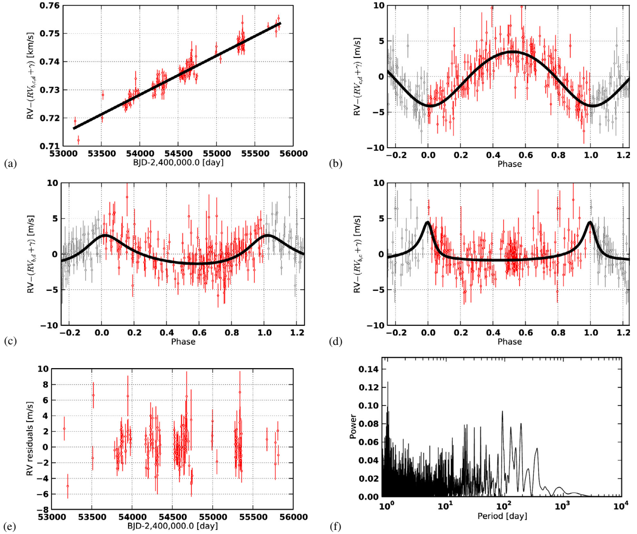
Fig. 7. Decomposition of our nominal three planet + 1 drift model for Gl 667C. Panel a) shows the contribution of the long-term drift with the three Keplerian contributions removed. Panels b), c), and d) show respectively radial velocity curves for Keplerians P_b = 7.2 d, P_c = 28.1 d, and P_d = 106.4 d. Residuals of this solution are shown in panel e) and their periodogram in panel f).
