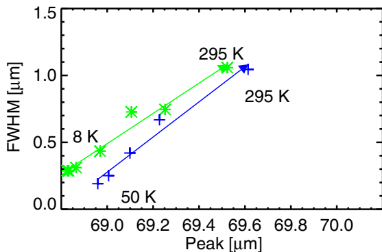
Fig. 2. Effect of temperature on the peak position and FWHM of the 69\ \mu\text{m} band. The blue crosses are based on optical constants from Suto et al. (2006) using the distribution of hollow spheres by Min et al. (2003) with a grain size of 0.1\ \mu\text{m} . The green asterisks represent mass absorption coefficients from Koike et al. (2006). Both datasets were taken on pure forsterite.
