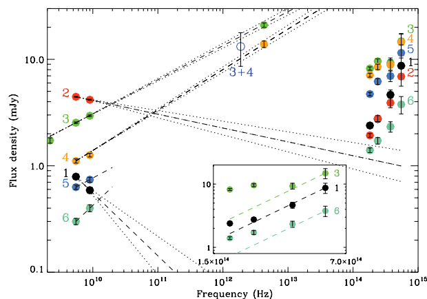
Figure 3. Evolution of the radio to OIR broad-band spectra during the soft to hard state transition. The numbers (and associated colours) refer to the epochs highlighted in Fig. 2. The dashed lines correspond to the extrapolation of the radio spectra (with dotted lines to indicate the 1\sigma error when it is not too large). For the spectra # 3 and 4 (which include the Herschel observations), we use the measured radio to far-IR spectral index. The open blue circle is the 160 \mu\text{m} detection combining the two Herschel observations. Inset: zoom of the OIR spectra # 1, 3 and 6. The dashed lines correspond to an extrapolation of the V-band with an index of +1.5 (possible for an irradiated disc; Hynes 2005) for a selection of the spectra.
