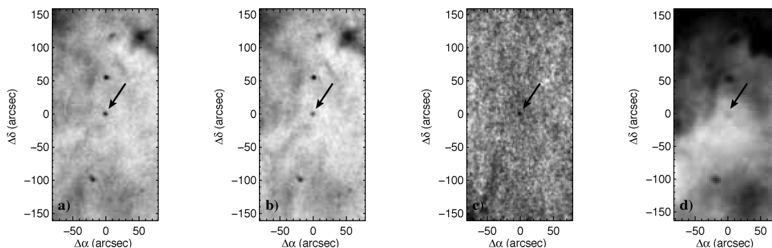
Figure 1. Herschel maps of GX 339–4: at 70 \mu\text{m} on February 25 (a) and March 6 (b), their difference in (c), and at 160 \mu\text{m} (two epochs) in (d).
