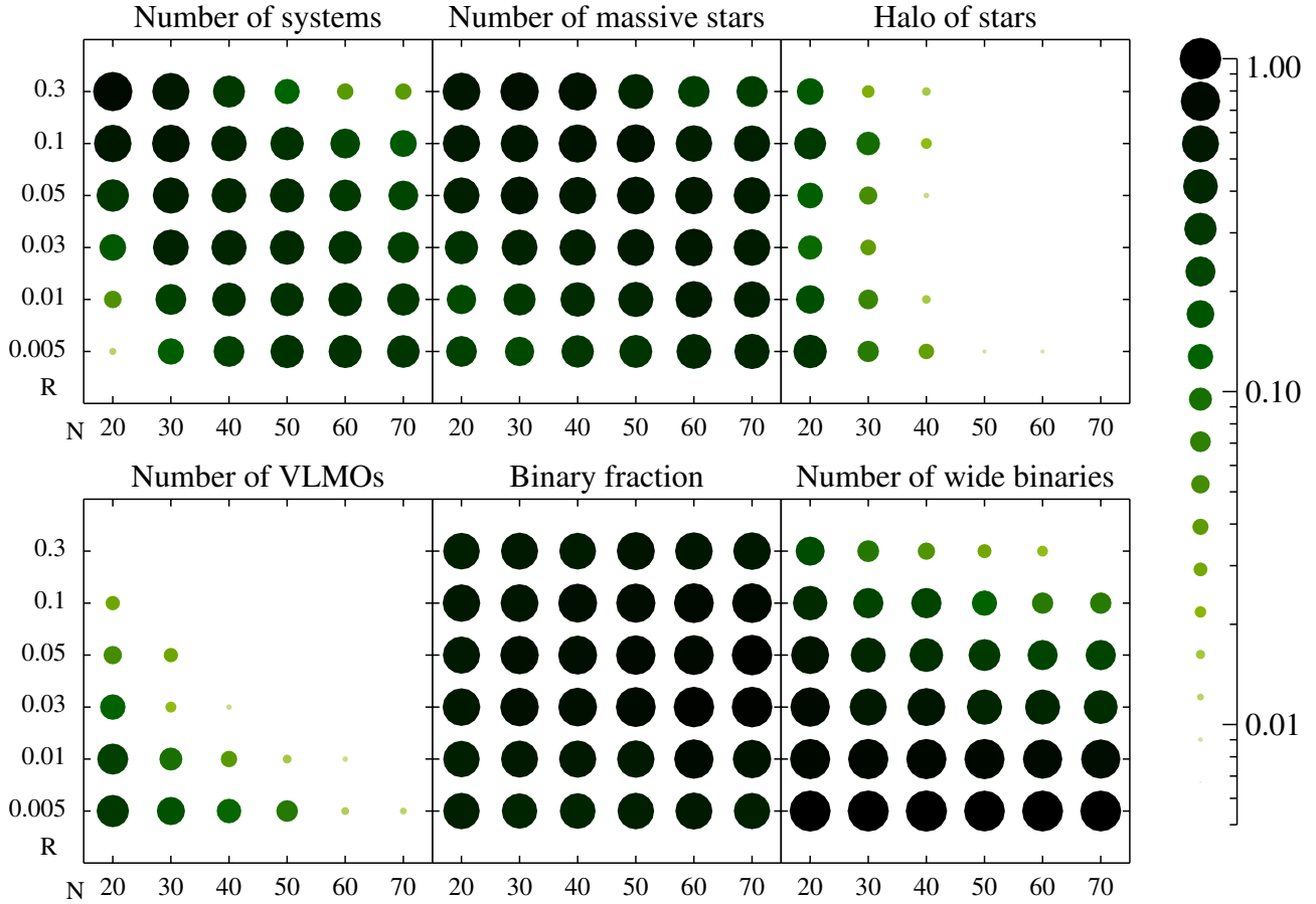
Fig. 4. Summary for all tested configurations for model A with a virial ratio Q_i = 0.5 . For convenience the value for the quality measure, a_i(t_{i,m}) is also indicated by the dot size, with a logarithmic scale. For each criterion, the colour (and size) of the circles indicates the probability for the simulations to reproduce the observations. The results obtained with a different virial ratio Q_i are very similar.
