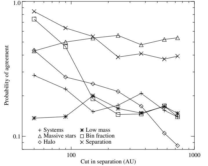
Fig. 8. Evolution of the agreement probability for the different criteria, when setting a maximum value for the binary separation, varying from 50 to 730 AU, and adopting a flat mass-ratio distribution (model C). The results are given for \{Q_i = 0.5, N_{sys} = 20, R_{pl} = 0.1 pc \} .
