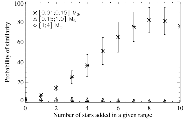
Fig. 1. KS test evaluating the similarity of the \eta Cha mass distribution with the log-normal system IMF. The comparison is done considering three mass ranges, in order to assess which parts of the distribution are alike. We progressively added ten stars in \eta Cha data set, selected randomly from the IMF within the mass range [0.01;0.15] M_{\odot} . Each time a star is added we compute a probability from the KS test. This process is repeated for the mass ranges [0.15;1] M_{\odot} and [1;4] M_{\odot} .
