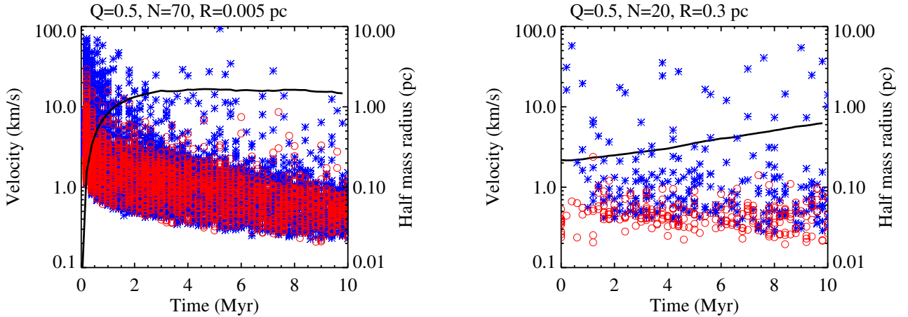
Fig. 2. Left panel: velocity of ejected members at the time of ejection (blue asterisks for single objects, and red open circles for binaries) for a dense configuration from model A, with N_{\text{sys}} = 70 , Q_i = 0.5 , and R_{\text{pl}} = 0.005 pc. Right panel: sparse configuration with N_{\text{sys}} = 20 , Q_i = 0.5 , and R_{\text{pl}} = 0.3 pc. The half mass radius evolution is superimposed (thick line), as a footprint of the stellar density for both cases.
