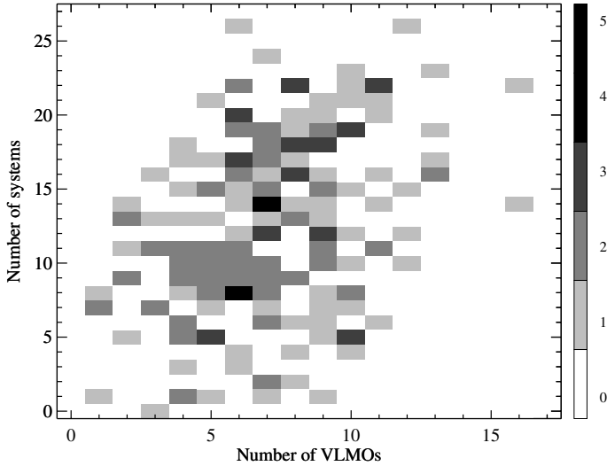
Fig. 6. Correlation map between the number of systems ( N_1 ) and the number of VLMOs ( N_3 ) at t = 7 Myr for N_{\text{sys}} = 30 , R_{\text{pl}} = 0.05 pc and Q_i = 0.5 (model A).
