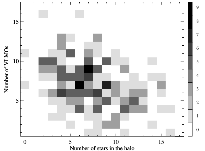
Fig. 5. Correlation map between the number of VLMOs ( N_3 ) and the number of solar-type stars in the halo ( N_4 ) at t = 7 Myr for N_{\text{sys}} = 30 , R_{\text{PI}} = 0.05 pc and Q_i = 0.5 (model A).
