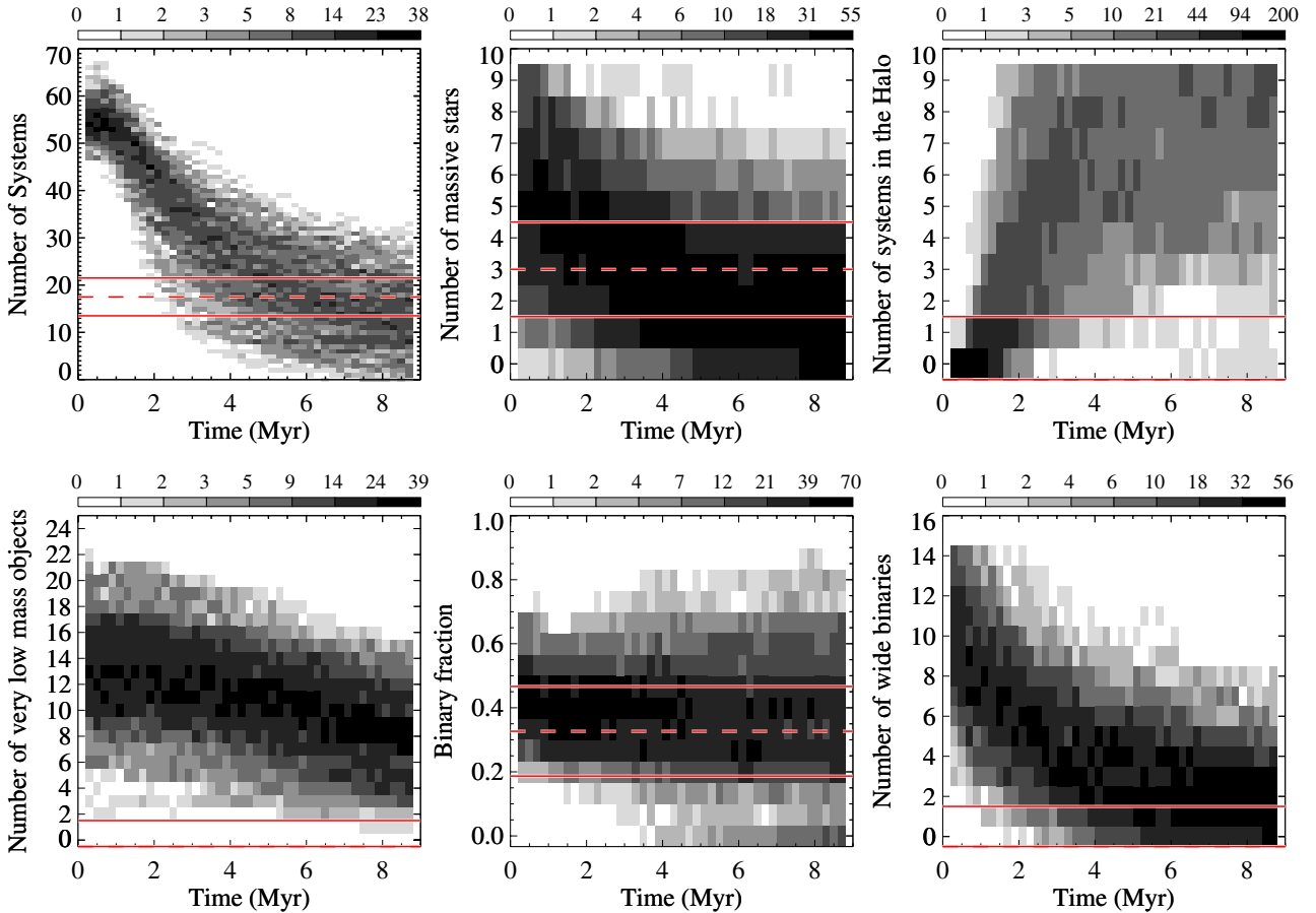
Fig. 3. 3D histograms showing the evolution of a) the number of systems in the core N_1 ; b) the number of massive stars in the core N_2 ; c) the number of systems in the halo N_3 ; d) the number of VLMOs inside a 2.6 pc radius N_4 ; e) the binary fraction in the core N_5 ; and f) the number of wide (separation greater than 50 AU) binaries N_6 as a function of time for model A and for the initial configuration \{N_{\text{sys}} = 40, R_{\text{pl}} = 0.05 \text{ pc}, Q_i = 0.5\} . The histogram density corresponds to the number of simulations (out of 200) that fall in a given bin. The dashed and solid red lines correspond to the observed value and the acceptable range respectively.
