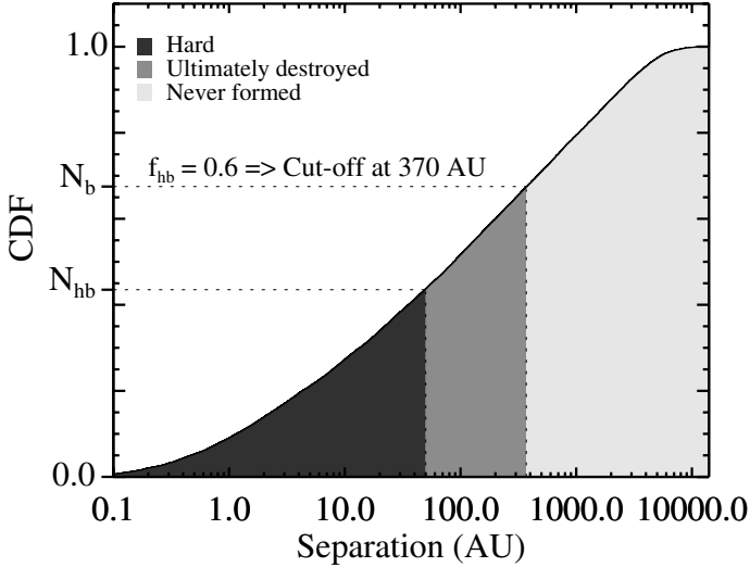
Fig. 7. Cumulative separation distribution function (solid line) obtained from the Kroupa period distribution (see section 3). This highlights how the distribution is truncated in Model C in the case of f_b = 0.8 . Expression 1 yields f_{hb} = 0.6 , which imposes to truncate the separation distribution to 370 AU, so that N_{hb} = 0.6 \times N_b .
