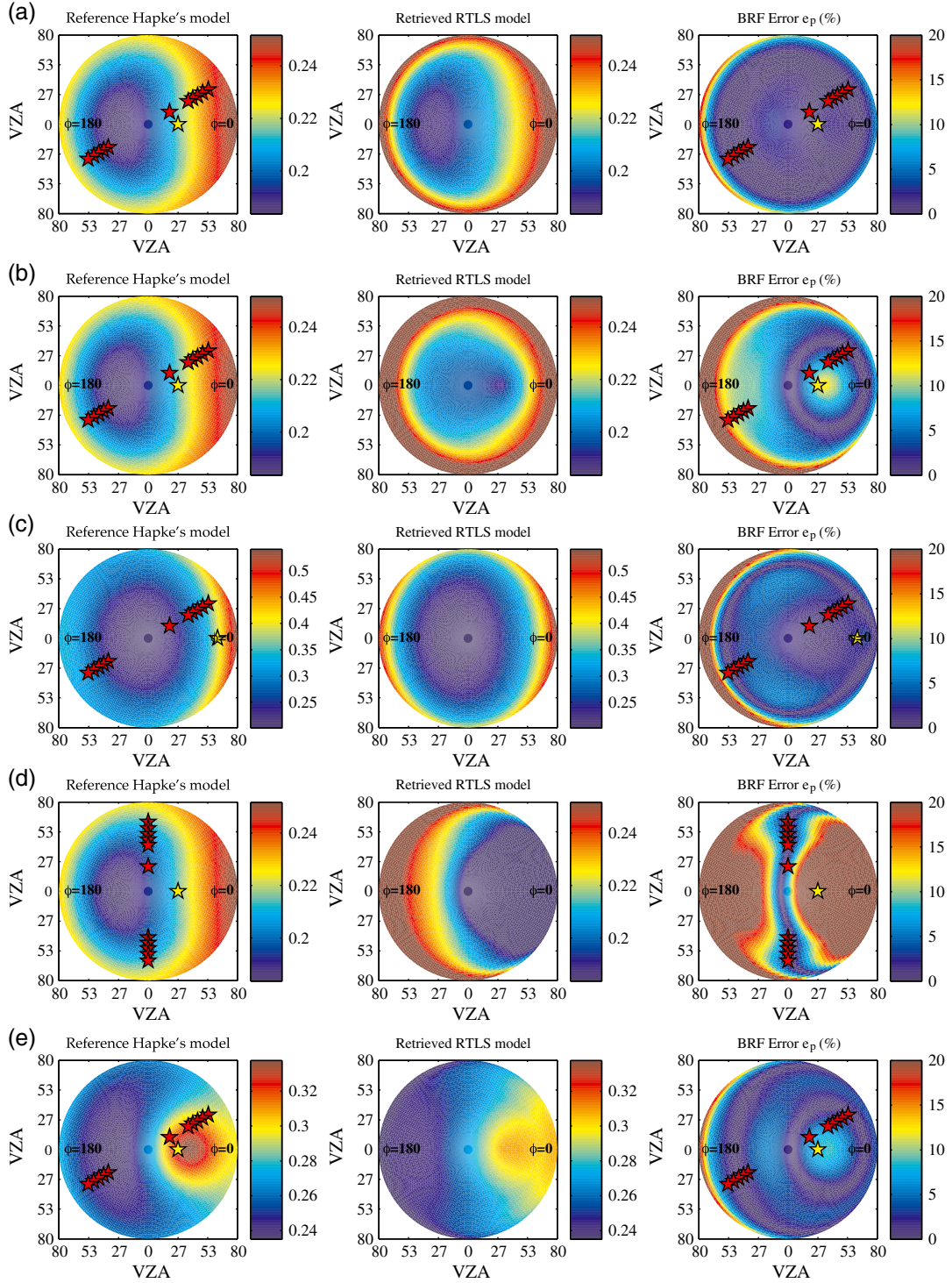
Figure 7. From top to bottom, same as Figure 6 when (a) \tau_0 = 0.5 , (b) \tau_0 = 2 , (c) \tau_0 = 0.5 and \theta_0 = 70^\circ , (d) \tau_0 = 0.1 and \varphi_1, \varphi_2 = \{90^\circ, 90^\circ\} , and (e) \tau_0 = 0.5 and surface made of material Red rock-1.
