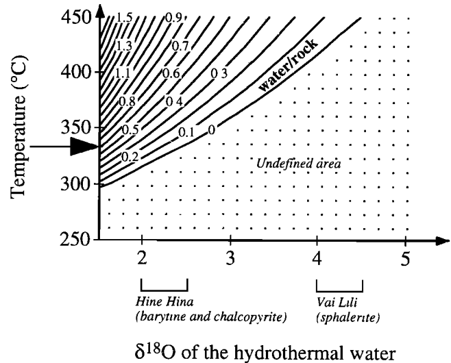
Figure 13. Domain of water-rock ratios defined by the temperature and oxygen isotope composition of hydrothermal fluids. The \delta^{18}\text{O} values (‰ SMOW) of water inclusions that have been measured in the mineralizations from the Hine Hina and Vai Lili fields are reported.
