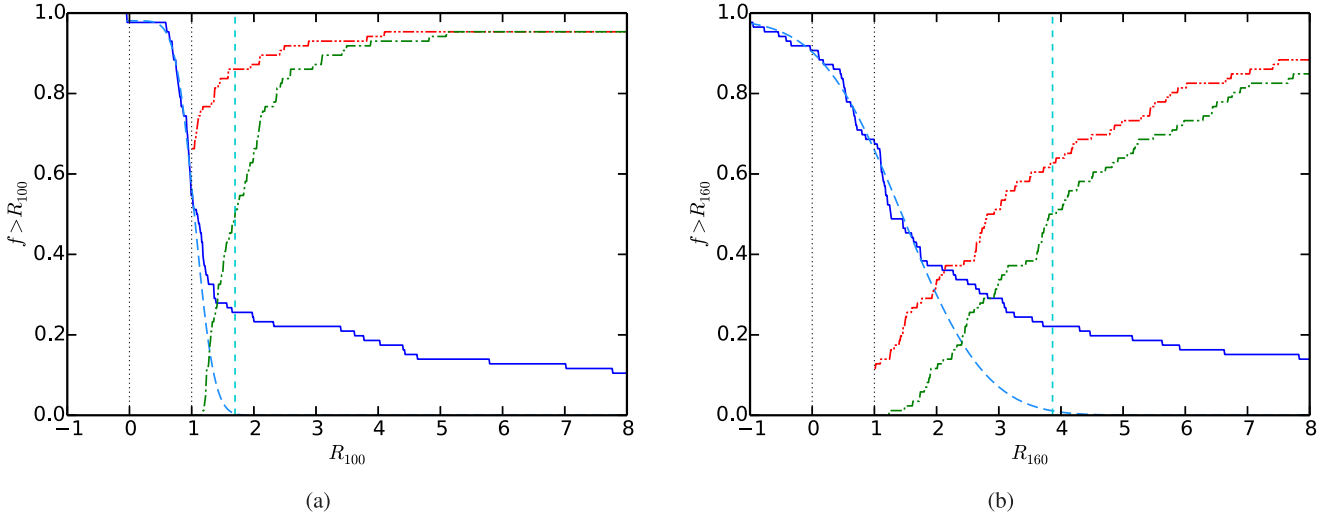
Figure 2. (a) Solid line: the cumulative distribution function (CDF) of R_{100} . Double-dot-dashed line: fraction of stars with P_{100} > \frac{3 \times \epsilon_{100}}{R_{100}} as a function of R_{100} . Dash-dotted line: fraction of stars for which disc emission could have been detected at this level (i.e. F_{100}^{\text{disc}} > \frac{3 \times \epsilon_{100}}{R_{100}} ) as a function of R_{100} . F_{100}^{\text{disc}} is the measured 100 \mu\text{m} disc flux. Long-dash curve: lognormal fit to the R_{100} < 1 values. The R_{100} CDF departs from the fit for R_{100} = 1.05 , while the R_{160} CDF departs from the fit for R_{160} = 1.81 . The vertical short-dash line indicates the 3\sigma R_{100}^{\text{det}} = 1.70 median detection limit. The vertical dotted lines indicate the R_{100} = 0 and =1 values. (b) Same as (a) for wavelength 160 \mu\text{m} where the 3\text{-}\sigma median detection limit is R_{160}^{\text{det}} = 3.87 .
