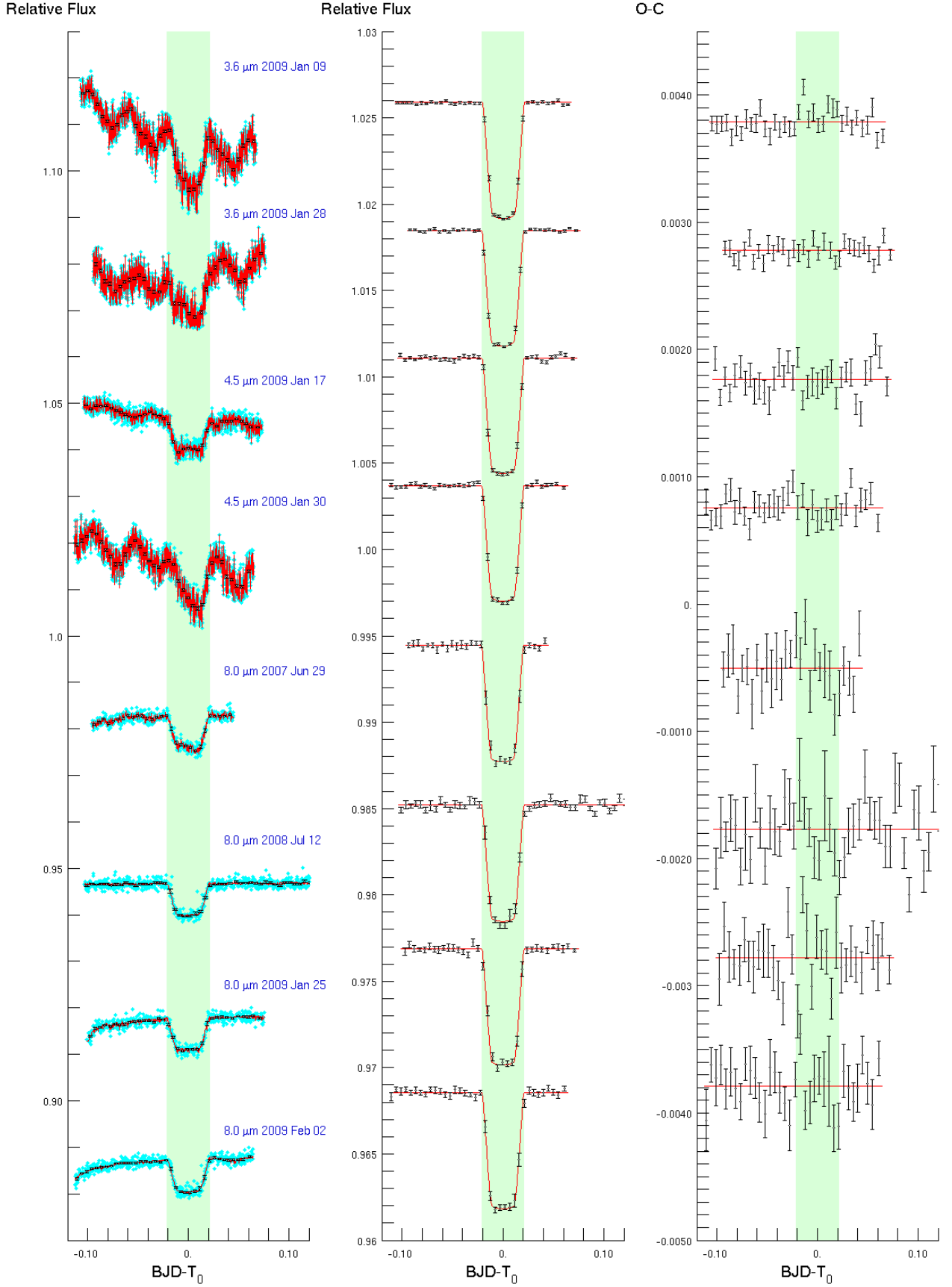
Fig. 5. Eight transit light curves of GJ 436b. The two upper panels are the data at 3.6\ \mu\text{m} from 2009 January 9 and 28. The following two were taken at 4.5\ \mu\text{m} on 2009 January 17 and 30. The lower four were obtained at 8\ \mu\text{m} on 2007 June 29, 2008 July 12, 2009 January 25 and February 2. The left plot displays the raw binned and unbinned data, the middle one the binned data corrected for instrumental systematics, and the right one the binned residuals. Measurements are binned per interval of 7 min. The light curves are shifted along the y -axis for the sake of clarity. The shaded green areas show the transit events.
