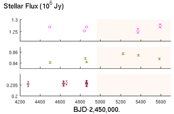
Fig. 4. Stellar flux evolution in the 3.6 (top), 4.5 (middle), and 8.0\ \mu\text{m} (bottom) IRAC channels. The stellar flux slightly fluctuates with time in the 3.6 and 4.5\ \mu\text{m} bandpasses, and is constant at 8.0\ \mu\text{m} . A different inter-pixel map is used for the Warm mission data. The Warm Spitzer phase is shaded in pale pink for clarity. The flux modulation is probably due to the uncorrected intra-pixel effect and to the calibration uncertainties, which are not displayed here for clarity.
