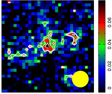
Fig. 15. PACS blue channel ( 70\ \mu\text{m} ) combined map of the undetected Class II objects. The map is 30'' in size along each axis. The beam size is represented by the yellow circle in the bottom, right-hand corner and the black star marks the peak position in the map. Contour levels are plotted at 4 , 5 and 6\sigma . The scale bar shows the intensity of the map in \text{mJy/pixel} .
