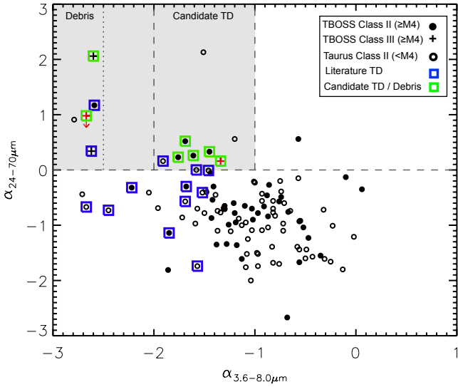
Fig. 13. Spectral index plot showing the Taurus Class II and Class III members with mid-IR and far-IR excess. The spectral indices; \alpha_{3.6-8.0\mu\text{m}} and \alpha_{24-70\mu\text{m}} are used to identify candidate targets with transition disks (TDs; points bounded by the horizontal and vertical dashed lines) and debris disks (points bounded by the horizontal dashed and vertical dotted lines). Targets identified in the literature with TDs, and the candidate TD/debris disks reported here, are enclosed by blue and green squares respectively. J04295422+1754041 (red cross) was unobserved with IRAC and MIPS, and the spectral indices are calculated from the WISE 3.4 \mu\text{m} and 12 \mu\text{m} flux densities, and the WISE 22 \mu\text{m} and PACS 70 \mu\text{m} flux densities. XEST 08-033 (red cross with downward arrow) was only detected with PACS at 160 \mu\text{m} , and the 24–70 spectral index shown is calculated from the 70 \mu\text{m} upper limit.
