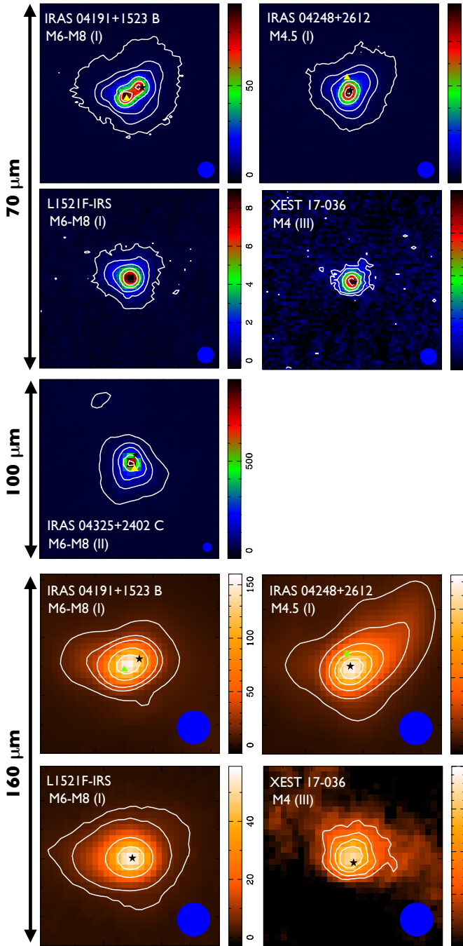
Fig. 5. PACS blue channel (70 \mu\text{m} and 100 \mu\text{m} ) and red channel (160 \mu\text{m} ) maps of the five spatially extended TBOSS targets. Target name, spectral type and evolutionary class are labeled in the top, left-hand corner of each map. The 70 \mu\text{m} and 160 \mu\text{m} maps are 60'' in size along each axis, and the 100 \mu\text{m} maps are 120'' in size along each axis. Beam sizes are represented by the blue circles in the bottom, right-hand corner of each map. The scale bar shows the intensity of each map in units of mJy/pixel. 2MASS coordinates of the TBOSS targets are represented by the black stars. For binary systems, the position of the companion star are indicated with yellow triangles in the 70 \mu\text{m} and 100 \mu\text{m} maps, and by green triangles in the 160 \mu\text{m} maps. Contours levels begin at 3\sigma in all maps and extend up to 500\sigma , 400\sigma , 150\sigma , 40\sigma and 300\sigma in the blue channel maps of IRAS 04191+1523 B, IRAS 04248+2612, L1521F-IRS, XEST 17-036 and IRAS 04325+2402 C respectively, and up to 50\sigma , 60\sigma , 70\sigma and 10\sigma in the red channel maps of IRAS 04191+1523 B, IRAS 04248+2612, L1521F-IRS and XEST 17-036 respectively.
