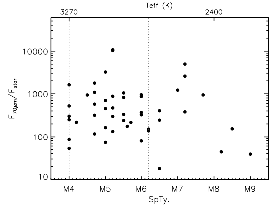
Fig. 9. 70\ \mu\text{m} disk excess fraction shown as a function of spectral type for the detected Class II objects within the TBOSS sample.
