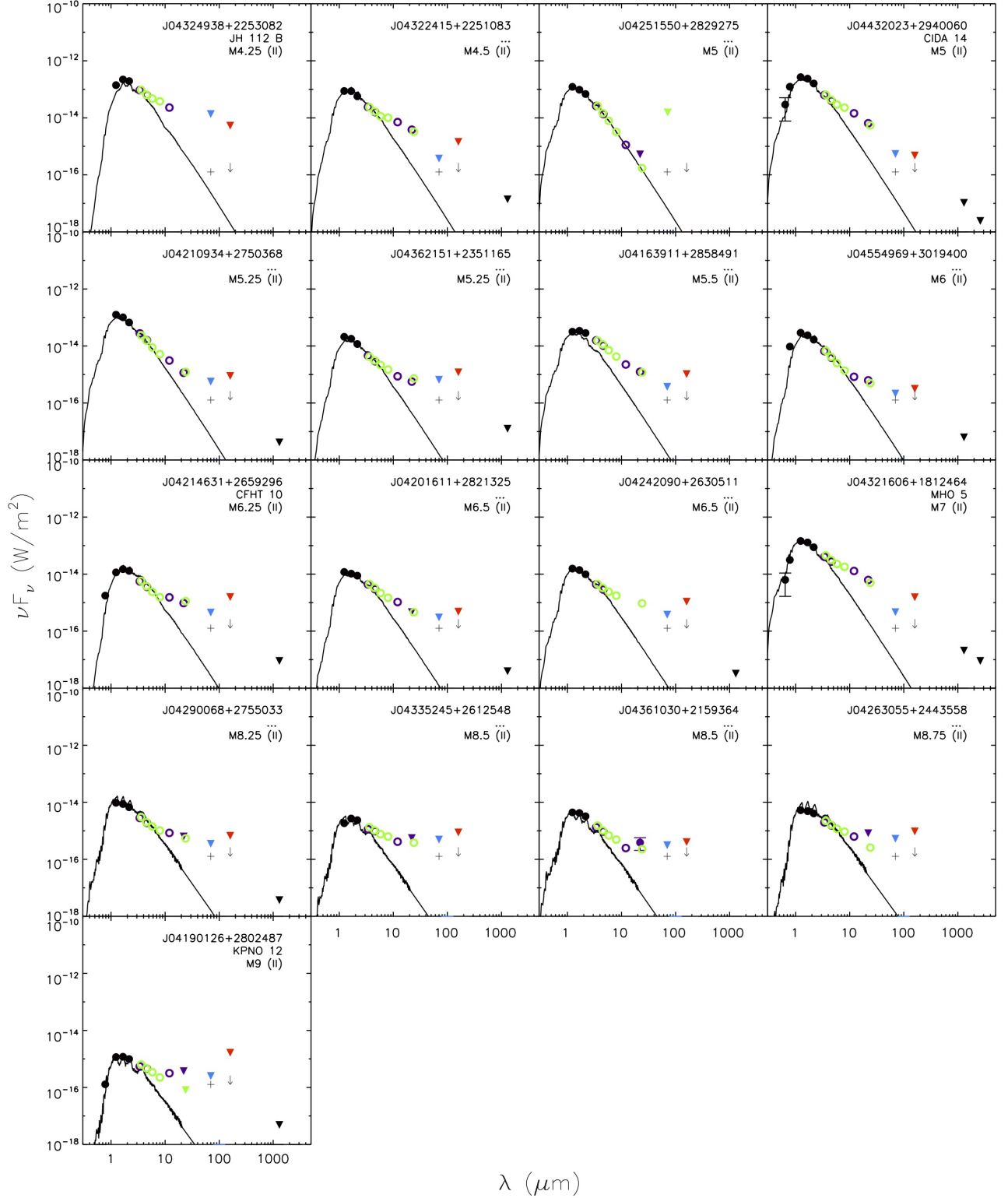
Fig. D.4. SEDs of the undetected Class II objects with spectral types spanning M4.25-M9. The target name, spectral type, and spectral class are labeled in each SED. The observed broadband photometry is compiled from optical ( R_C , I_C ), and near-IR (2MASS; JHK_S ) wavelengths (black points), the mid-IR (IRAC and WISE ; green and purple open circles respectively), the far-IR (MIPS, PACS blue and red channels; green open circles, blue and red points respectively) and submm-mm wavelengths (black points). 3\sigma upper limits are represented by the downwards triangles. The best-fit atmospheric model is displayed for each target. The gray cross shows level of the artificial detection generated from combined Class II ( 70\ \mu\text{m} ) upper limit maps, and similarly the gray downward arrow shows the 160\ \mu\text{m} upper limit from the combined maps.
