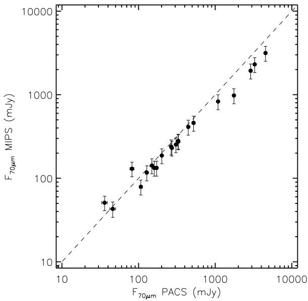
Fig. 3. Relation of PACS 70 \mu\text{m} and corresponding MIPS 70 \mu\text{m} flux densities (Rebull et al. 2010) for the TBOSS targets detected with both instruments. Non-linearity of the MIPS detector at \sim 1 Jy is the likely cause of the 25–40% flux discrepancy seen for the targets > 1 Jy, measured with PACS.
