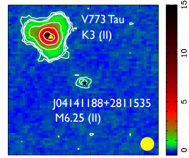
Fig. 6. PACS blue channel (70 \mu\text{m} ) map of the faintly detected brown dwarf J04141188+2811535 (black star). The earlier type companion V773 Tau (yellow triangle) is also seen within the map and is spatially extended. Target name, spectral type and evolutionary class for each component of the system are indicated on the map. The map is 60'' in size along each axis. The beam size is represented by the yellow circle in the bottom, right-hand corner. Contour levels are plotted at 3 , 5 , 7 , 20 , 50 and 100\sigma . The scale bar shows the intensity of the map in mJy/pixel.
