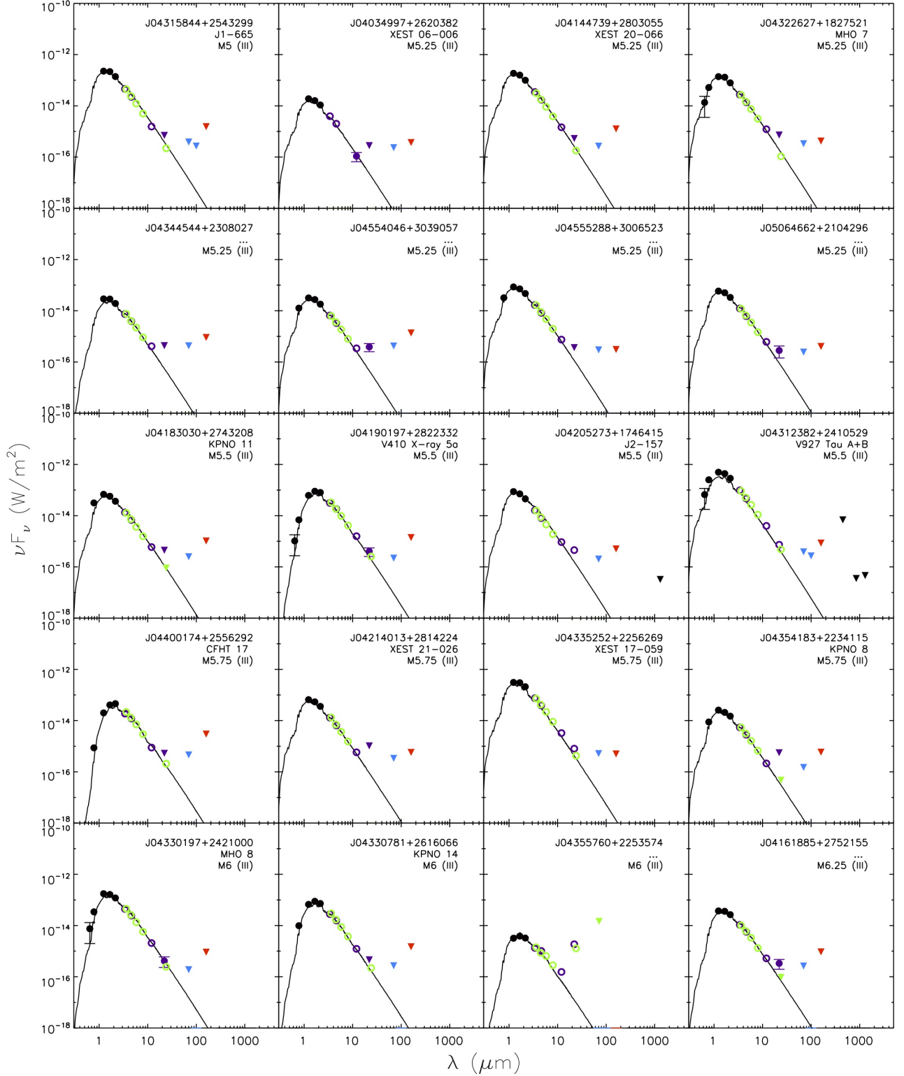
Fig. E.2. SEDs of the undetected Class III objects with spectral types spanning M5-M6.25. The target name, spectral type, and spectral class are labeled in each SED. The observed broadband photometry is compiled from optical ( R_C , I_C ), and near-IR (2MASS; JHK_S ) wavelengths (black points), the mid-IR (IRAC and WISE; green and purple open circles respectively), the far-IR (MIPS, PACS blue and red channels; green open circles, blue and red points respectively) and submm-mm wavelengths (black points). 3\sigma upper limits are represented by the downwards triangles. The best-fit atmospheric model is displayed for each target.
