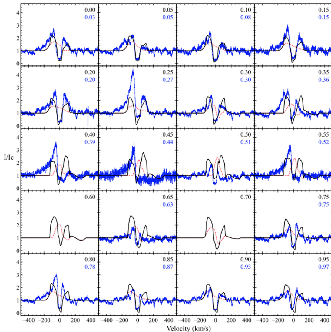
Figure 18. Best-fitting models for H \beta profiles out of occultation, with \dot{M}_{\text{wind}}/\dot{M}_{\text{acc}} = 0.1 , T_{\text{mag}} = 8900 K and T_{\text{wind}} = 8000 K. The magnetosphere contribution is shown by the red dotted line, and the magnetosphere-plus-wind profile is shown by the black solid line.
