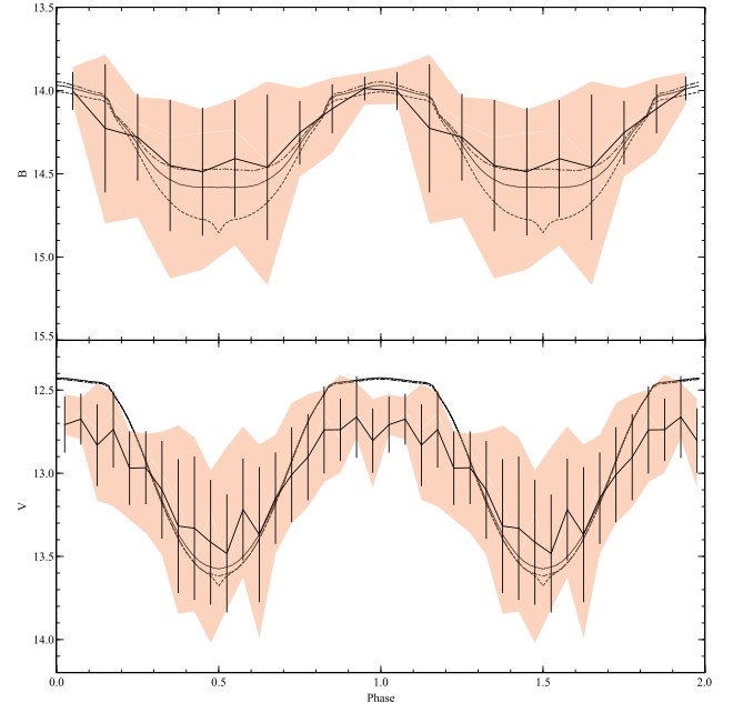
Figure A5. Comparisons between observations and models where \theta = 20^\circ and h_{\max}/r_o = 0.33 .
