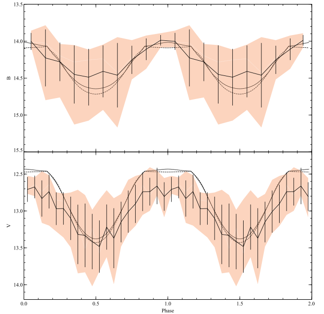
Figure 9. Best fits to average photometric data from B99, B03, B07, and ASAS. The solid line shows the mean brightness at each phase with the standard deviation given by the error bars. We found observations were best fitted by models with \dot{M}_{\text{acc}} = 5 \times 10^{-9} M_\odot \text{ yr}^{-1} , r_i = 5.2R_* , and h_{\max}/r_o = 0.31 . The dashed line shows \theta = 10^\circ and the dotted line shows \theta = 20^\circ .
