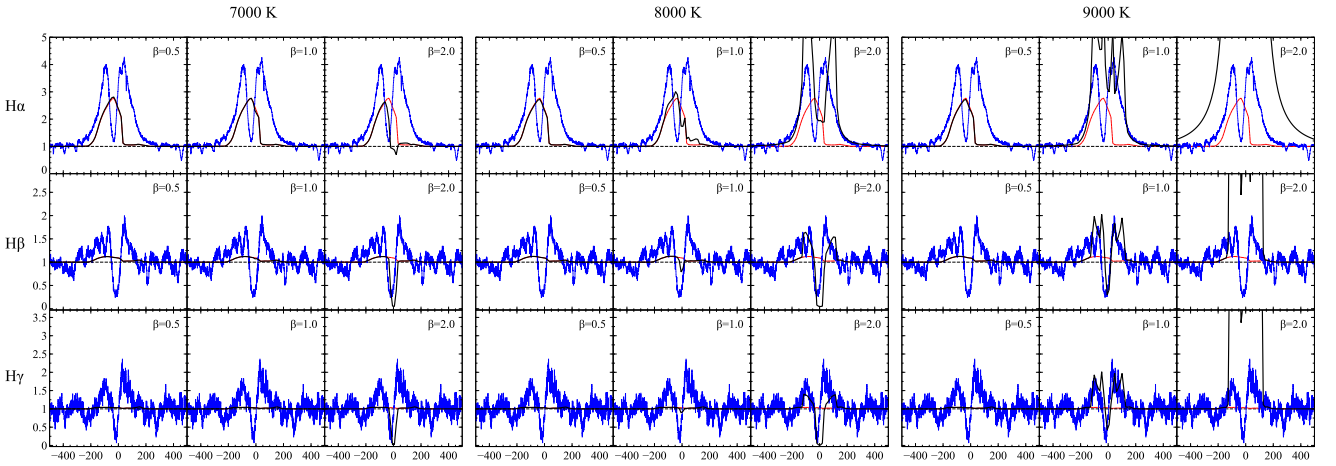
Figure 13. Magnetosphere with wind models for H \alpha , H \beta , and H \gamma at \varphi = 0.0 , with \theta = 10^\circ . Wind temperature and the acceleration parameter are varied with T_{\text{wind}} = 7000, 8000 , and 9000 K, and \beta = 0.5, 1.0 , and 2.0 . Our line profiles are shown in black, observed profiles are shown in blue, and the magnetosphere contribution is given in red.
