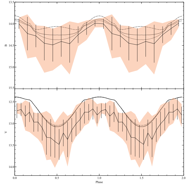
Figure A6. Comparisons between observations and models where \theta = 30^\circ and h_{\max}/r_o = 0.29 .
