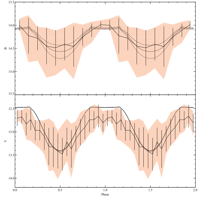
Figure A1. Comparisons between observations and models where \theta = 10^\circ and h_{\text{max}}/r_o = 0.31 .
