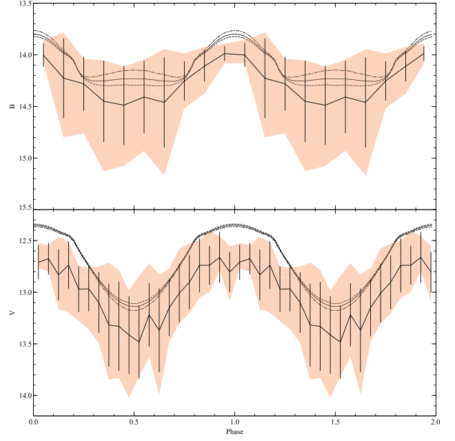
Figure A9. Comparisons between observations and models where \theta = 40^\circ and h_{\max}/r_o = 0.30 .
