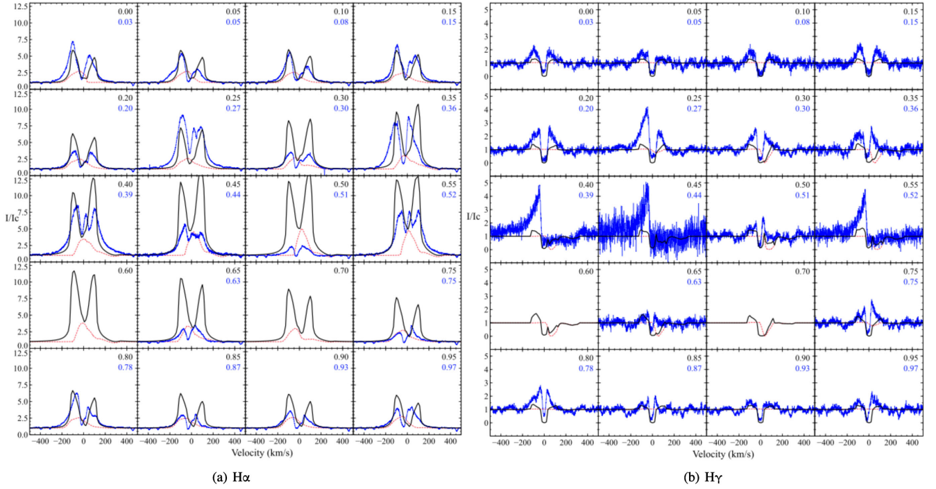
Figure B2. Comparison of models with observed line profiles for \dot{M}_{\text{wind}}/\dot{M}_{\text{acc}} = 0.09 , T_{\text{mag}} = 8500 K and T_{\text{wind}} = 8000 K for H \alpha and H \gamma . The magnetosphere contribution is shown by the red dotted line.
