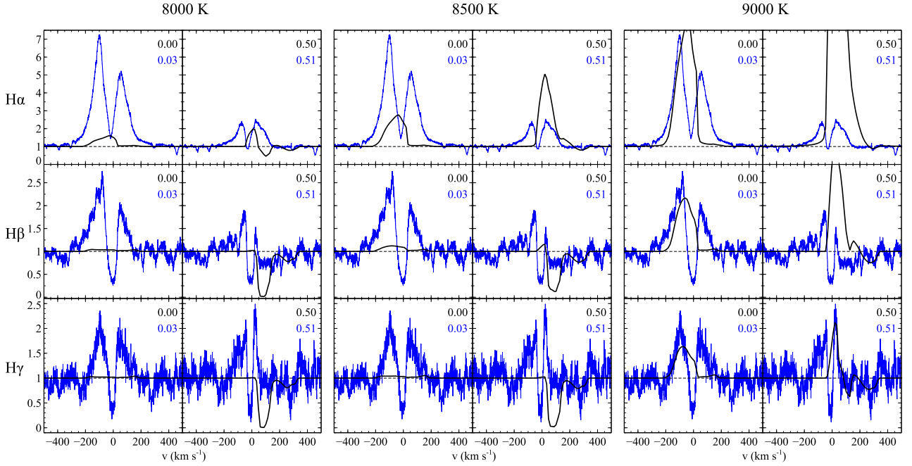
Figure 12. Magnetosphere-only models for H \alpha , H \beta , and H \gamma at a range of temperatures at \varphi = 0.0 and \varphi = 0.5 . Observed profiles are given in blue, and the continuum level is shown by the dashed line.
