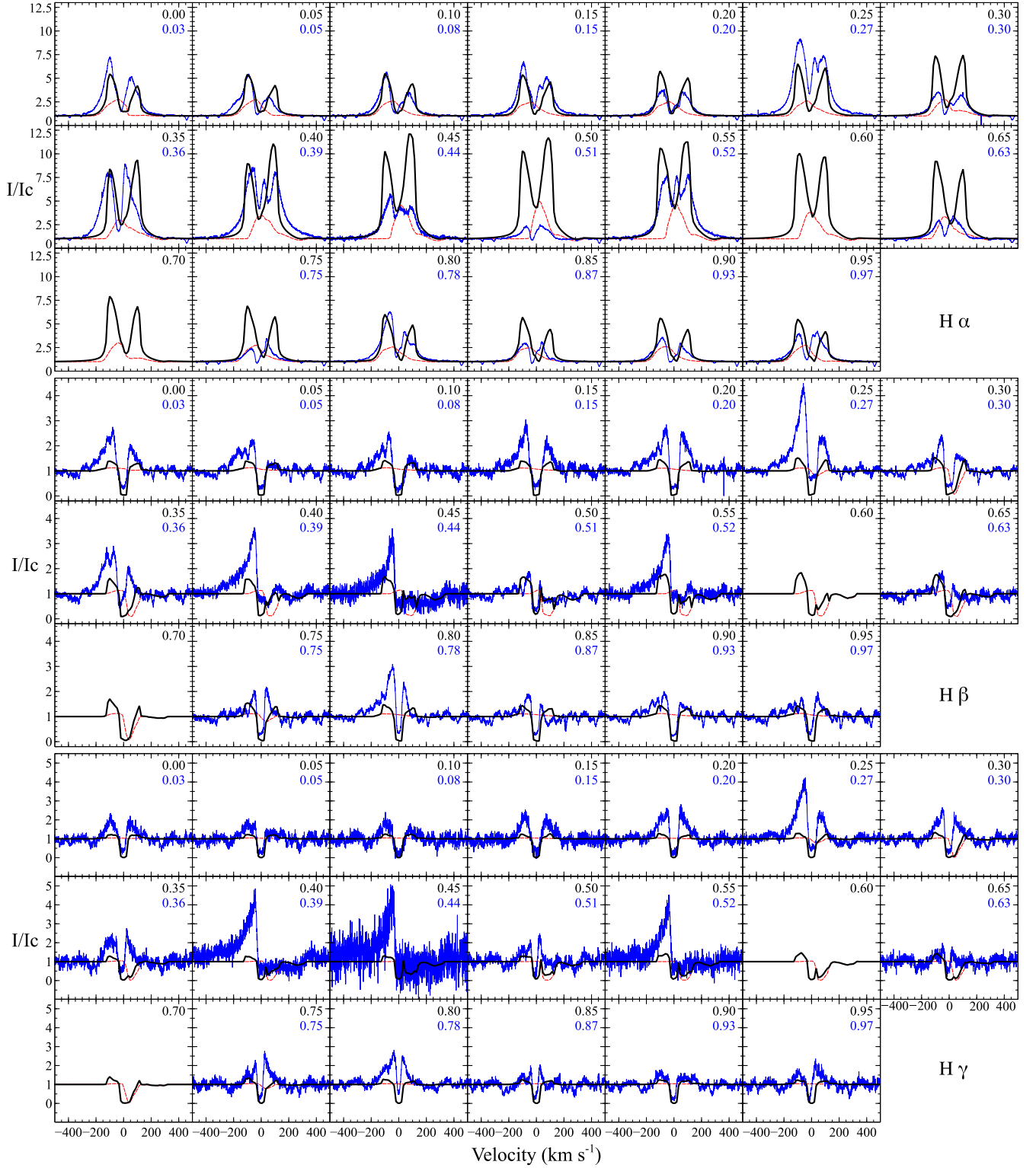
Figure B3. Observed H\alpha , H\beta , and H\gamma profiles compared with models where \dot{M}_{\text{wind}}/\dot{M}_{\text{acc}} = 0.10 , T_{\text{mag}} = 8500 K and T_{\text{wind}} = 7900 K. The magnetosphere contribution is shown by the red dotted line.
