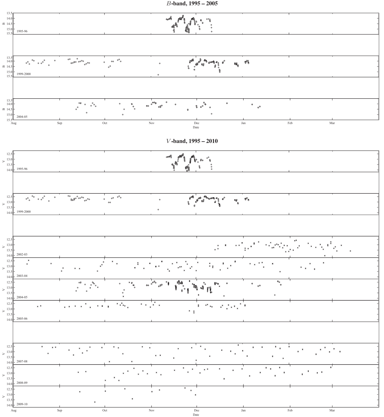
Figure 1. All B - and V -band photometry for AA Tau from 1995 to 2010 (B99; B03; B07; ASAS). Data from Bouvier et al. is shown with circles and ASAS data with crosses. Short-term variations in photometric behaviour are clear, for instance in 1999–2000 where the system shows little variation initially but exhibits deep luminosity dips after just a few weeks. A similar ‘quiet’ period is evident towards the end of 2005.
