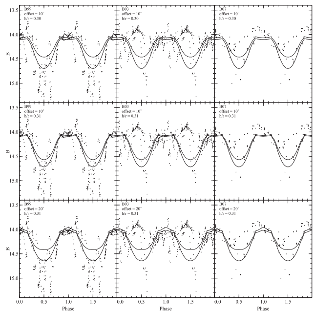
Figure 7. Fits to B -band photometry. The data source and parameter set are labelled on the top left of each plot. Dashed lines show the largest magnetosphere size, r_i = 5.2R_* , and dotted lines show r_i = 6.4R_* .
