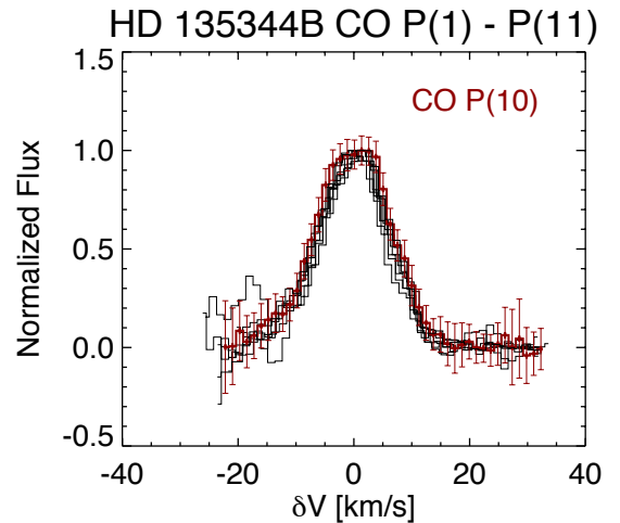
Fig. A.3. The CO P(1) to P(11) line profiles are available within the CRISRES spectrum. The lines have been continuum subtracted and normalized by the peak flux. The CO P(10) line is in red.
