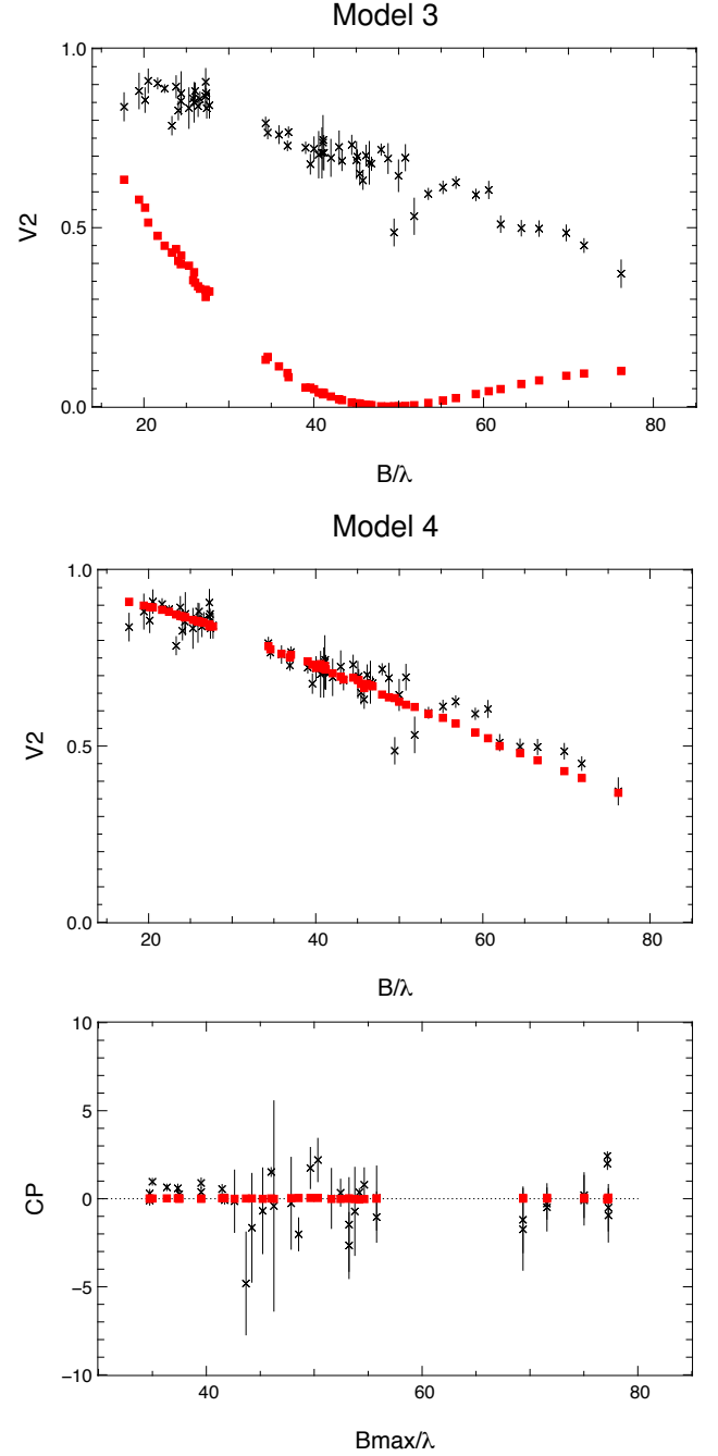
Fig. 5. Upper panel: squared visibilities (in red) of Model 3 overplotted on the observed 1.6 \mu\text{m} VLTI/PIONIER visibilities (in black). An inner disk starting at 0.2 AU is not consistent with observations. VLTI/PIONIER data clearly shows that there is material at smaller radii (i.e., inside the silicate sublimation radius). Central panel: squared visibilities (in red) predicted by Model 4 ( R_{\text{in}} = 0.08 AU). Lower panel: closure phases (CP) predicted by Model 4 (red) and measured by VLTI/PIONIER (black).
