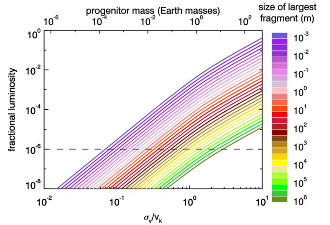
Figure 12. Initial fractional luminosity of impact debris versus \sigma_v and progenitor mass for an impact occurring at 50 au from a Sun-like star assuming 3 per cent of the progenitor mass is released as debris. The black dotted line represents the approximate detection limit. The relationship between \sigma_v and progenitor mass assumes a constant density equal to that of the Earth.
