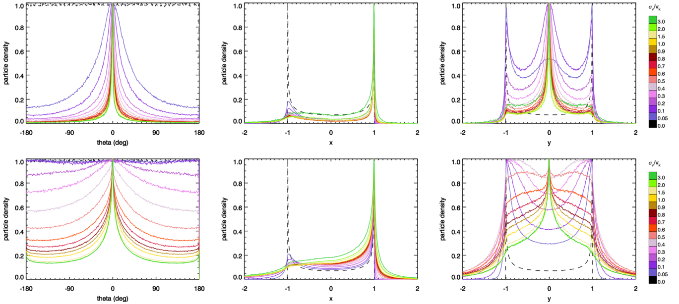
Figure 9. Top row: particle density along line cuts through the images in Fig. 8. At left the cut is around a ring of radius 1 in the x-y plane, at centre it is along z = 0 in the x-z plane, and at right it is along z = 0 in the y-z plane. Bottom row: particle density integrated over one dimension of the images in Fig. 8. At left the integral is over radius, and at centre and right right it is over z . Within each frame all curves are normalized to a peak value of 1.
