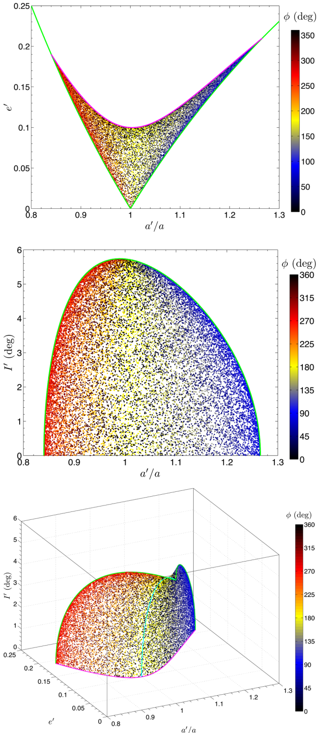
Figure 2. Distributions of orbital elements for a set of 20 000 particles given a kick of magnitude (\Delta v/v_k) = 0.1 in a random direction from an initially circular orbit. Top: a-e distribution, middle: a-i distribution, bottom: three parameter a-e-i distribution. The boundaries of the distribution are set by the new apocentre or pericentre being at the old semimajor axis distance (green lines) and the I' = 0 contour for a (\Delta v/v_k) = 0.1 kick (magenta line). On the a-e-i distribution, we also show the line of a'/a = 1 in cyan, which tracks close to one of the lines of principal curvature. Points are coloured by the value of \phi , with black corresponding to a kick directly away from the star, yellow directly towards the star, blue in the direction of orbital motion and red against the direction of orbital motion.
