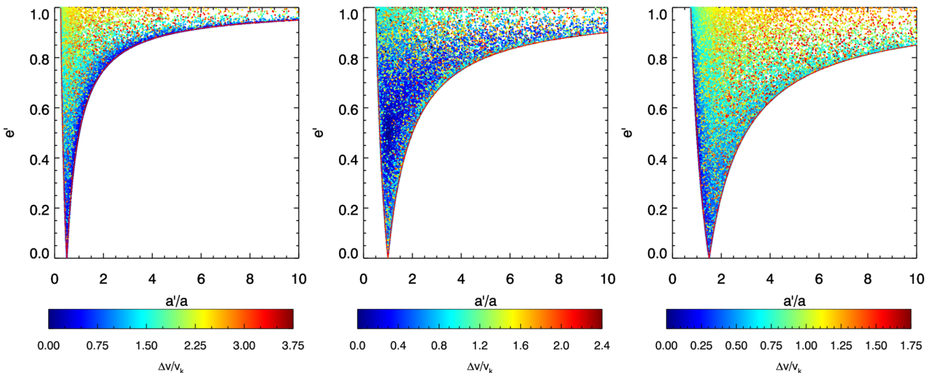
Figure 6. Semimajor axis–eccentricity distributions for particles on an initial orbit with an eccentricity of 0.5 kicked at three different points around their orbit, left : at pericentre, centre : at the semimajor axis distance, right : at apocentre. Points are coloured by the kick velocity received with the distribution of kick velocities uniform between zero and the maximum kick a particle can receive and remain bound in each case.
