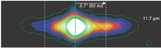
Figure 17. 11.7 \mu\text{m} image of Beta Pictoris (Fig. 1 d of Telesco et al. 2005). The image has been rotated 58^\circ counterclockwise with respect to the sky position-angle; north-east is to the left and south-west is to the right. The small circle at bottom right indicates the T-ReCS point-source FWHM. The vertical solid line is at the star (centre) and the vertical dotted lines are at 52 au from the star. The contours (in units of 0.01 \text{ mJy pixel}^{-1} ) are 10, 17, 26, 36, 45, 56, 68, 80, 93, 108, 123, 140. The brightest (inner) colours correspond to the highest numbered contour levels. Note that the star is heavily saturated in this image. There is a strong left–right asymmetry, peaked at a separation of 52 au from the star.
