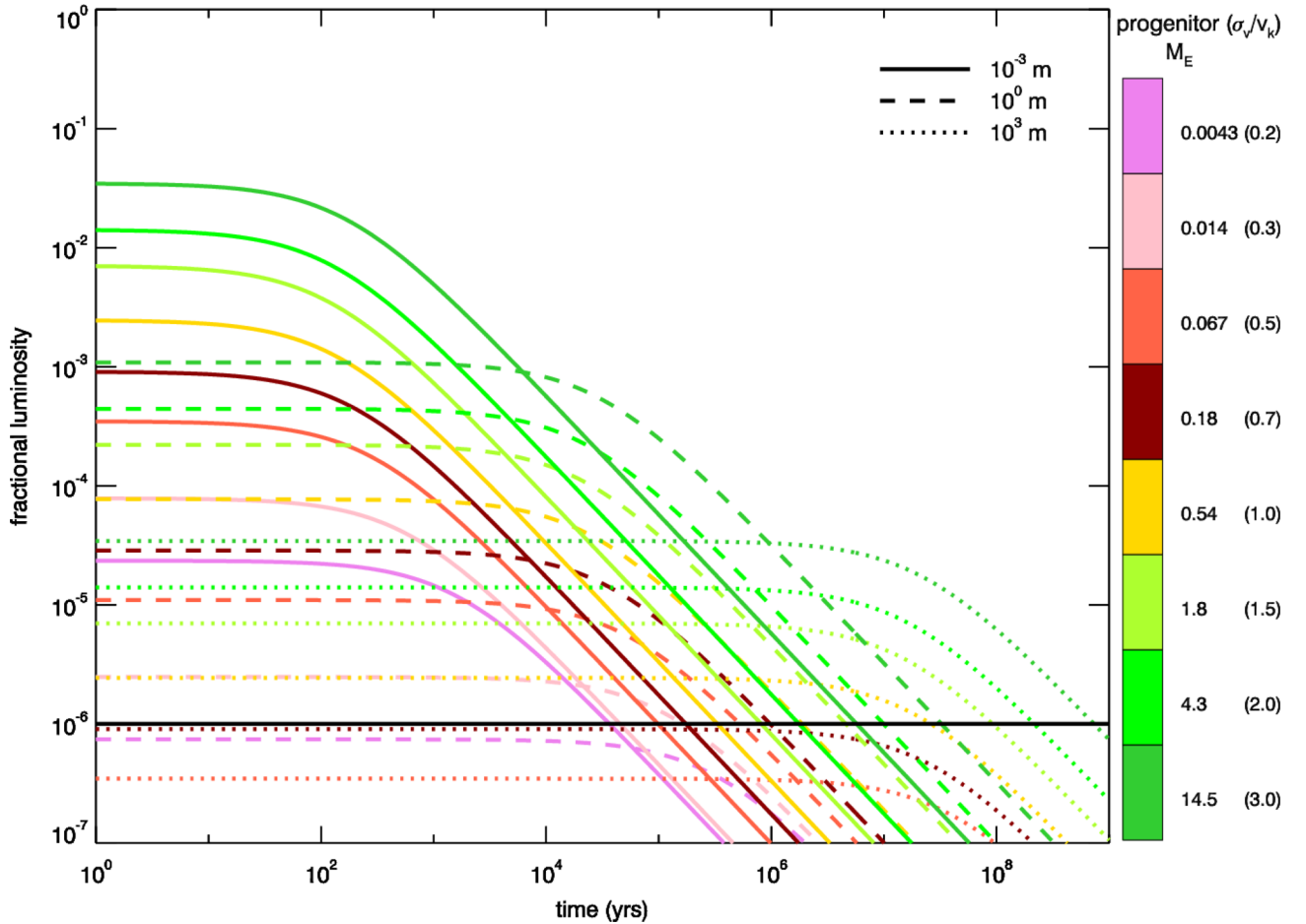
Figure 14. Temporal evolution of the fractional luminosity of a disc produced by a giant impact occurring at 50 au from a Sun-like star, releasing debris equal to 3 per cent of the progenitor mass, for a selection of velocity dispersions and largest fragment sizes. The black line indicates the approximate detection limit. The colour scale gives the mass of the progenitor (in M_{\oplus} ), with the corresponding value of \sigma_v/v_k in parentheses. The line style corresponds to the value of D_{\max} , as indicated.
