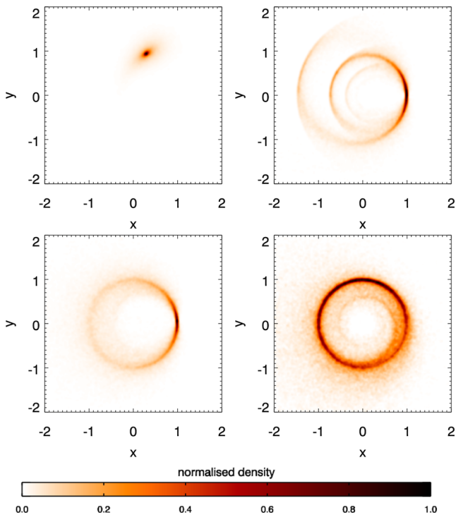
Figure 7. Phases of the dynamical evolution of a giant impact debris disc created at (1,0) at t = 0 from a progenitor on a circular orbit. Top left: appearance after 0.2 orbits. Top right: after 2 orbits. Bottom left: 200 orbits. Bottom right: 10 000 orbits. A velocity dispersion of \sigma_v/v_k = 0.3 is used. The effects of precession due to a Jupiter mass planet interior to the disc at 0.2 semimajor axis units are included. All images are normalized individually and have a Gaussian smoothing with FWHM 0.05 semimajor axis units applied.
