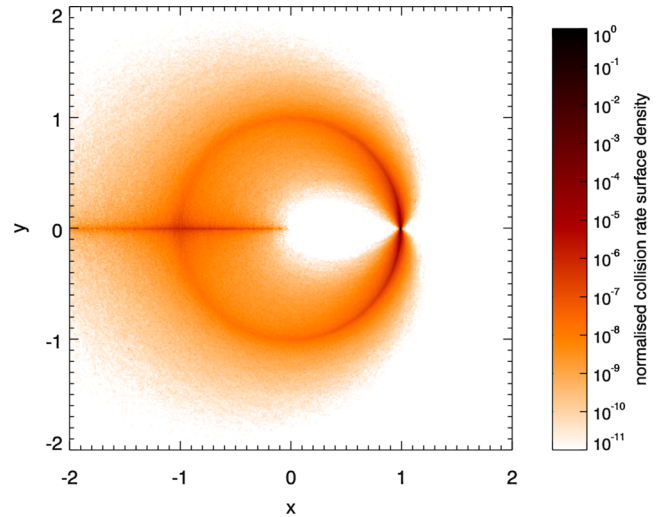
Figure 13. Image showing the normalized rate of collisions within a disc produced by an impact with \sigma_v/v_k = 0.3 . Produced using the same data as the bottom-left panel of Fig. 8.
