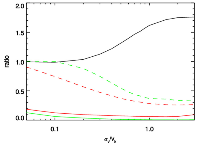
Figure 10. Ratios of different quantities from Figs 8 and 9 as a function of the kick velocity. Black: the ratio of the integral of the right-hand side of the face-on images over the left-hand side ( +x/-x ). Red: ratio of the ansae values in the x-z plane (centre column of Fig. 9), solid: the ratio of peaks from the line cut (upper frame), dashed: ratio of the sums within 0.15 of -0.95 and 0.95 in the lower frame. Green: collision-point versus anticollision line ratio with respect to \theta (left-hand column of Fig. 9), solid: trough-to-peak ratio in the upper frame, dashed: ratio of the sums within 20 degrees of the anticollision line and collision-point.
