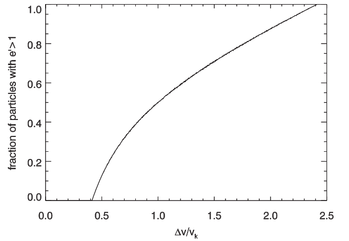
Figure 3. Fraction of particles that are put on to hyperbolic orbits ( e' > 1 ) as a function of the kick velocity for an isotropic distribution of kick directions. Above \Delta v/v_k = \sqrt{2} + 1 all particles have e' > 1 .
