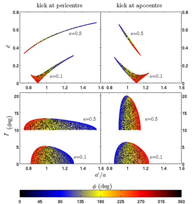
Figure 5. Semimajor axis–eccentricity distributions ( upper row ) and semi-major axis–inclination distributions ( lower row ) for particles kicked at pericentre ( left-hand column ) and at apocentre ( right-hand column ) and two different initial eccentricities ( e = 0.1 and e = 0.5 ). An isotropic kick of magnitude \Delta v/v_k = 0.1 is used. All distributions are coloured according to the value of \phi as described in Fig. 2. Each distribution is annotated with the initial eccentricity. The inclination distributions for initial eccentricity 0.5 have been offset by +10^\circ to separate the distributions.
