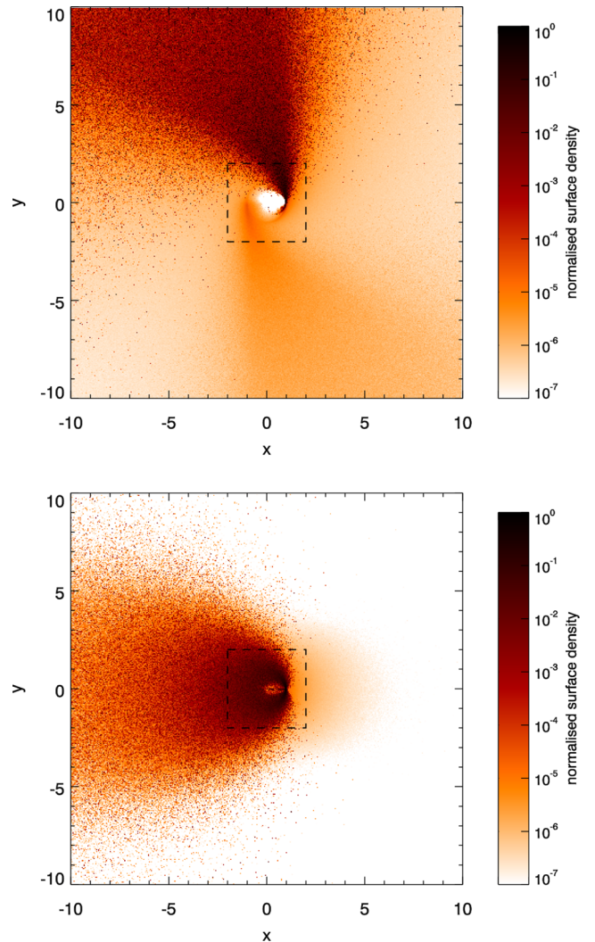
Figure 15. The distribution of small dust grains for a disc produced by an impact with \sigma_v/v_k = 0.3 . Top : unbound grains, bottom : bound grains. In both images, \beta is uniformly distributed between 0 and 0.99. Note the zoomed out scale in comparison with previous figures, the dashed box indicates the region covered by earlier images. The corresponding distribution of large grains can be found in Fig. 8(c).
