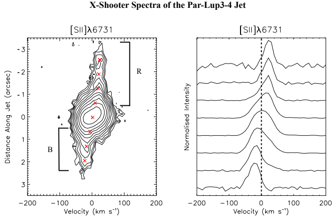
Fig. 7. Position velocity diagram of the Par-Lup 3-4 jet in [S II]λ6731 with the velocity centroid measured at various positions along the jet marked (red crosses). Right panel: line profiles corresponding to each red cross. Contours begin at 1.5 \times 10^{-18} erg/s/cm 2 and increase logarithmically to 68 \times 10^{-18} erg/s/cm 2 . Velocities are systemic. The extraction window for the spectra of the blue and red jets is also shown. The fluxes of the lines which are detected in these regions of the jets are given in Table A.2. The Par-Lup 3-4 jet is fairly symmetric and clearly the velocity of both lobes increases with distance from the source. Comerón & Fernández (2011) note the presence of a small red-shifted knot at \sim -2''.5 which is also seen here.
