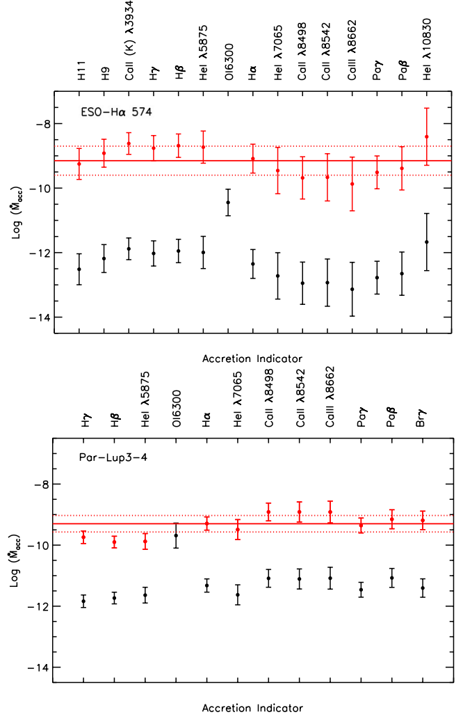
Fig. 8. Mass accretion rate calculated for various accretion indicators in ESO-H \alpha 574 ( top ) and Par-Lup 3-4 ( bottom ). The red points are the values of \dot{M}_{\text{acc}} after correction for obscuration by the disk. [OI] \lambda 6300 emission is an indirect indicator of accretion coming from extended regions and as such is blocked by disk. Therefore it is used as a test of the factor chosen to correct the other tracers for disk obscuration. The solid line gives the mean value of \log(\dot{M}_{\text{acc}}) and the dashed line is the \pm 1\sigma uncertainty.
