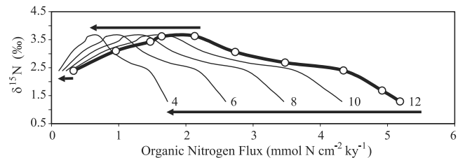
Figure 5. The SA effect. The curve of the basic experiment corresponds to a SA of 12 months. Other curves correspond to different situations with reduced SA (10, 8, 6, and 4 months).
