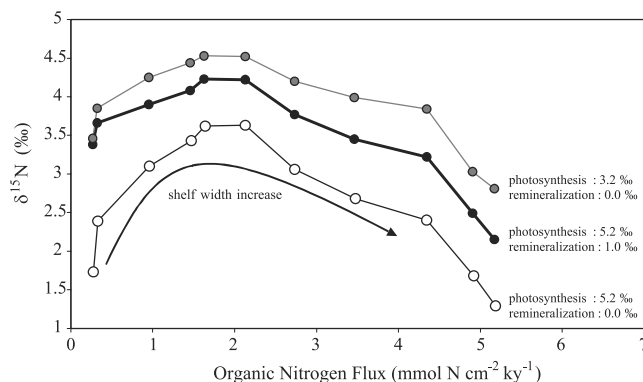
Figure 8. Model outputs of isotopic \delta^{15}\text{N} signal (‰) and ONF ( \text{mmol N cm}^{-2} \text{kyr}^{-1} ) as a function of the SW evolution for different configurations of fractionation factors (Nu, fractionation factor for nitrate uptake; Rm, fractionation factor for remineralization). Open circles: Nu = 5.2‰, Rm = 0‰ (curve of Figure 4); black circles: Nu = 5.2‰, Rm = 1‰; shaded circles: Nu = 3.2‰, Rm = 0‰.
