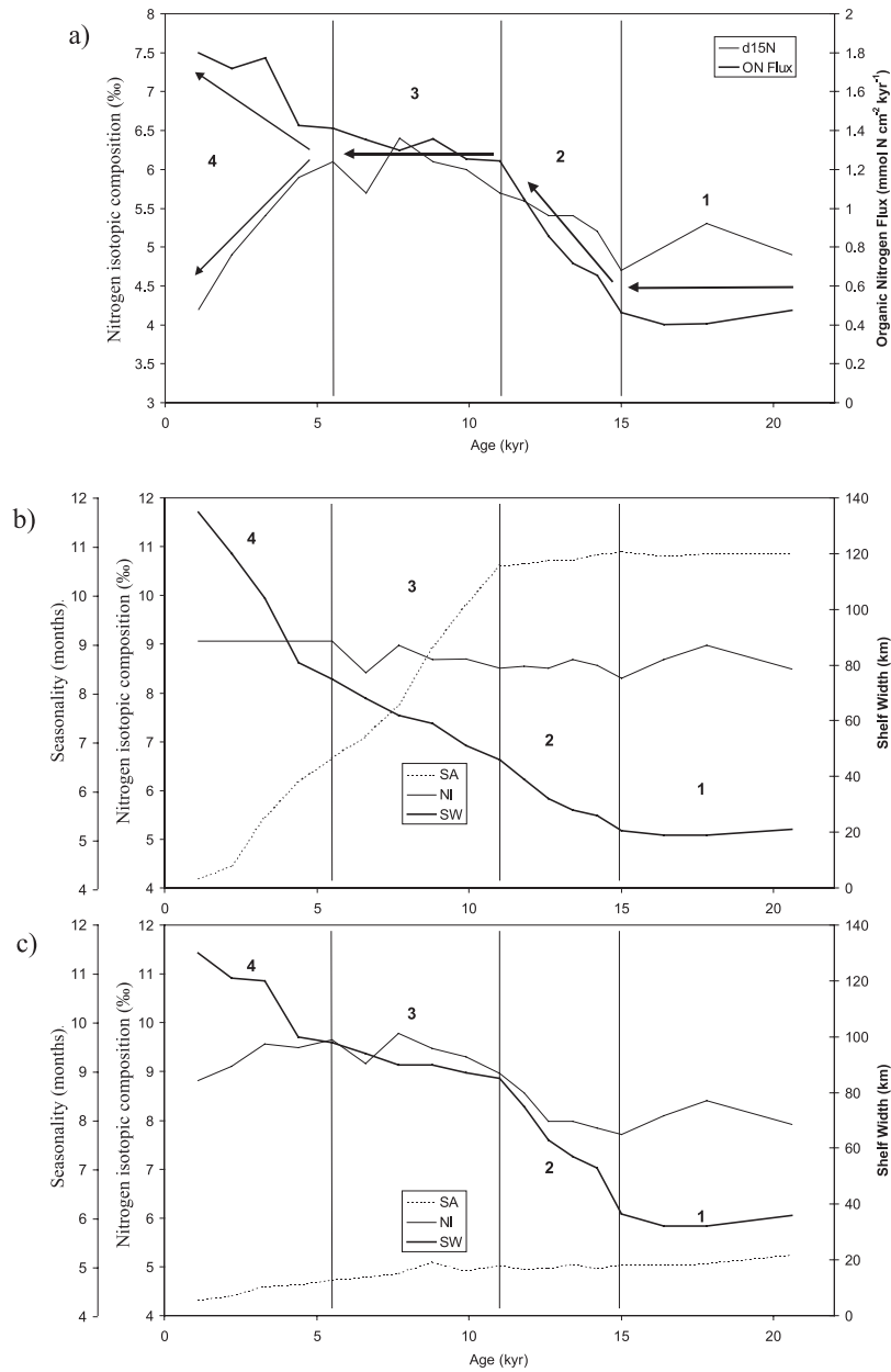
Figure 11. (a) Isotopic \delta^{15}\text{N} signal (‰) and ONF ( \text{mmol N cm}^{-2} \text{kyr}^{-1} ) from the LGM to present for core 11K ( 21^{\circ}28.87'\text{N} ; 17^{\circ}57.35'\text{W} ; 1200 m depth). Data from Martinez [1997]. Reconstructed SW, SA, and NI for two different scenarios: (b) minimized nutrient input variations, and (c) more or less constant SA.
