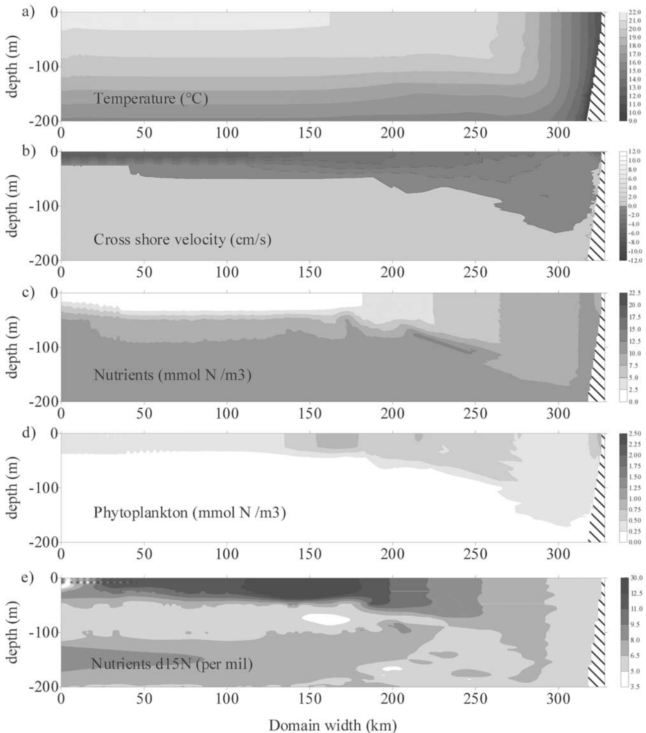
Figure 3. Cross section of (a) temperature (in ^{\circ}\text{C} ), (b) cross-shore velocity (in \text{cm s}^{-1} , positive values indicate currents directed onshore), (c) nutrients and (d) phytoplankton concentrations (in \text{mmol N m}^{-3} ), and (e) nitrate \delta^{15}\text{N} (in ‰) for a low sea level scenario (no continental shelf).
