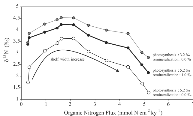
Figure 8. Model outputs of isotopic \delta^{15}\text{N} signal (‰) and ONF ( \text{mmol N cm}^{-2} \text{ kyr}^{-1} ) as a function of the SW evolution for different configurations of fractionation factors (Nu, fractionation factor for nitrate uptake; Rm, fractionation factor for remineralization). Open circles: Nu = 5.2‰, Rm = 0‰ (curve of Figure 4); black circles: Nu = 5.2‰, Rm = 1‰; shaded circles: Nu = 3.2‰, Rm = 0‰.
