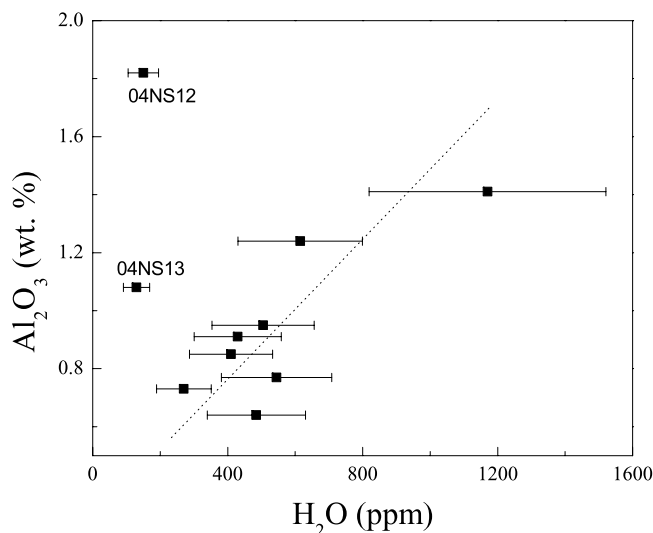
Figure 6. Correlation between \text{H}_2\text{O} (ppm wt) and \text{Al}_2\text{O}_3 (wt %) contents of the Nushan orthopyroxenes. Error bar indicates 30% of the \text{H}_2\text{O} content.
