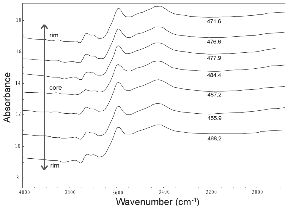
Figure 7. Hydrogen profile in an orthopyroxene grain from Nushan. The absorption at 3740\text{ cm}^{-1} is an artifact of the instrument and 3700\text{ cm}^{-1} is possibly from alteration products in submicroscopic cracks, while the other two bands are typical of OH in opx.
