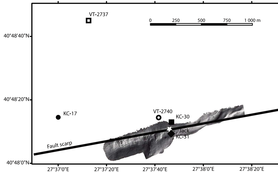
Figure 3. Detail map of structure and site location at the Tekirdağ Basin site.
