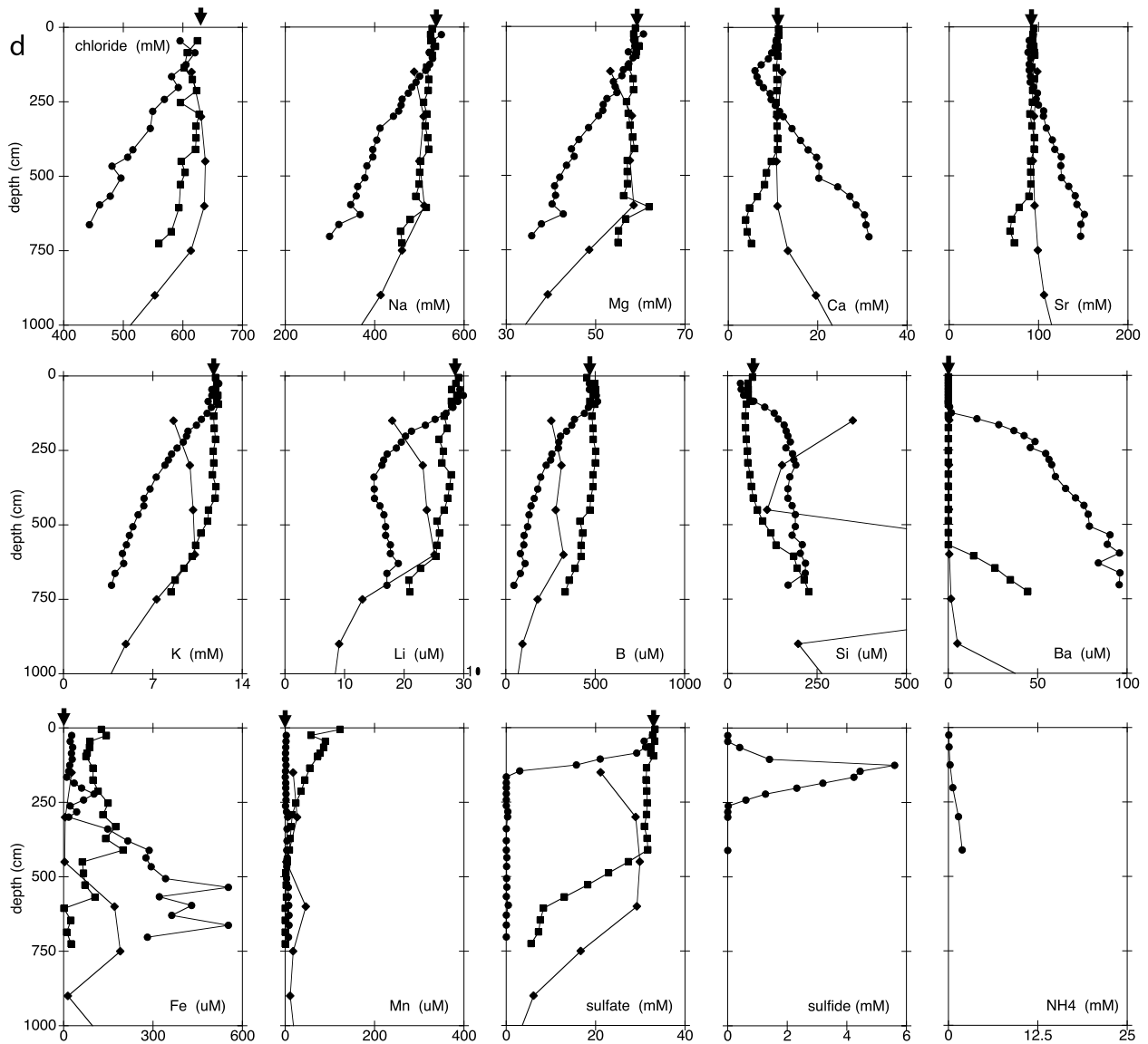
Ridge site cores • KC-20 ■ KC-26 ♦ VT-2741 Arrows indicate the composition of Sea of Marmara bottom water
