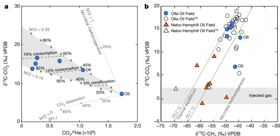
Fig. 2 | The \delta^{13}\text{C} of CO 2 in the Olla (CO 2 injected field) samples. a, The \delta^{13}\text{C} of CO 2 as a function of the CO 2 / ^3\text{He} ratio. The dashed lines show endmember methanogenesis and dissolution (pH 7) fractionation trajectories. The tick marks represent the total amount of CO 2 trapping within the system, relative to sample O5. The shaded region represents trapping by the combination of both microbial methanogenesis and dissolution. The upper and lower methanogenesis:dissolution ratios (M:D) are 0.33 and 0.19, respectively, showing that dissolution accounts for approximately three times more CO 2
