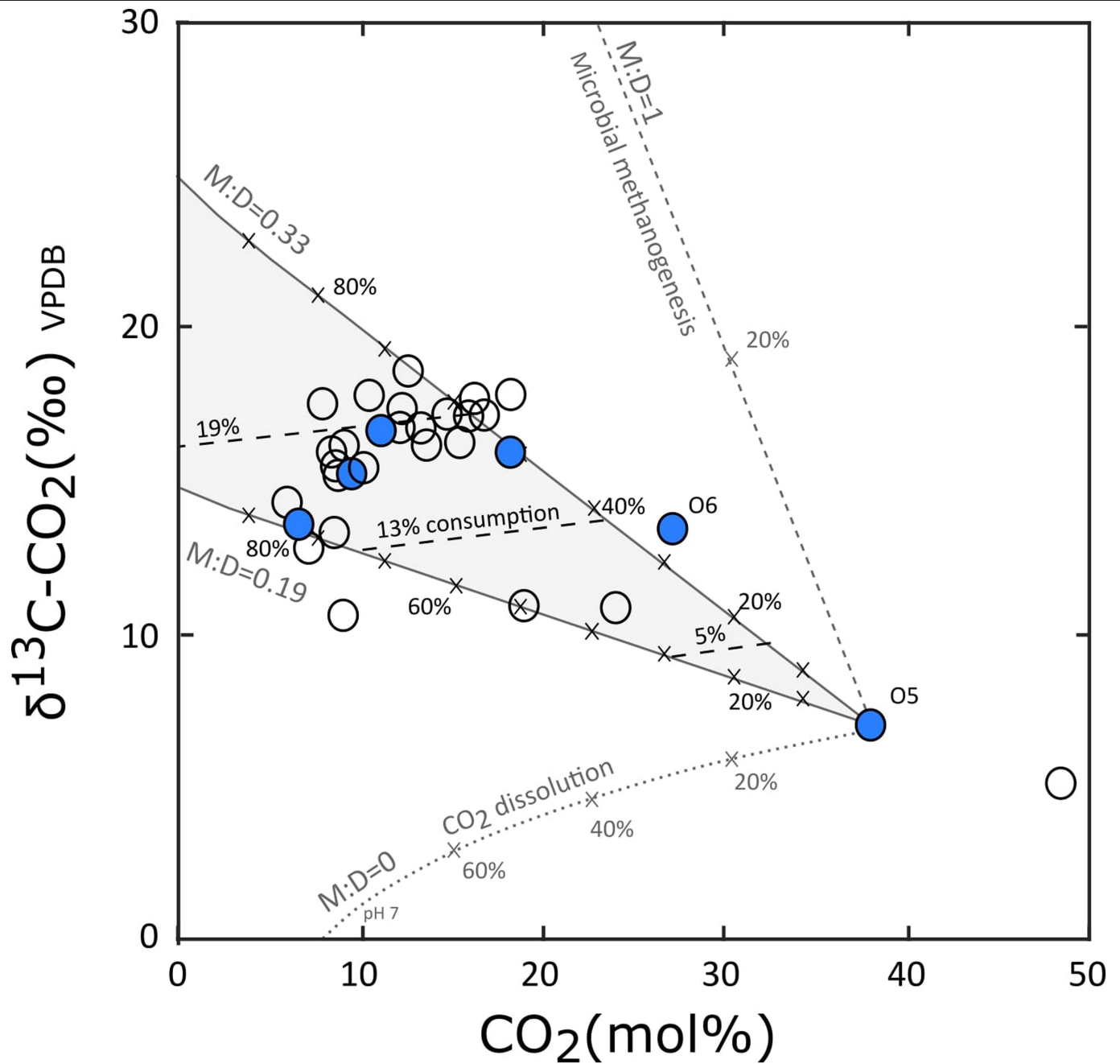
Extended Data Fig. 6 | Carbon isotopic composition of the Olla samples as a function of \text{CO}_2 concentration for data from this study (dark blue circles) and those collected without {}^3\text{He} analysis 10 (unfilled circles). One standard deviation error bars are within symbol size. Dashed lines show endmember methanogenesis and dissolution fractionation (at pH 7) trajectories. Tick marks represent the total amount of \text{CO}_2 trapping within the system, relative to sample O5. The shaded region represents trapping by the combination of both microbial methanogenesis and dissolution. The same combination of
