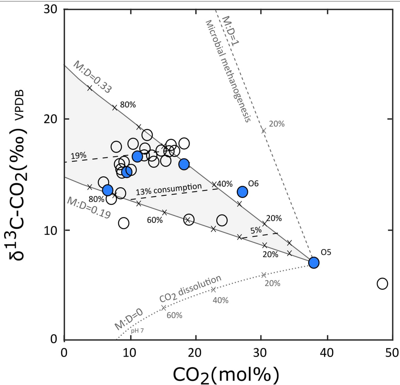
Extended Data Fig. 6 | Carbon isotopic composition of the Olla samples as a function of CO 2 concentration for data from this study (dark blue circles) and those collected without 3 He analysis 10 (unfilled circles). One standard deviation error bars are within symbol size. Dashed lines show endmember methanogenesis and dissolution fractionation (at pH 7) trajectories. Tick marks represent the total amount of CO 2 trapping within the system, relative to sample O5. The shaded region represents trapping by the combination of both microbial methanogenesis and dissolution. The same combination of
