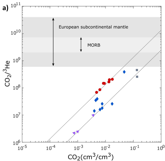
Extended Data Fig. 7 | Carbon composition of the Pannonian Basin samples. a , Szegholm South 20,99 (red circles), Szegholm North 20,99 (purple triangles), Ebes 20,99 (blue diamonds) and Hajduszoboszlo 20,99 (grey squares) gas field samples as a function of their CO 2 concentrations and CO 2 /³He. Dashed lines represent the projection of CO 2 trapping in the fields. b , The Szegholm South field had multiple CO 2 isotope data and this field has been used to investigate the processes controlling this pattern using the carbon isotopic composition as a function of CO 2 /³He. Dashed lines show endmember
