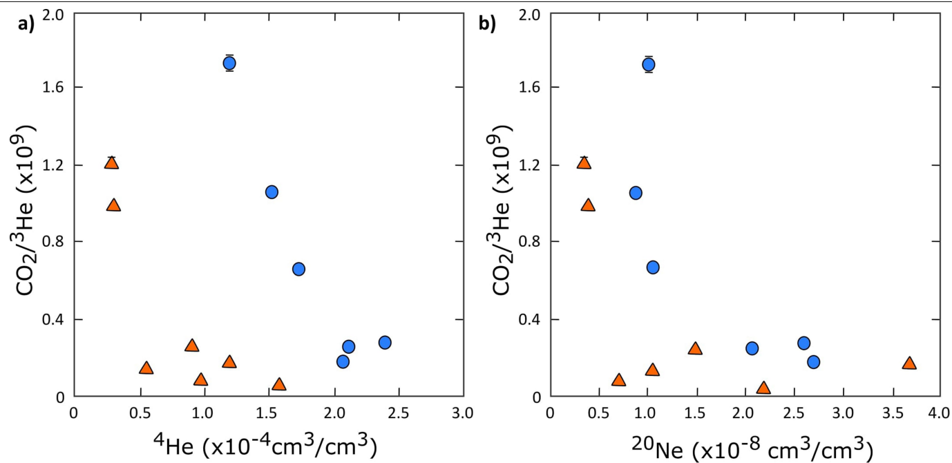
Extended Data Fig. 2 | \text{CO}_2/{}^3\text{He} variation vs. a, b, {}^4\text{He} (a) and {}^{20}\text{Ne} (b) abundances in the Olla (blue circles) and Nebo-Hemphill (orange triangles) oil fields. 1\sigma level of uncertainty is shown on the measured samples. A negative correlation between {}^4\text{He} , which accumulates in formation waters as a function
