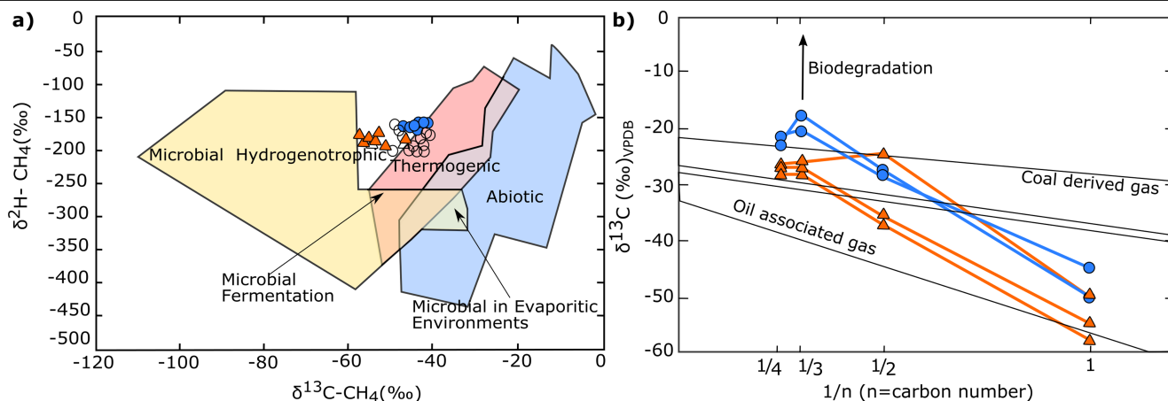
Extended Data Fig. 3 | Hydrocarbon isotopic composition in the Olla (blue circles) and Nebo-Hemphill (orange triangles) oil fields.
