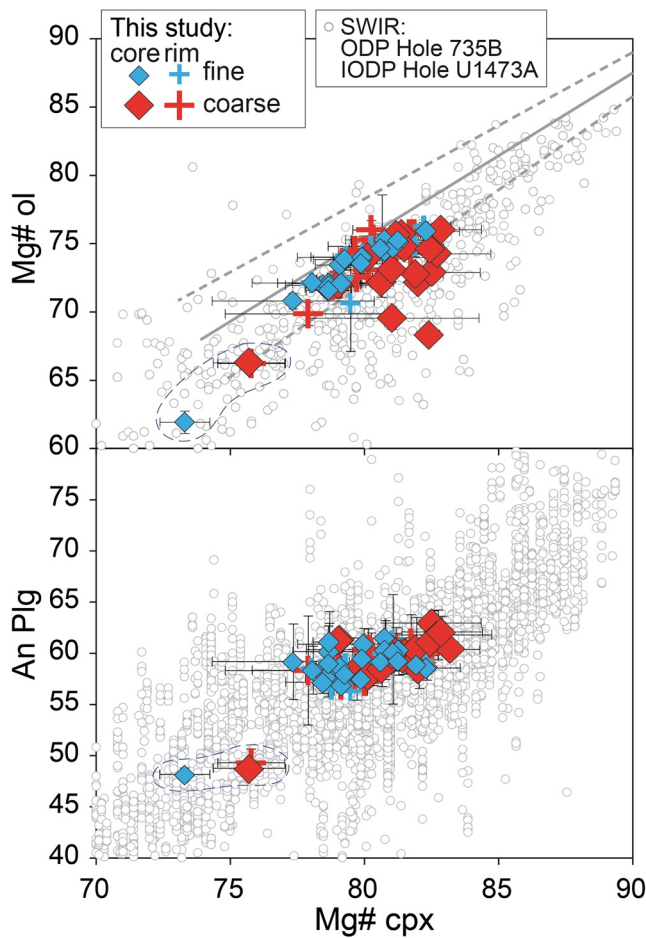
Figure 5. Coarse- (red) and fine-grained (blue) clinopyroxene Mg# ( Mg\# = 100 \times \text{cationic } (Mg/(Mg + Fe)) ) versus olivine Mg# and An content in plagioclase (average mineral composition per sample) from the studied olivine gabbros. Data are compared with theoretical Fe–Mg equilibrium between olivine and clinopyroxene, assuming mineral–melt Fe–Mg partition coefficients of 0.30 for olivine and 0.23 for clinopyroxene (Roeder & Emslie, 1970). The dashed lines represent the calculated olivine–clinopyroxene equilibrium line assuming an uncertainty of \pm 0.02 on the mineral–melt partition coefficients. Compositions of clinopyroxene–olivine and clinopyroxene–plagioclase in olivine gabbros from the nearby recovered ODP Hole 735B (Boulanger et al., 2020; Dick et al., 2002) and recent data from IODP Hole U1473A (Boulanger, 2020; Sanfilippo et al., 2020; Zhang et al., 2020) are reported for comparison. The dashed circles highlight the most evolved mineral compositions in sample 360-U1473A-83R-4W, 118–124 cm.
