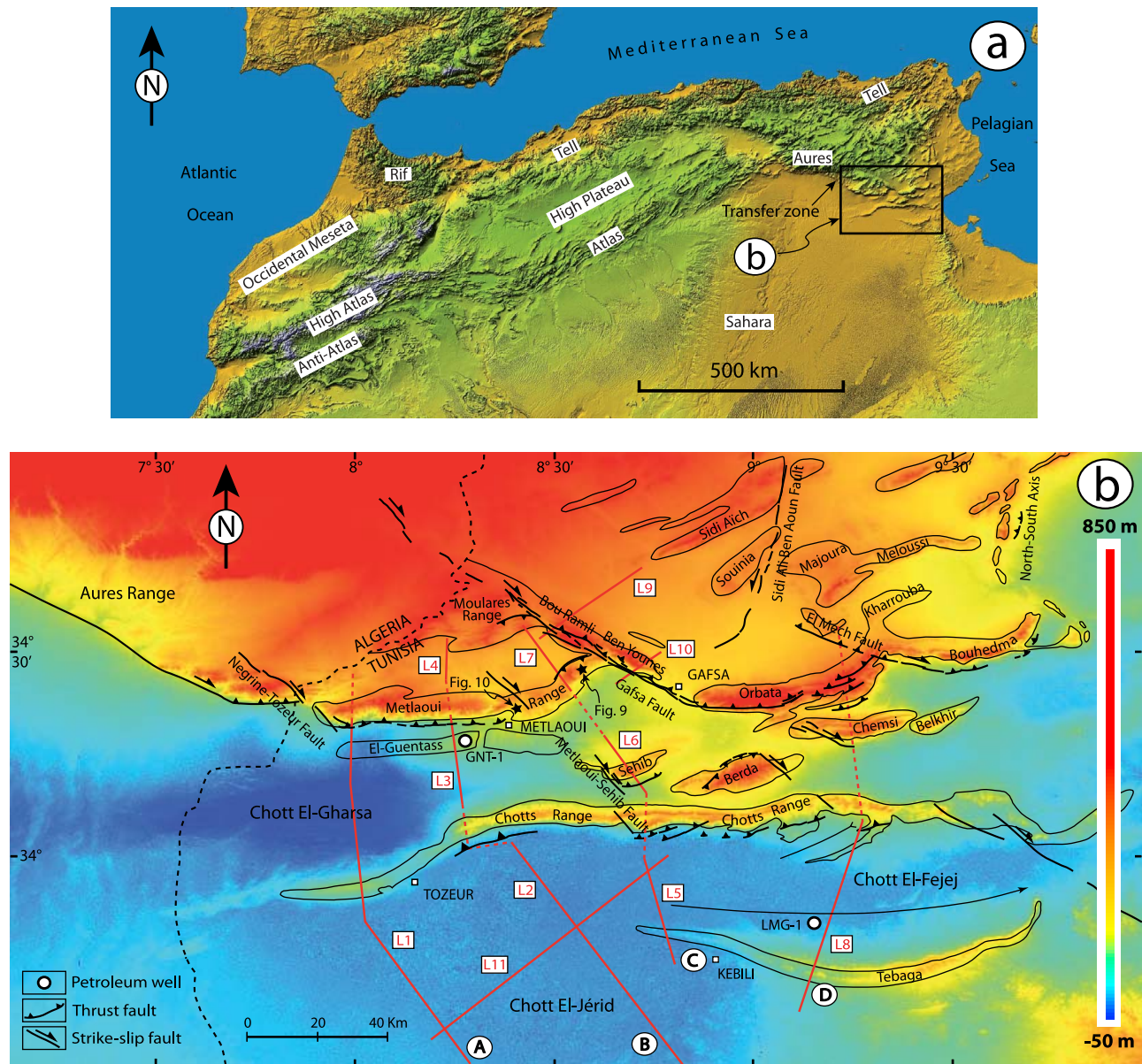
Figure 1. (a) Digital elevation model (DEM) of the Atlas with location of the study area. (b) Tectonic setting of central and southern Tunisia with location of the balanced cross sections (A–D) and the data set used in this study (DEM from the NASA Shuttle Radar Topography Mission GTOPO30). Continuous red lines represent reflection seismic sections (L1–L11) used for this study. Petroleum wells are also shown.
