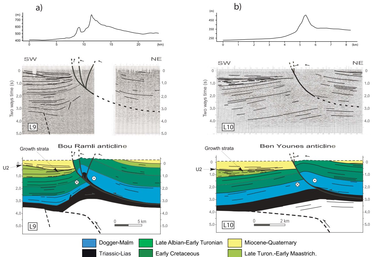
Figure 6. Seismic sections and corresponding geological cross sections crossing the Gafsa fault through the (a) Bou Ramli (L9) and (b) Ben Younes (L10) anticlines (see location in Figure 1). Note the topographic step related to the fault offset.
