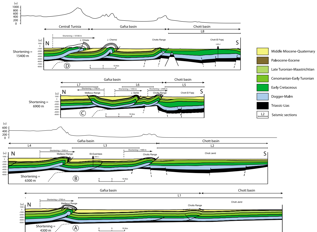
Figure 3. Balanced cross sections across the southern Tunisian Atlas. Detailed topographic profiles are shown for cross sections B and D. Balanced cross sections and data set are located in Figure 1b. Seismic sections used for the construction (L1–L8) are represented with continuous lines. Horizontal shortenings are calculated using Midland Valley 2DMove software.
