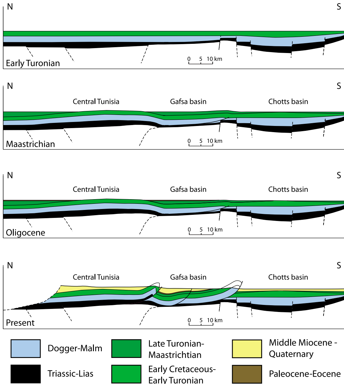
Figure 10. Schematic kinematic evolution of the central and southern Tunisian Atlas illustrating the mean stages since the Late Cretaceous to the Present.
