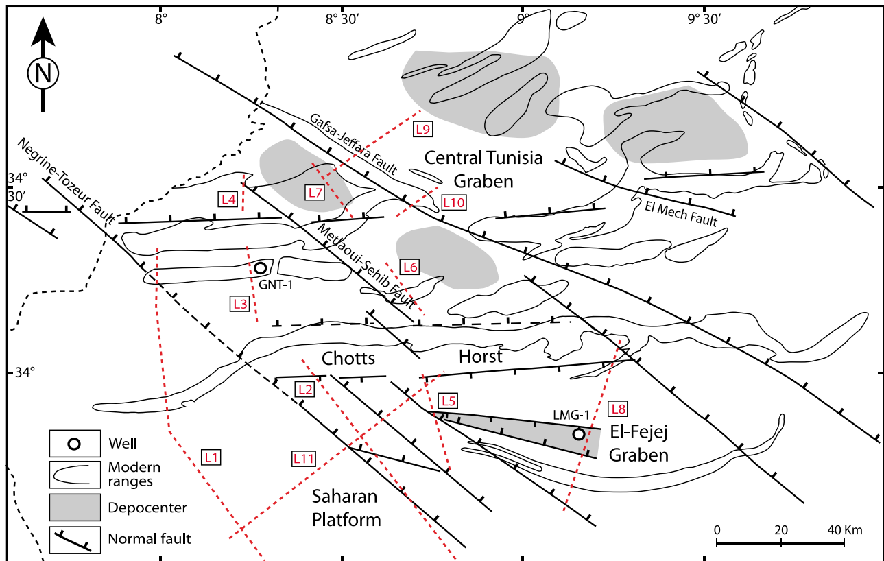
Figure 8. Late Triassic–Early Jurassic structural pattern of the central and southern Tunisian Atlas. Faults and depocenters are superimposed on the map of modern ranges derived from Figure 1b.
