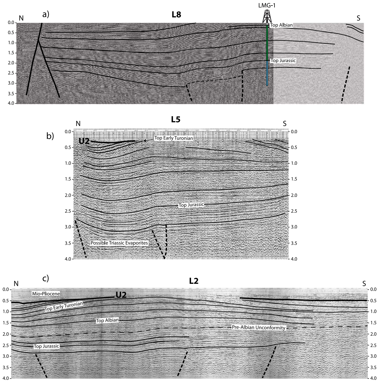
Figure 4. (a) Cross section L8. Interpreted seismic section crossing the Chott El-Fejej used for the construction of cross section D (Figure 3). (b) Cross section L5. Interpreted seismic section crossing the Chott El-Fejej used for the construction of cross section C (Figure 3). (c) Cross section L2. Interpreted seismic section crossing the Chott El-Jerid used for the construction of cross section B (Figure 3). U2 corresponds to the Oligocene-Early Miocene unconformity. L8, L5, and L2 are located in Figure 1b.
