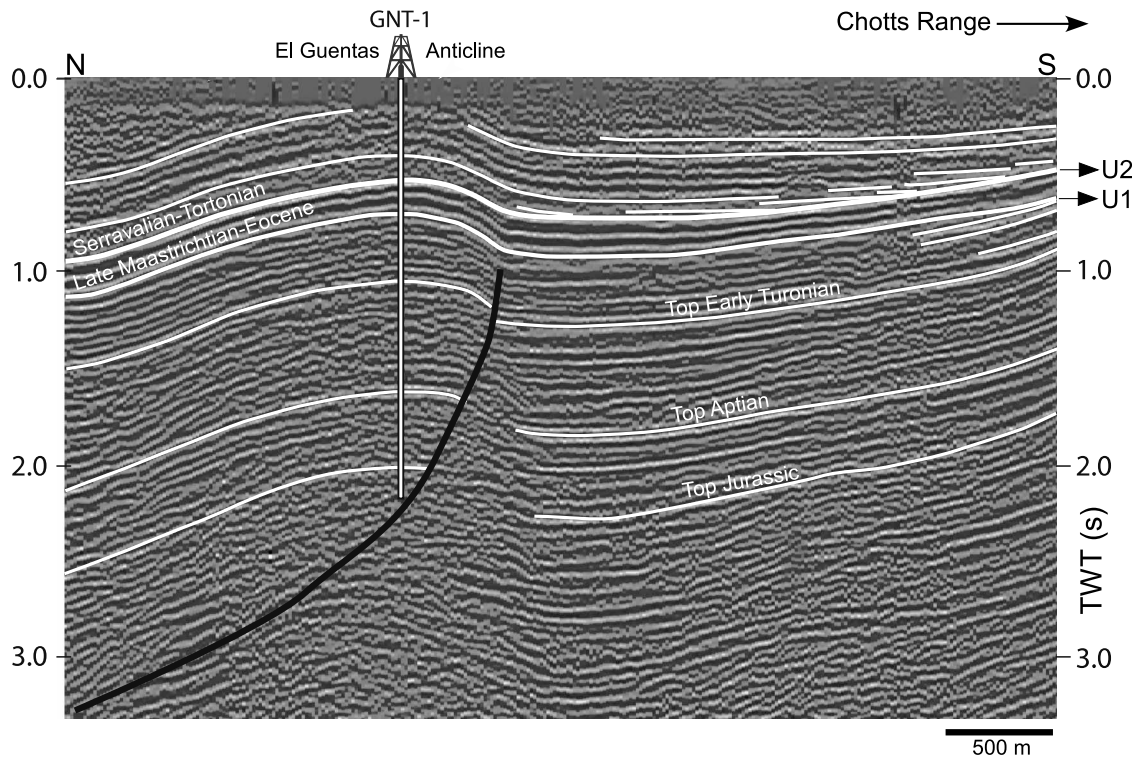
Figure 5. Interpreted seismic section (L3) crossing the El Guentass anticline (see location in Figure 1b). Two unconformities are outlined, U1 at the base of the early Maastrichtian and U2 sealed by the Serravalian-Tortonian Beglia formation.
