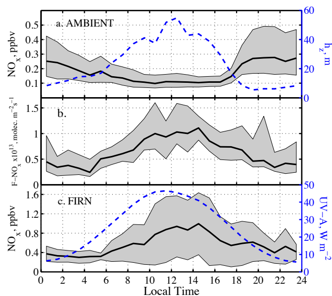
Fig. 9. The diurnal cycle of \text{NO}_x atmospheric mixing ratios and flux during 22 December 2009–28 January 2010: (a) \text{NO}_x mixing ratios at 1 m with boundary layer height h_z estimated after Pollard et al. (1973), (b) observed \text{NO}_x flux ( F\text{-NO}_x ) between 0.01 and 1 m and (c) \text{NO}_x mixing ratios in firn air from occasional sampling (Table 2) and UV-A irradiance at 1 m. Lines are median values and shaded areas the 25–75 percentile range of 1-hourly bins; except \text{NO}_x in firn air is average \pm 1\sigma .
