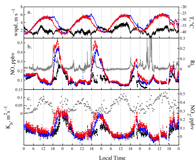
Fig. 4. Diurnal variability during 1–4 January 2010: (a) wind speed (wspd) at 3 m (black line), temperatures ( T ) of air at 1 m (blue line) and the snow surface (red line), (b) NO mixing ratios at three heights and bulk Richardson number ( Ri_b ) (grey line) and (c) NO 2 mixing ratios at three heights and turbulent diffusion coefficient of heat ( K_h ) at 1 m (grey symbols). Mixing ratios at 0.01, 1.0 and 4.0 m are shown as red, blue and black symbols, respectively.
