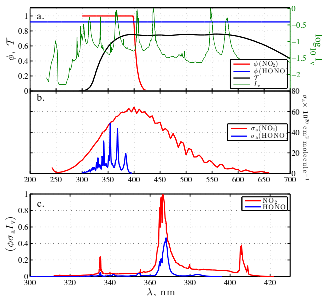
Fig. 2. The potential interference of HONO in the detection of \text{NO}_2 was estimated using (a) the scaled intensity I_v of the photolytic converter (200-W high pressure arc mercury lamp, USHIO-200DP), the respective quantum yield \phi , total transmittance \mathcal{T} of the optical filters, including a Pyrex window (Oriel, Part No. 60127) and a KBr filter (KG3, Oriel Part No. 51960), (b) the respective absorption cross sections \sigma_a (Sander et al., 2006) and (c) scaled (\phi\sigma_a I_v) in order to calculate respective photolysis rate constants j = \int \phi\sigma_a I_v d\lambda and their ratio. \lambda is wavelength and note different scale of x-axis in (c).
