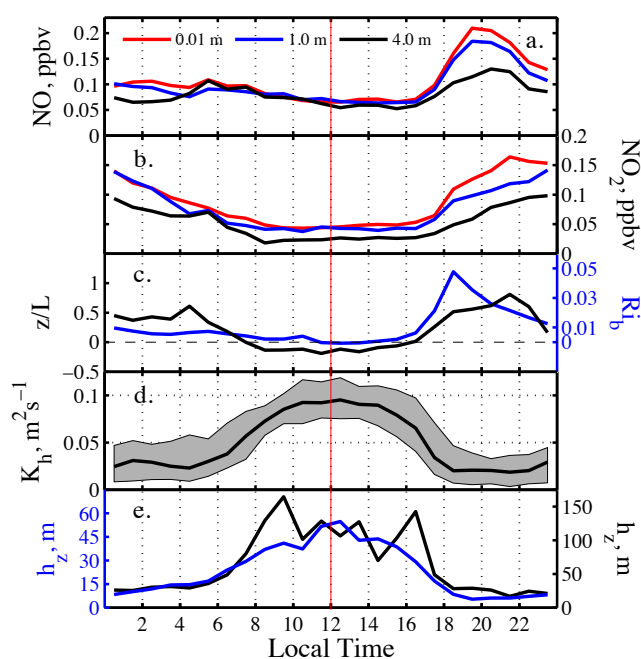
Fig. 5. The asymmetry in diurnal cycles of mixing ratios and physical boundary layer variables with respect to local noon (vertical red line): (a) NO mixing ratios, (b) NO 2 mixing ratios, (c) atmospheric stability as expressed by the Monin-Obukhov length ratio z/L , with sonic anemometer height z , and bulk Richardson number Ri_b , (d) turbulent diffusion coefficient of heat K_h at 1 m and (e) boundary layer height h_z estimated after Pollard et al. (1973) (blue line) and Zilitinkevitch et al. (2002) (black line); note different y-axis scales. Lines represent median values and shaded areas the range between the 0.25 and 0.75 percentiles of 1-hourly bins during 22 December 2009–28 January 2010.
