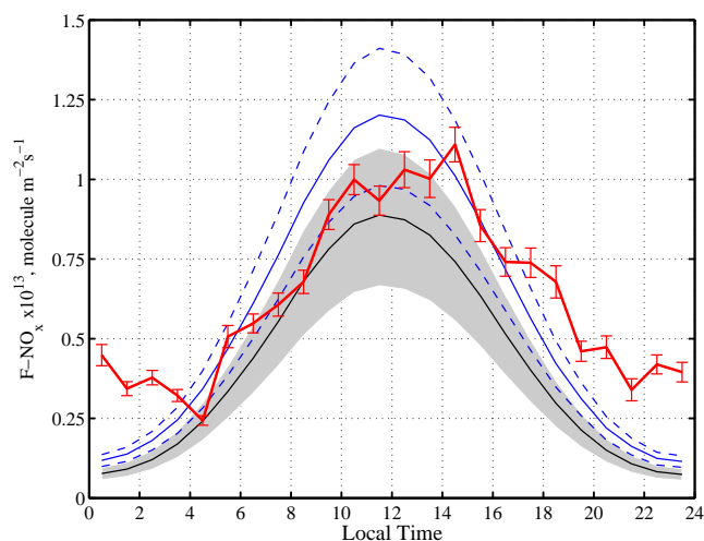
Fig. 10. The median diurnal variation of \text{NO}_x flux ( F\text{-NO}_x ) at Dome C compared to model calculations: F\text{-NO}_x during 22 December 2009–28 January 2010 observed between 0.01 and 1 m (red line) and its uncertainty (error bars indicating the 1\text{-}\sigma standard error of the median calculated as 1.253 \sigma/\sqrt{N} , where \sigma is the random error of 10-min flux values and N is the number of samples per 1-h bin, e.g. Maindonald and Braun, 2003). Modeled F\text{-NO}_x during 22 December 2009–21 January 2010 from \text{NO}_3^- photolysis only (Reaction R10, black line) and including also contributions from \text{NO}_2^- photolysis (Reaction R12) assuming a maximum \text{NO}_2^- concentration in snow of 0.5 ppbw (blue line). The shaded area and dashed lines show the range of F\text{-NO}_x due to the spatial variability in \text{NO}_3^- snow profiles at Dome C reported in France et al. (2011).
