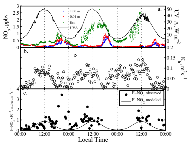
Fig. 8. Atmospheric mixing ratios of \text{NO}_x and snow emissions during 18–21 January 2010. Shown are (a) mixing ratios above the snow and in firn air along with UV-A irradiance, (b) the turbulent diffusion coefficient of heat K_h at 1 m and (c) observed \text{NO}_x flux compared to modelled potential \text{NO}_2 flux from nitrate photolysis (Reaction R10).
