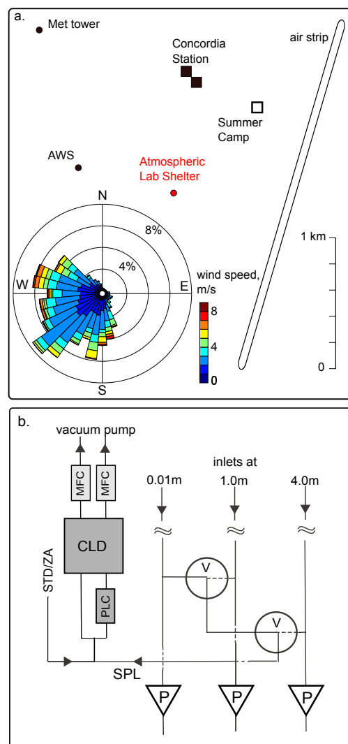
Fig. 1. (a) The wind rose for Dome C during December 2009 to January 2010 and location map of the atmospheric lab shelter, air strip, Concordia station, automatic weather station (AWS) and meteorology tower with sonic anemometer. (b) Schematic of the NO x sampling set up: sample air (SPL) is drawn continuously by vacuum pumps (P) from 3 inlet heights which are sampled by automatic switching of two 3-way valves (V). Sample flow into the chemiluminescence detector (CLD) through two channels, one with photolytic converter (PLC), is regulated by mass flow controllers (MFC). For calibration NO gas standard (STD) and for artefact tests zero air (ZA) are added upstream of the PLC. Triangles indicate flow direction (details in text).
