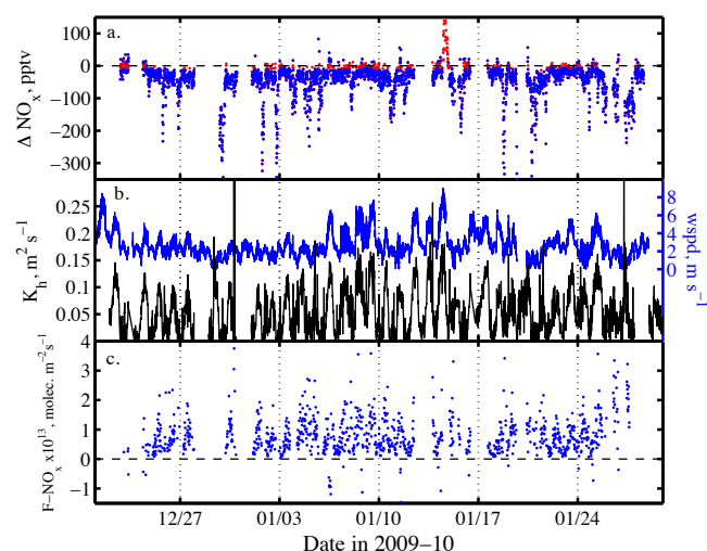
Fig. 7. 10-min averages of \text{NO}_x flux at Dome C in summer 2009–2010 between 1.0 and 0.01 m: (a) difference in \text{NO}_x mixing ratios ( \Delta\text{NO}_x ) between 1.0 and 0.01 m (blue symbols); values within \pm 1\sigma standard error were excluded from the flux calculation (red symbols), (b) turbulent diffusion coefficient of heat ( K_h ) at 1 m and wind speed (wspd) at 3 m, and (c) \text{NO}_x flux ( F\text{-NO}_x ).
