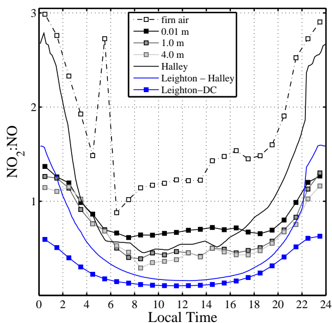
Fig. 11. The median diurnal cycle of the \text{NO}_2 : \text{NO} ratio during 22 December 2009 to 28 January 2010 shows significant deviations from Leighton steady-state at Dome C. Halley observations (black line) are shown for comparison (Bauguitte et al., 2012).
