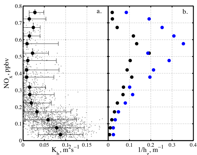
Fig. 6. (a) Atmospheric mixing ratios of \text{NO}_x as a function of the turbulent diffusion coefficient of heat K_h (both at 1 m). Plotted are 10-min means (grey symbols) and data binned into 50 pptv intervals (median values as black symbols and error bars indicating the 5–95 percentile range). (b) Binned \text{NO}_x mixing ratios as a function of boundary layer height h_z estimated after Pollard et al. (1973) (blue symbols) and Zilitinkevitch et al. (2002) (black symbols).
